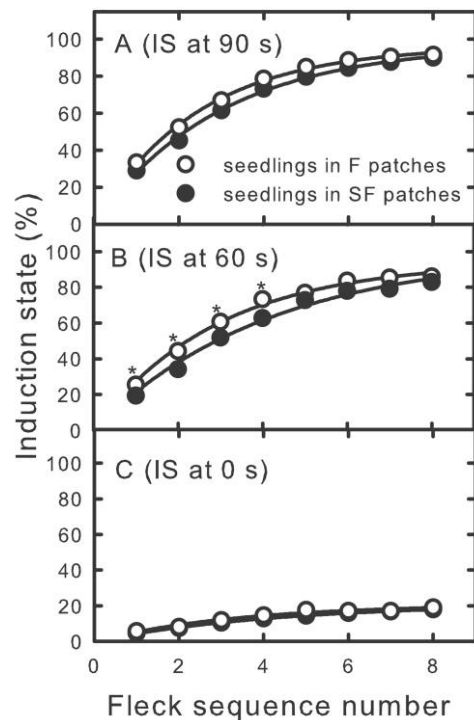
Fig. 4 Photosynthetic induction state at 90 s (A), 60 s (B), and 0 s (C) for each lightfleck in a series of eight replicate lightflecks experienced by Quercus rubra seedlings growing in a southern Appalachian forest. Each lightfleck response curve in the sequence consisted of (1) 60 s at low photon flux density (PFD; 10 \mu\text{mol m}^{-2} \text{s}^{-1} ), (2) 90 s at high PFD (500 \mu\text{mol m}^{-2} \text{s}^{-1} ), and (3) 60 s at low PFD (10 \mu\text{mol m}^{-2} \text{s}^{-1} ). Open circles represent seedlings growing in forest patches without understory evergreen shrubs (F patches). Filled circles represent seedlings growing in forest patches with understory evergreen shrubs (SF patches). An asterisk represents a significant difference (paired t -test) at the \alpha = 0.05 level between the two forest patch types.
