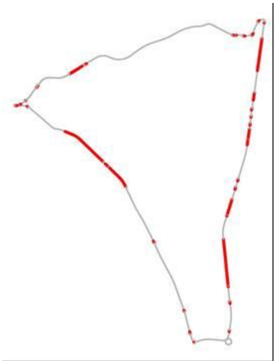
Figure 11 - Grip data plotted using GIS showing areas where wet grip is less than 0.4
