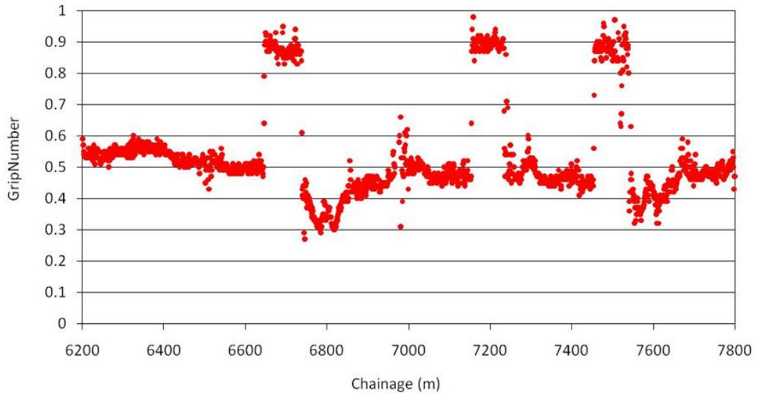
Figure 1 - Example GripTester data showing how short sections of high friction surfacing can significantly increase wet grip compared to hot mix asphalt
