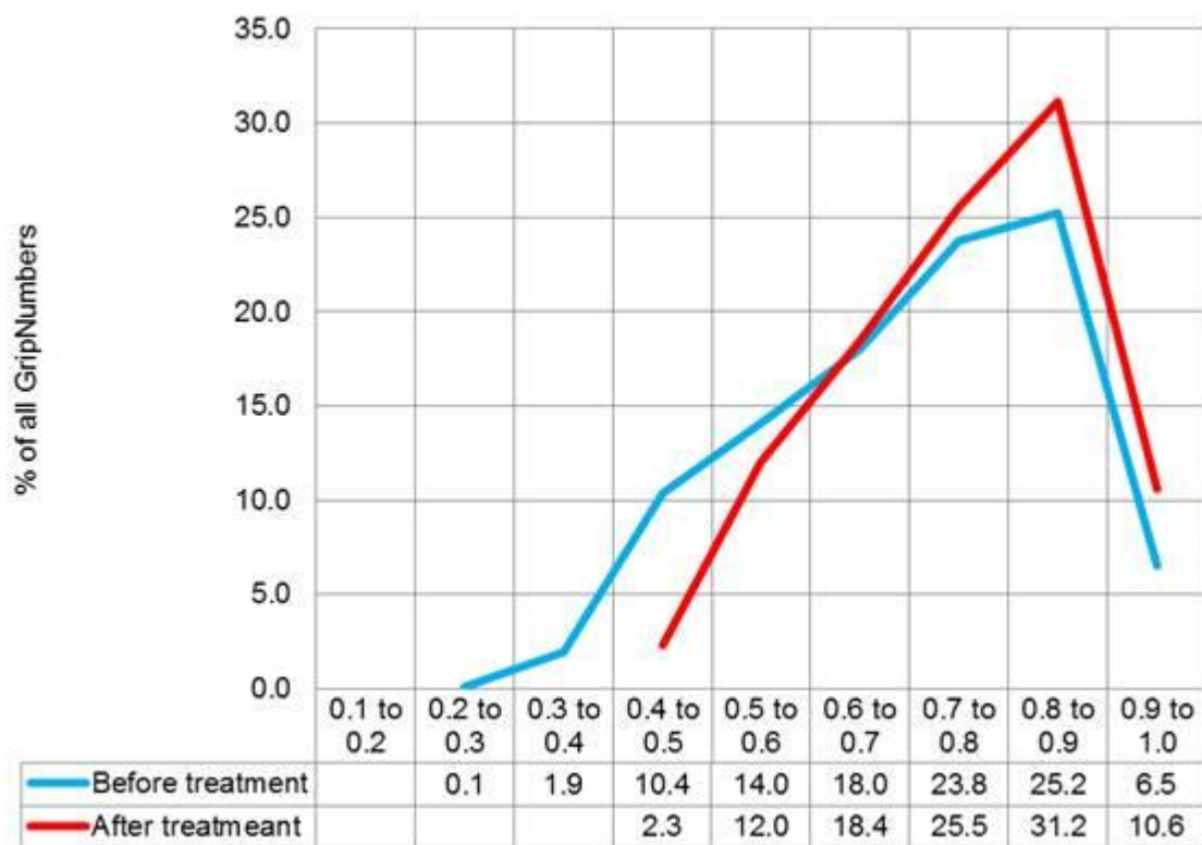
Figure 15 - Frequency distribution showing change in wet grip before and after treatment of corners
