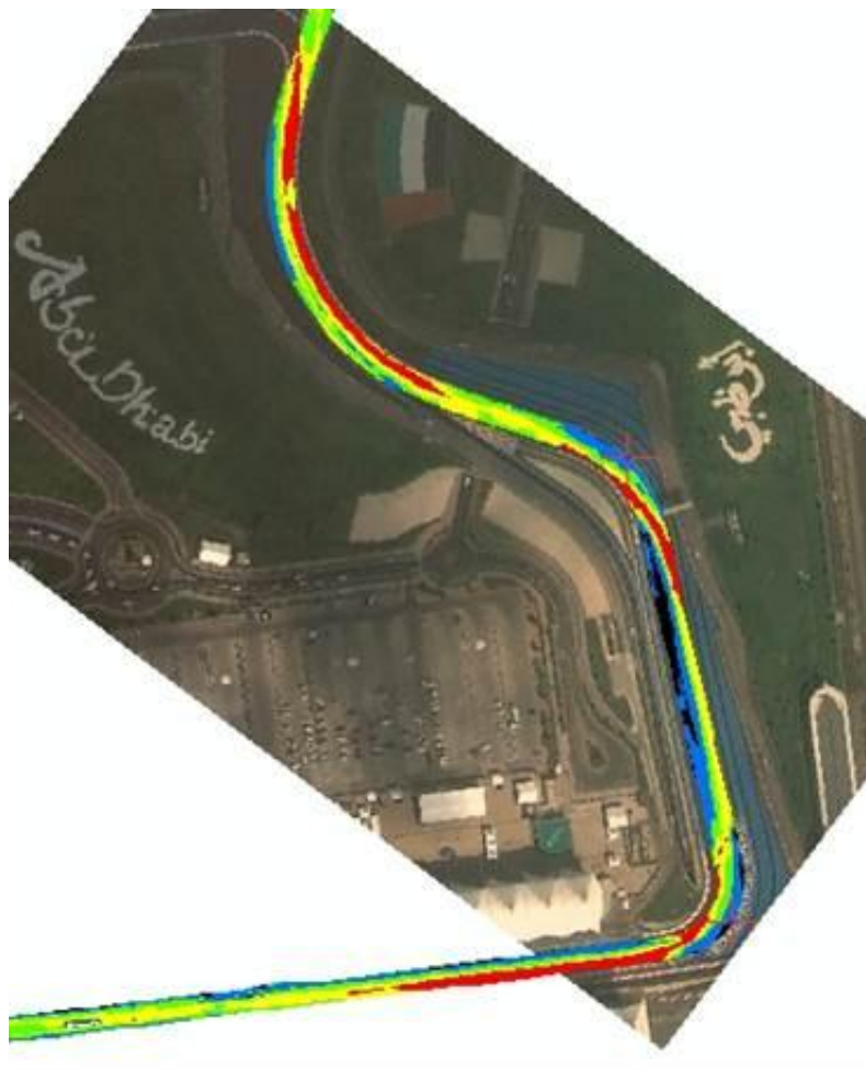
Figure 13 – GripMap showing variation in longitudinal and lateral wet grip at Yas Marina F1 circuit corners 1,2 and 3
