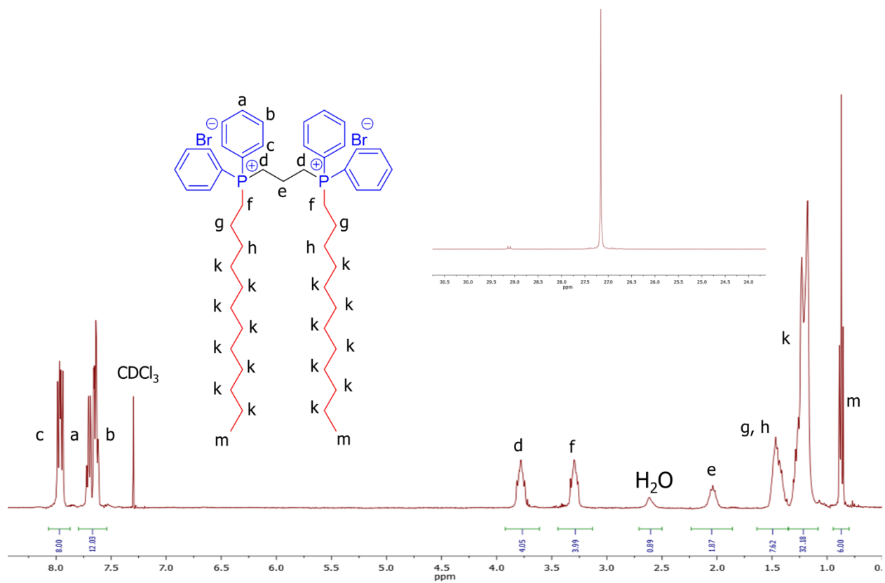
Figure S2. ^1\text{H} and ^{31}\text{P} NMR spectroscopy of 12-3-12P phosphonium gemini surfactant.
