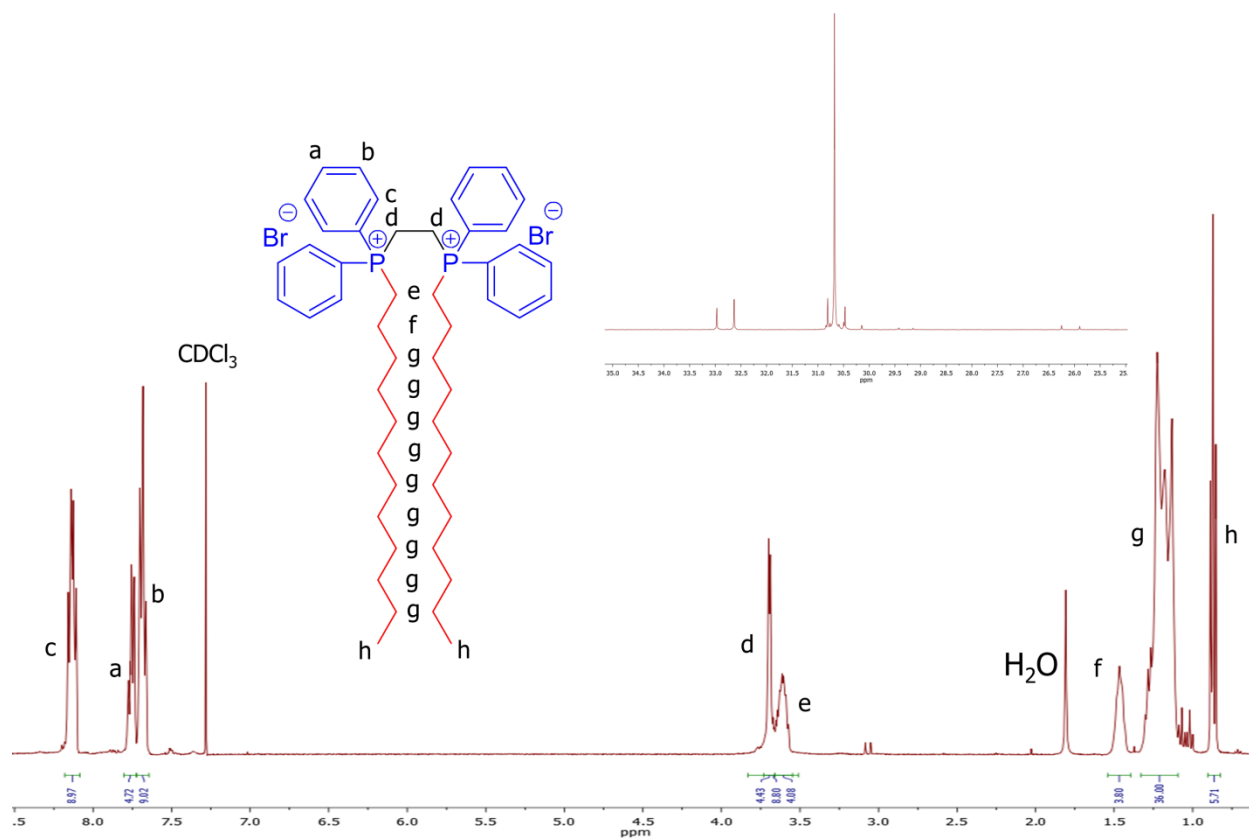
Figure S3. ^1\text{H} and ^{31}\text{P} NMR spectroscopy of 12-2-12P phosphonium gemini surfactant.
