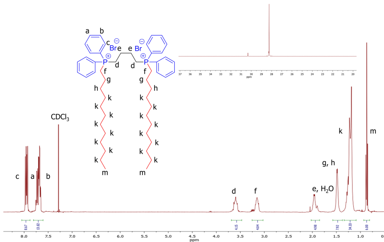
Figure S1. ^1\text{H} and ^{31}\text{P} NMR spectroscopy of 12-4-12P phosphonium gemini surfactant.
