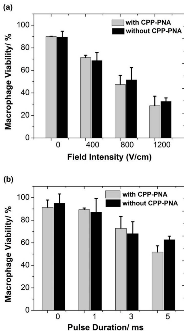
Fig. S1 Macrophage viability under various electroporation conditions. The presence of CPP-PNA (30 \mu M) did not affect the macrophage viability. Macrophages were not infected. (a) Macrophage viability under various field intensities when a single pulse with 5 ms duration was applied. (b) Macrophage viability under various pulse durations with a single pulse with 800V/cm field intensity applied.
