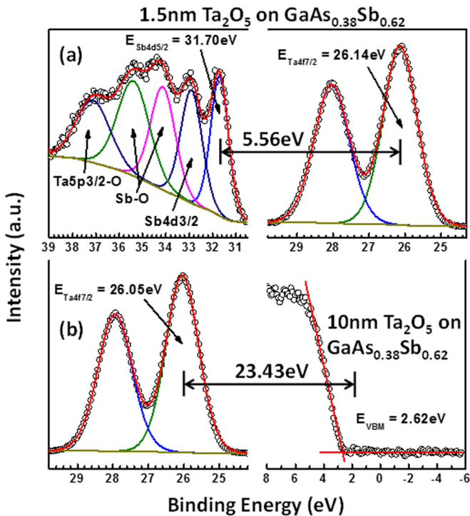
FIG. 8. XPS spectra of (a) the Sb 4d and Ta 4f core levels from 1.5 nm Ta 2 O 5 on bulk GaAs 0.38 Sb 0.62 ; (b) the Ta 4f core level and valence band from 10 nm Ta 2 O 5 on bulk GaAs 0.38 Sb 0.62 . Core level spectra were fitted using a Lorentzian convolution with a Shirley-type background. The valence band maximum is determined by linearly fitting the leading edge of the valence band spectrum to the base line.
