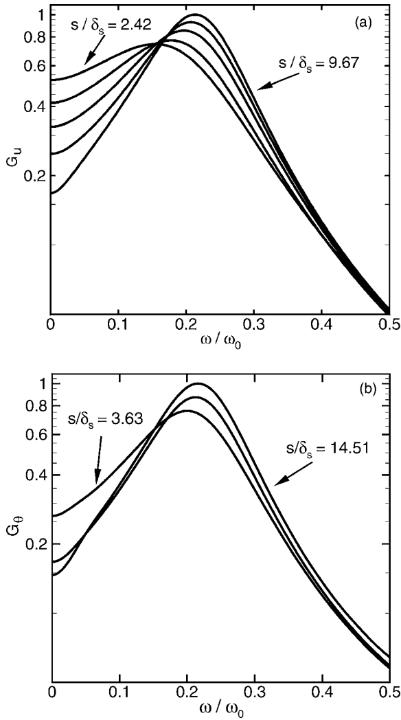
FIG. 9. Panel (a), the noise spectra G_u of stochastic fluctuations in cantilever tip deflection for separations s=10, 12, 15, 20, 40 \mu\text{m} . Panel (b), the noise spectra G_\theta of stochastic fluctuations in cantilever tip angle for separations s=15, 25, 60 \mu\text{m} . The spectra have been normalized by the maximum value of G_u or G_\theta . The smallest and largest values of separation are labeled with all other values appearing sequentially.
