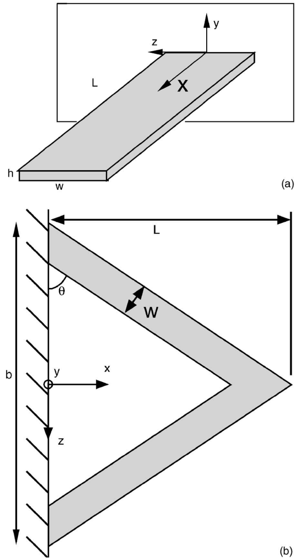
FIG. 1. Schematics of the two microw-scale cantilever geometries considered (not drawn to scale). Panel (a), a rectangular cantilever with aspect ratios L/h=98.5 , w/h=14.5 , and L/w=6.8 . The cantilever is composed of silicon with density \rho_c=2329 \text{ kg/m}^3 and Young's modulus E=174 \text{ GPa} . Panel (b), a V-shaped cantilever with aspect ratios L/h=233 , w/h=30 , and L/w=7.8 . The total width between the two arms normalized by the width of a single arm is b/w=10.36 . The cantilever platform is an equilateral triangle with \theta=\pi/3 . The cantilever is composed of silicon nitride with \rho_c=3100 \text{ kg/m}^3 and E=172 \text{ GPa} . The specific dimensions for the rectangular and V-shaped cantilever are given in Table I.
