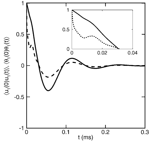
FIG. 6. The normalized autocorrelation of equilibrium fluctuations in the tip deflection \langle u_1(0)u_1(t) \rangle (solid line) and in tip angle \langle \theta_1(0)\theta_1(t) \rangle (dashed line) for the V-shaped cantilever. The inset shows a close-up of the dynamics for short time differences to illustrate the influence of the higher modes in the tip-angle measurements.
