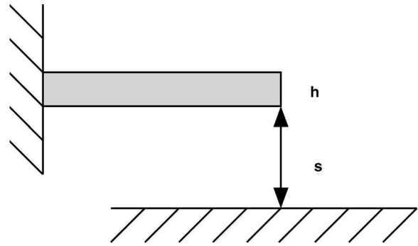
FIG. 8. A schematic of a cantilever a distance s away from a solid planar surface (not drawn to scale). The cantilever undergoes flexural oscillations perpendicular to the surface.
