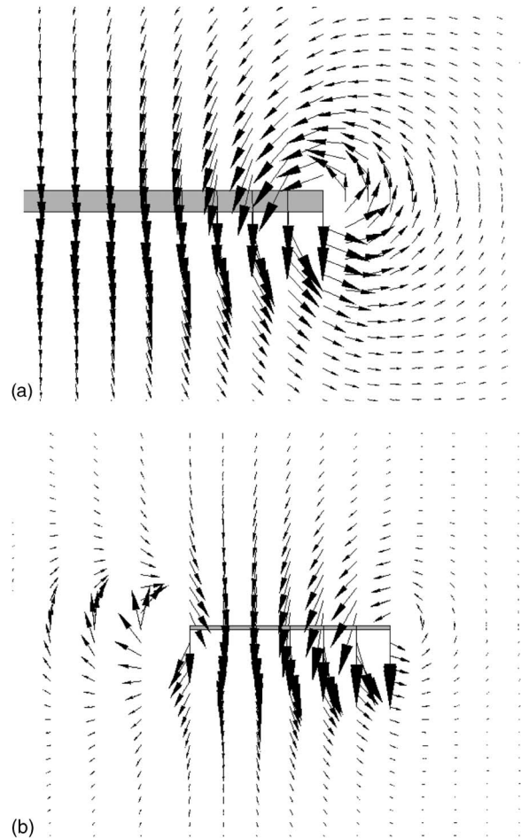
FIG. 4. The fluid flow near the tip of the cantilever as illustrated by the velocity vector field calculated from finite element numerical simulations. A cross section of the x-y plane at z=0 is shown (see Fig. 1) that is a close-up view of the tip region. The shaded region indicates the cantilever (because of the small deflections used in the simulations, that cantilever does not appear to be deflected). (a) The flow field near the tip of the rectangular cantilever. This flow field is at t=6 \mu\text{s} and the magnitude of the largest velocity vector shown is -0.3 \text{ nm/s} . (b) The flow field near the tip of the V-shaped cantilever. This flow field is at t=7.2 \mu\text{s} and the magnitude of the largest velocity vector shown is -26 \text{ nm/s} . The shaded region indicates the tip region where the two single arms have merged. The open region to the left is where the two single arms have separated, revealing the open region in the interior of the V-shaped cantilever.
