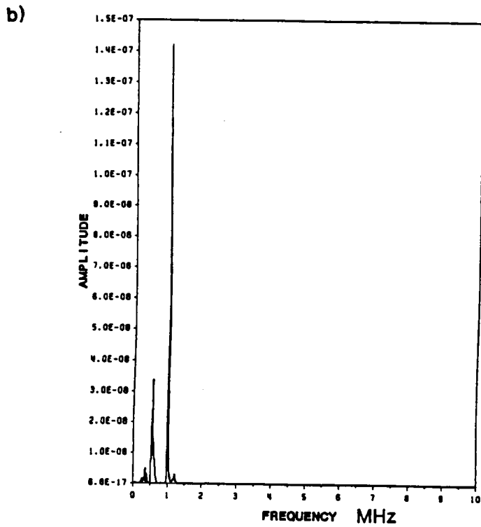
Figure 35. a)V/T and b)A/F, plots for .125" thick aluminum plate
