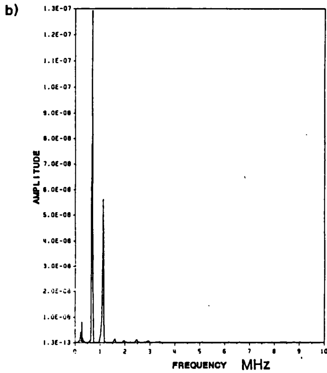
Figure 38. a)V/T and b)A/F, plots for Gr/Ep plate (24-ply, unidirectional)
