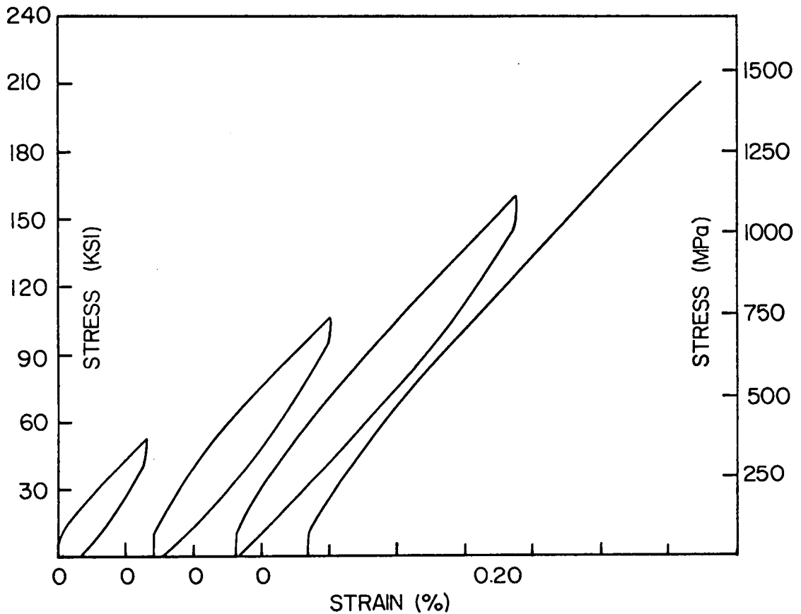
FIGURE 37. CYCLIC COMPRESSION STRESS-STRAIN DIAGRAM FOR [0/\pm 45/0]_s B/Al LAMINATE, F CONDITION.
