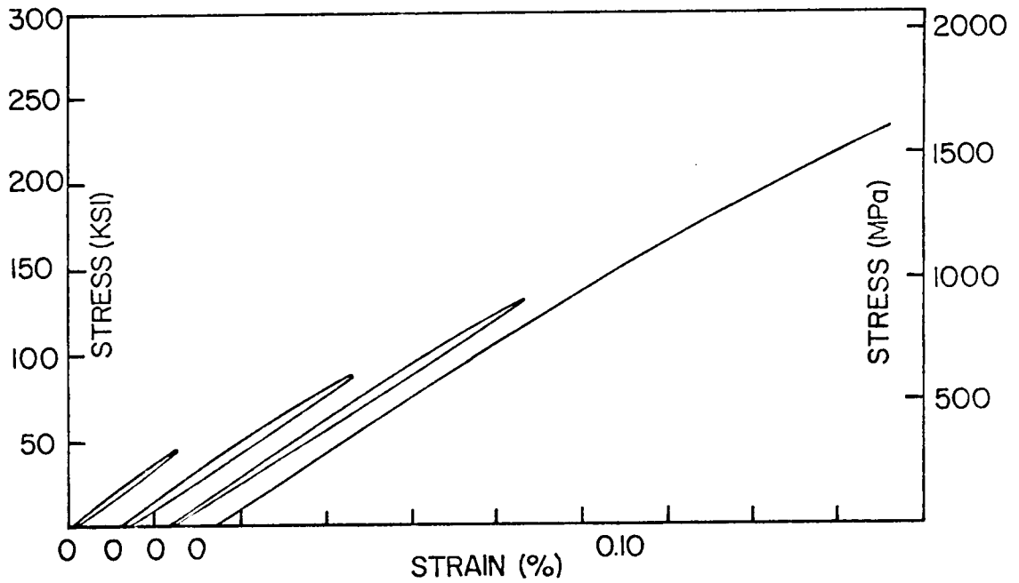
FIGURE 5. CYCLIC TENSION STRESS-STRAIN DIAGRAM FOR F CONDITION [0_8] B/Al LAMINATE.
