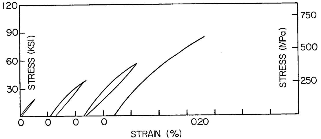
FIGURE 45. CYCLIC TENSION STRESS-STRAIN DIAGRAM FOR [0/\pm 45]_s B/Al LAMINATE, F CONDITION.
