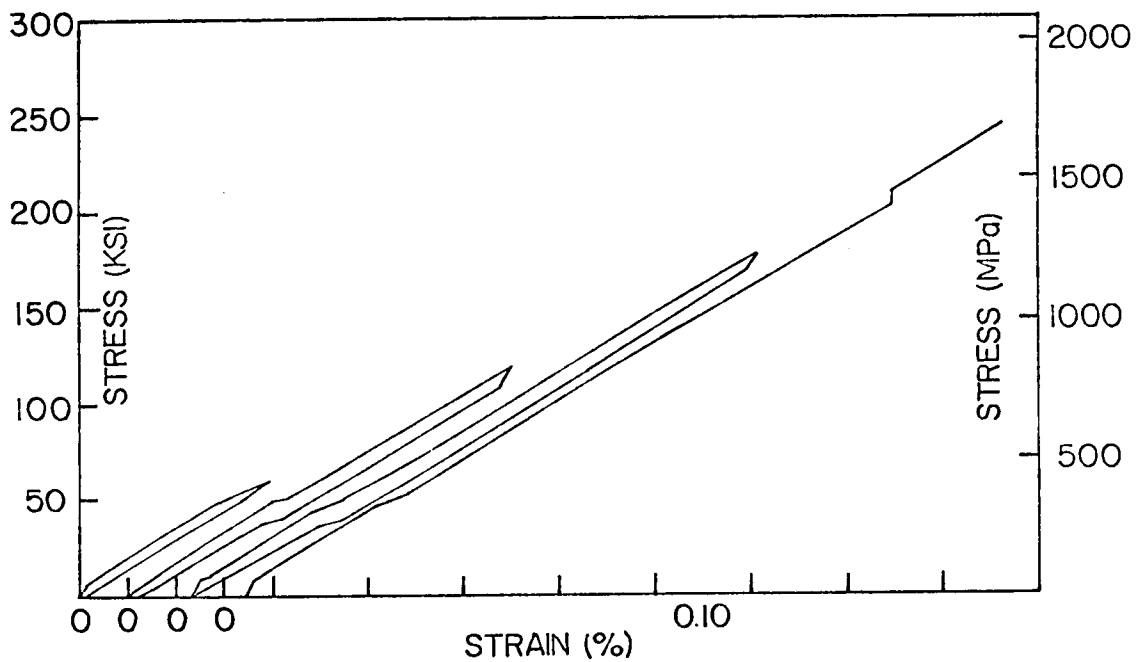
FIGURE 6. CYCLIC COMPRESSION STRESS-STRAIN DIAGRAM FOR F CONDITION [0_6] B/Al LAMINATE.
