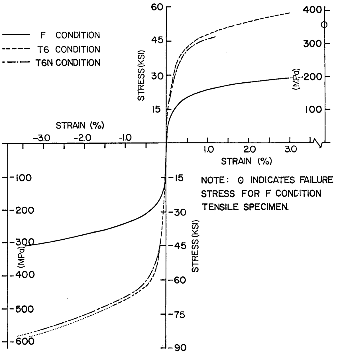
FIGURE 24. COMPARISON OF [\pm 45]_s B/Al LAMINATE WITH DIFFERENT TEMPER CONDITIONS IN TENSION AND COMPRESSION.
