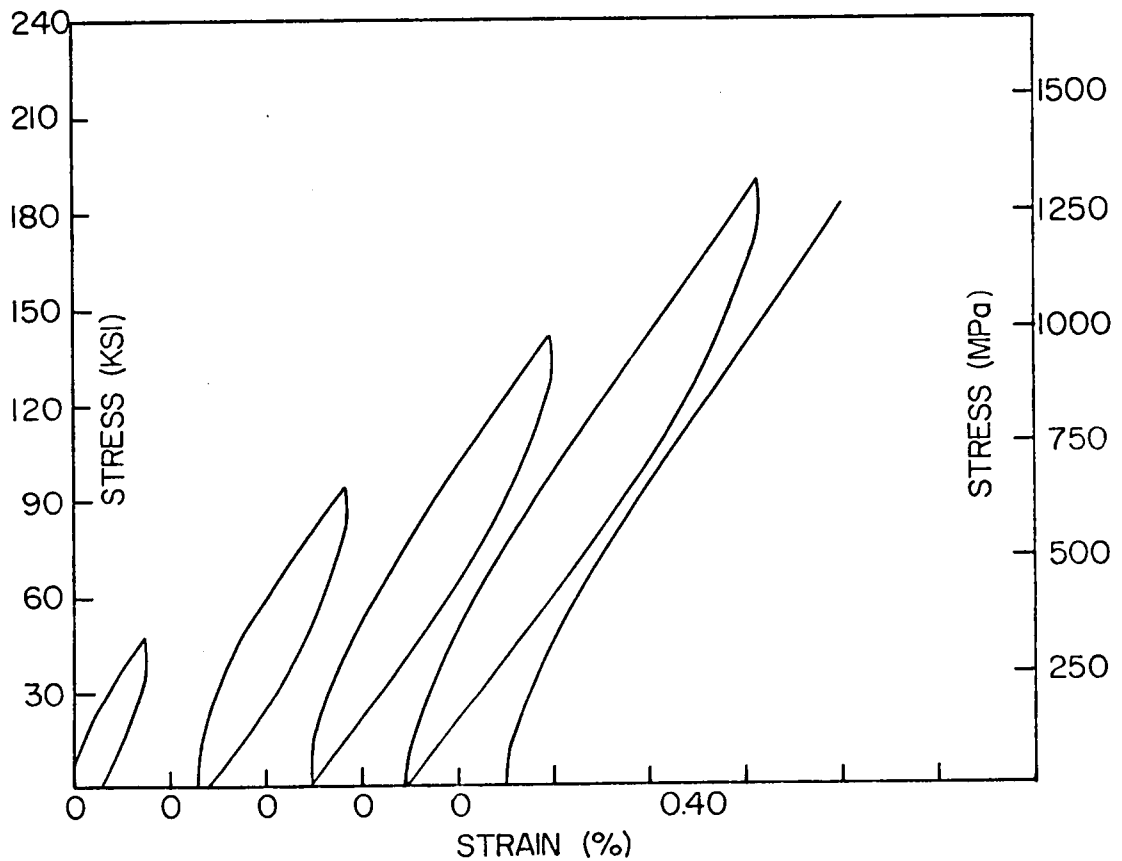
FIGURE 46. CYCLIC COMPRESSION STRESS-STRAIN DIAGRAM FOR [0/\pm 45]_s B/Al LAMINATE, F CONDITION.
