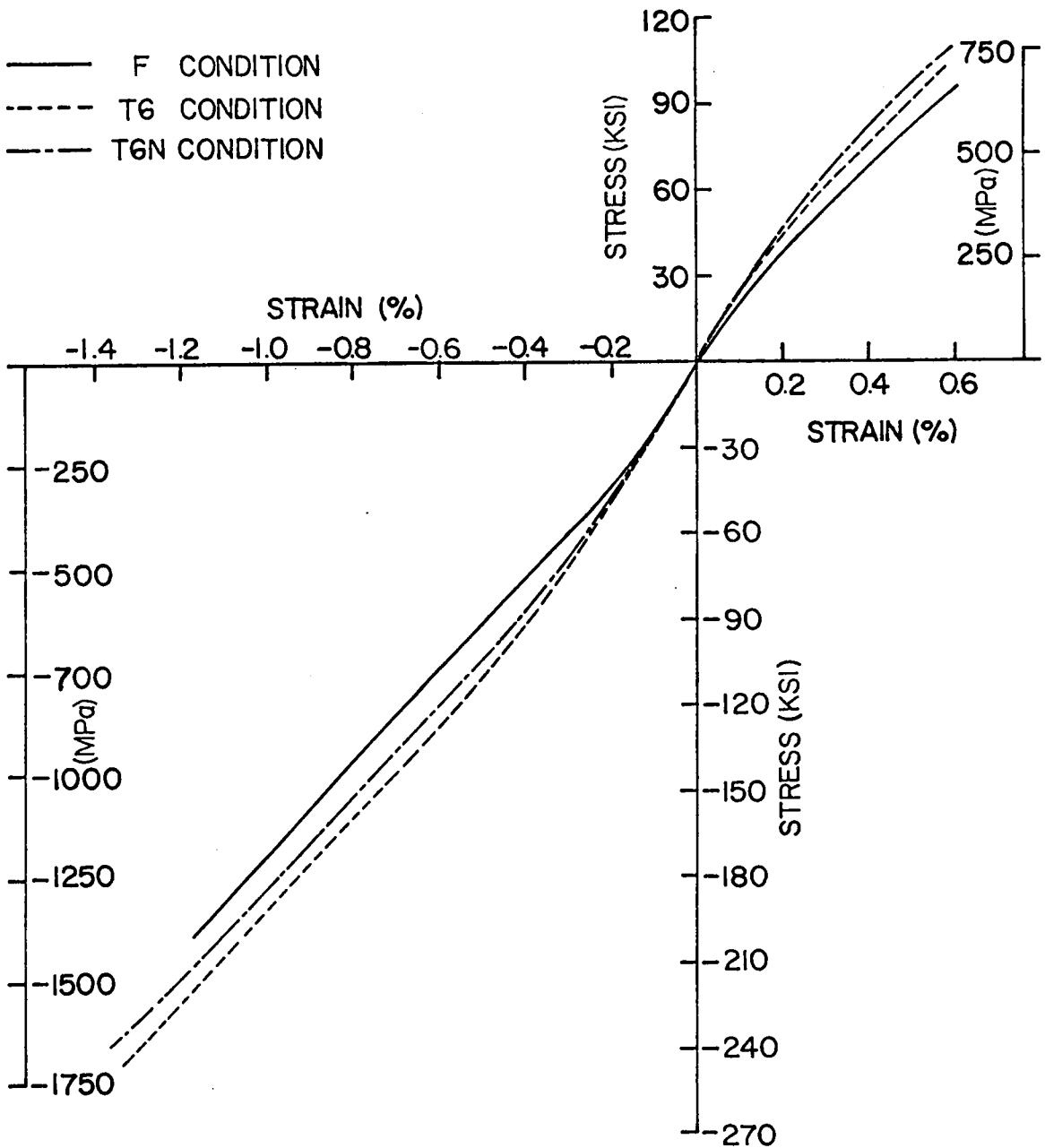
FIGURE 35. COMPARISON OF [0/\pm 45/0]_s B/Al LAMINATE WITH DIFFERENT TEMPER CONDITIONS IN TENSION AND COMPRESSION.
