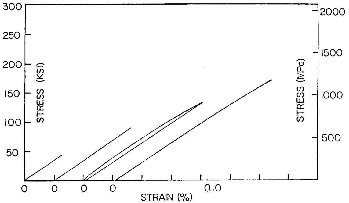
FIGURE 7. CYCLIC TENSION STRESS-STRAIN DIAGRAM FOR [0_8] B/AI LAMINATE, MODIFIED T4 CONDITION.
