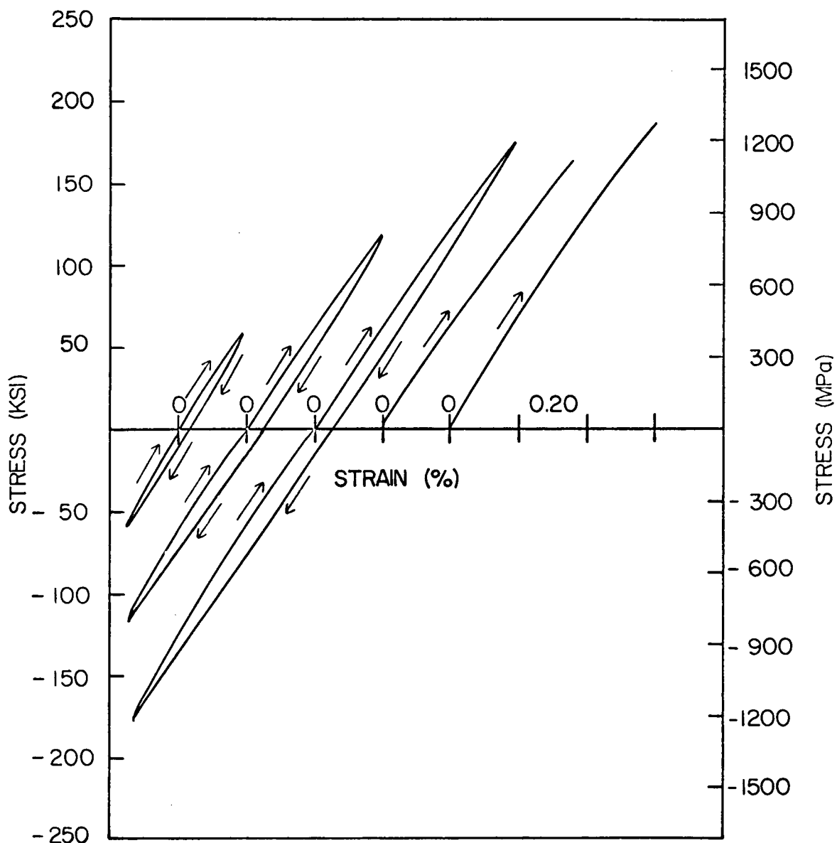
FIGURE 11. CYCLIC TENSION-COMPRESSION STRESS-STRAIN DIAGRAM FOR [0_6] B/AI LAMINATE, F CONDITION.
