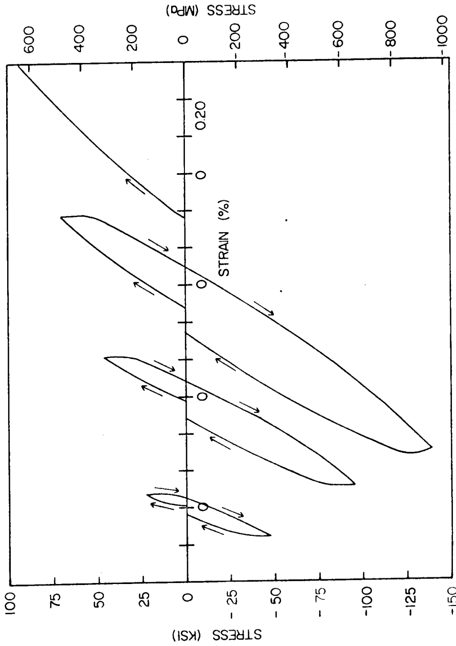
FIGURE 53. CYCLIC TENSION-COMPRESSION STRESS-STRAIN DIAGRAM FOR [0/\pm 45]_s B/AI LAMINATE, MODIFIED T6 CONDITION.
