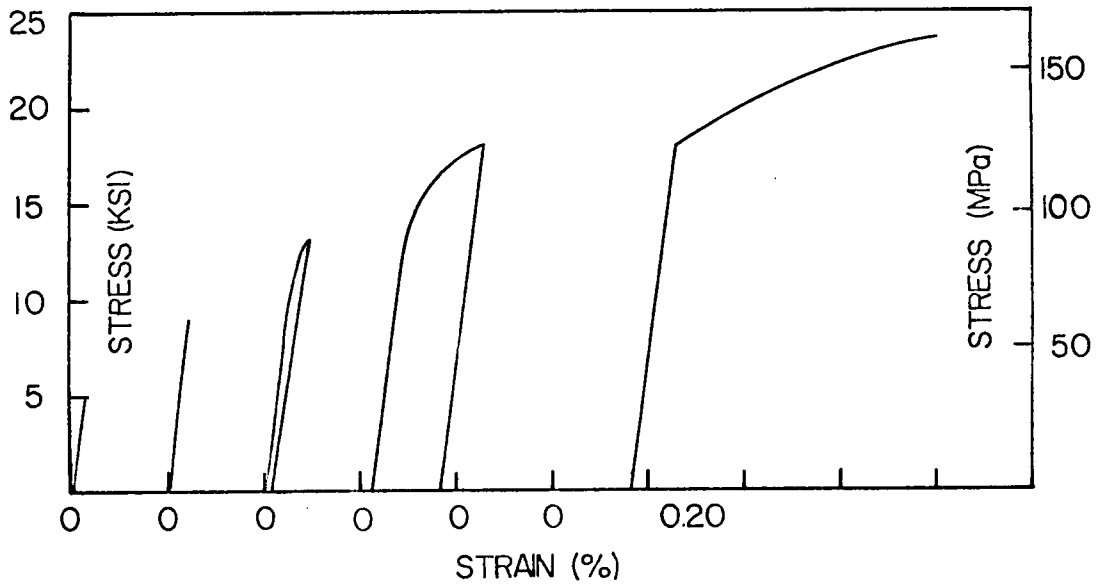
FIGURE 15. CYCLIC TENSION STRESS-STRAIN DIAGRAM FOR [90_8] B/Al LAMINATE, F CONDITION.
