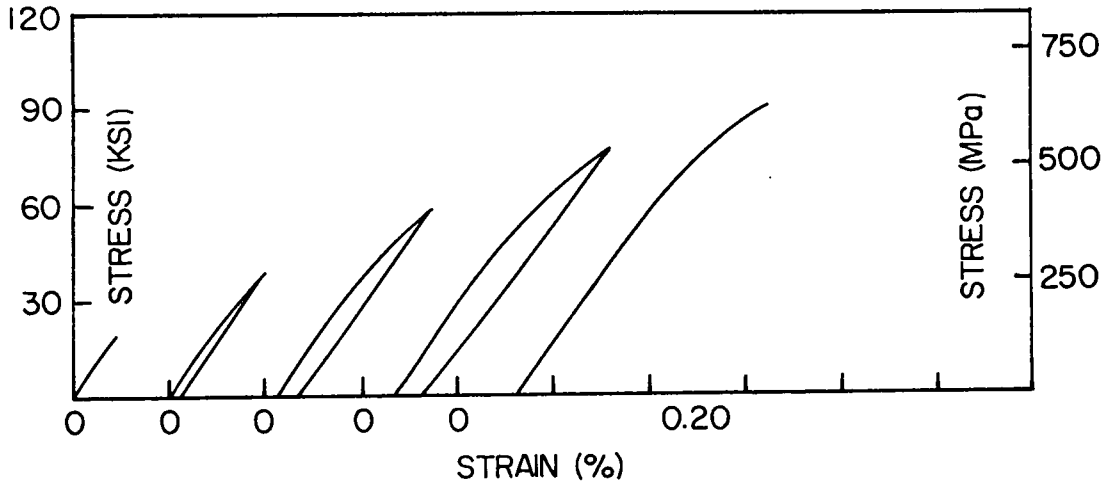
FIGURE 47. CYCLIC TENSION STRESS-STRAIN DIAGRAM FOR [0/+45]_s B/AI LAMINATE, T6 CONDITION.
