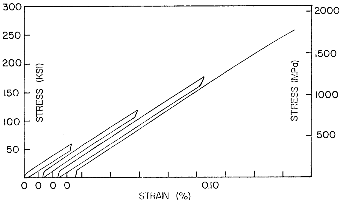
FIGURE 8. CYCLIC COMPRESSION STRESS-STRAIN DIAGRAM FOR [0_6] B/AI LAMINATE, T6 CONDITION.
