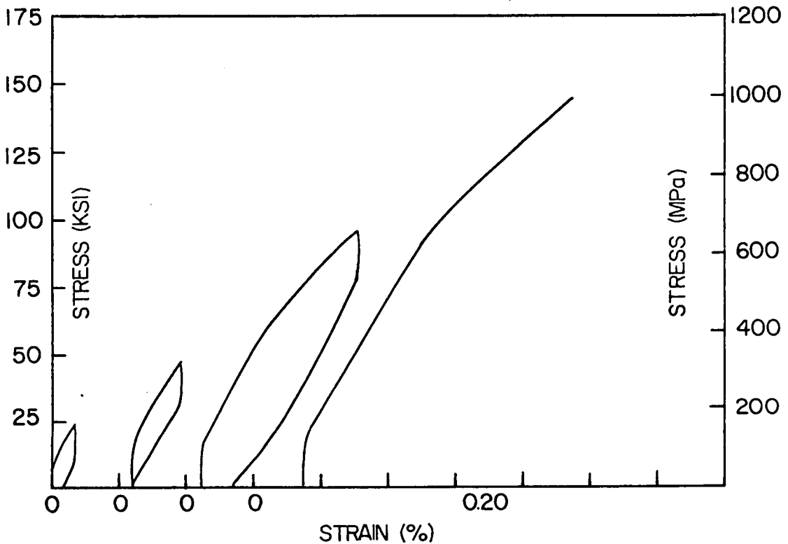
FIGURE 58. CYCLIC COMPRESSION STRESS-STRAIN DIAGRAM FOR [\pm 45/0]_s B/Al LAMINATE, MODIFIED T6 CONDITION.
