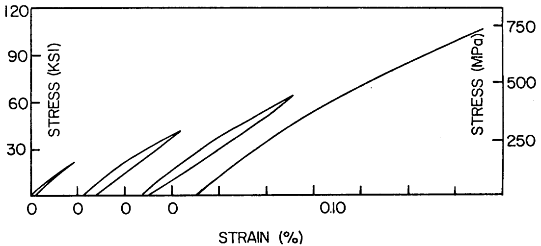
FIGURE 36. CYCLIC TENSION STRESS-STRAIN DIAGRAM FOR [0/\pm 45/0]_s B/Al LAMINATE, F CONDITION.
