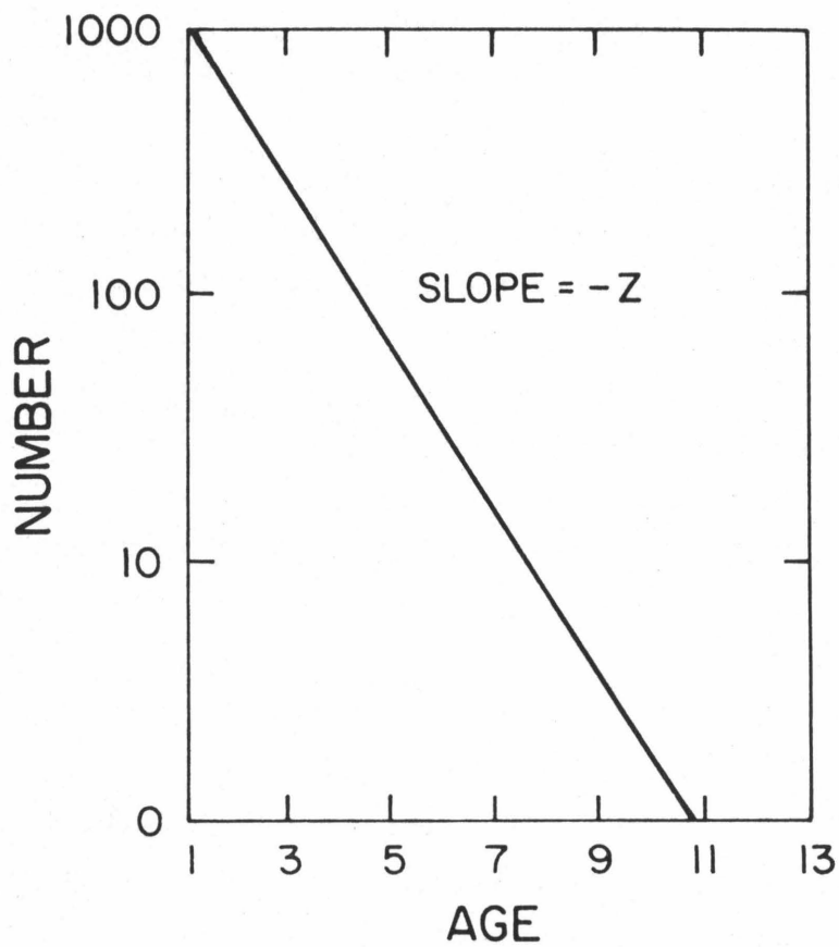
Figure IV-1: Upper - Relationship of the number of fish with time. Lower - Age-frequency distribution resulting from 50% survival and constant recruitment of 1,000 individuals per year (from Everhart, Eipper, and Youngs, 1975).
