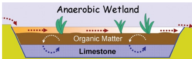
Figure 4. Simplified cross-sectional view of an anaerobic wetland. These systems are also called “composted wetlands” because the substrate layer generates alkalinity. The substrate can be comprised of biodegradable organic materials that are placed over limestone, as represented, or as an organic-limestone mixture. The circular arrows represent diffusion of treatment waters through the substrate which generates alkalinity.
