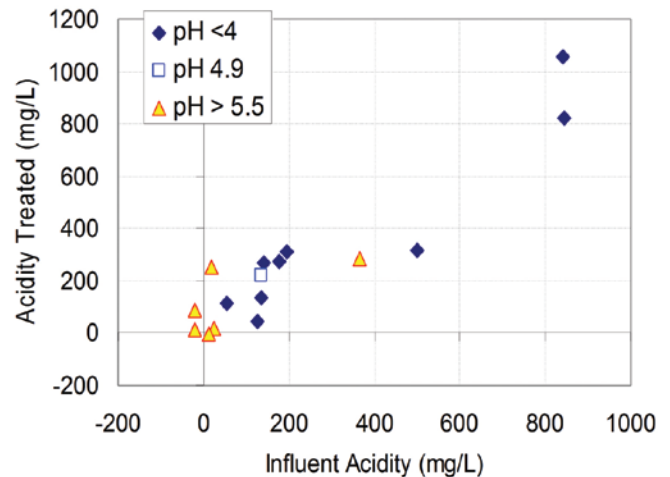
Figure 10. Performance of 16 open limestone channels, as documented by Skousen and Ziemkiewicz (2005), plotted by influent pH. All values charted are averages of multiple samples collected over extended time periods.
