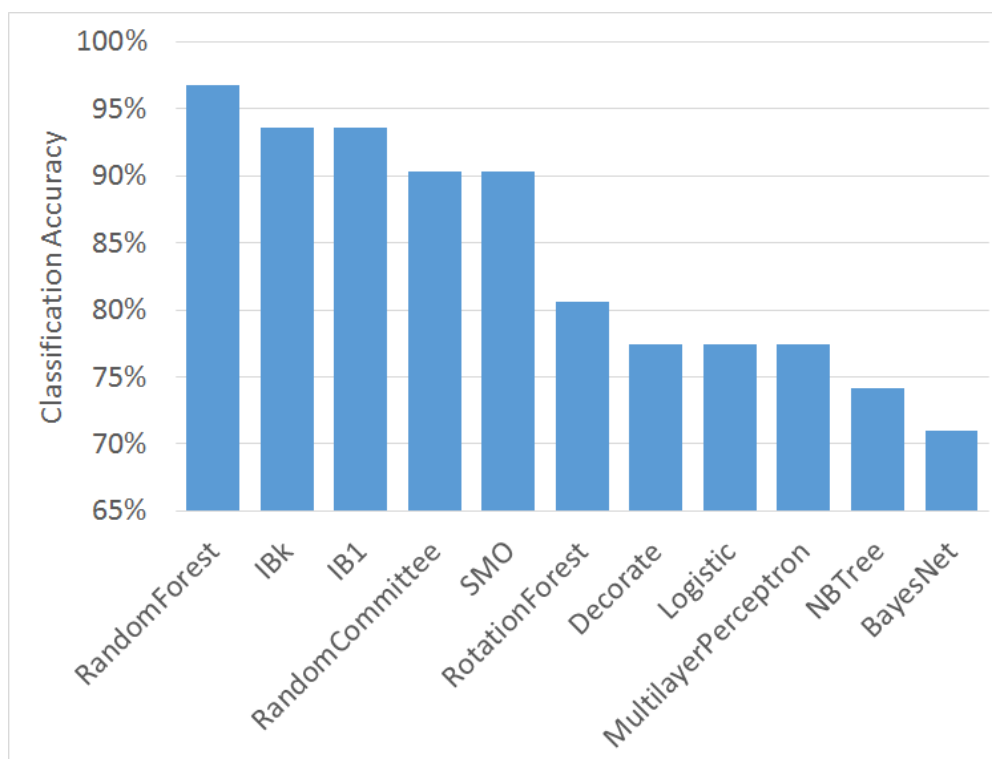
Figure 4.1: Randomly generated training and test sets were used to evaluate several different classification algorithms. Random forests were the most accurate and were therefore used for further analysis.
