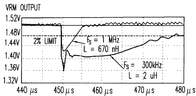
FIG.6 (PRIOR ART)
