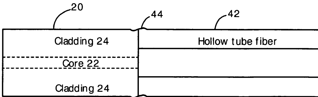
Fig. 3a Splice fiber and tube
