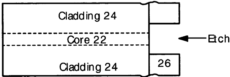
Fig. 5c Remove core by etching
