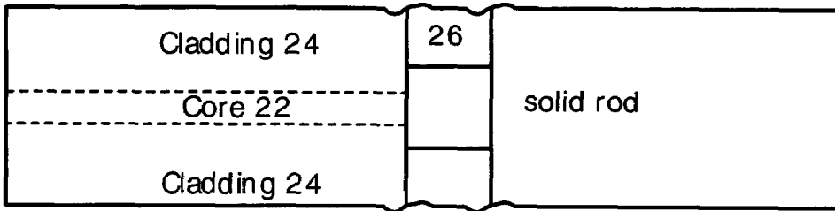
Fig. 3c Splice tube and rod
