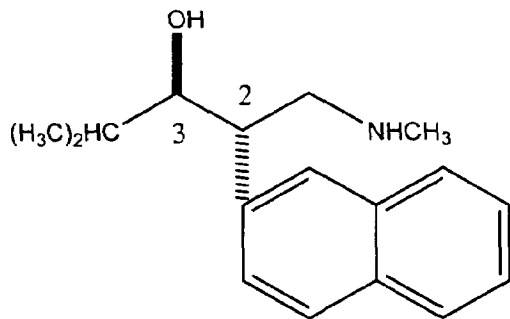
(2S,3R) - N -methyl-3-hydroxy-4-methyl-2-(2'-naphthyl)pentylamine
