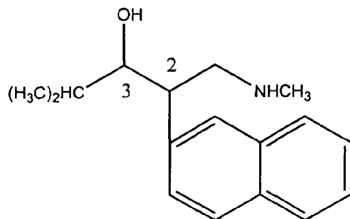
N -methyl-3-hydroxy-4-methyl-2-(2'-naphthyl)pentylamine
