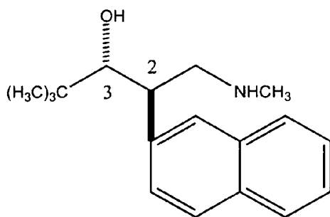
(2 R ,3 R )- N -methyl-3-hydroxy-4,4-dimethyl-2-(2'-naphthyl)pentylamine
