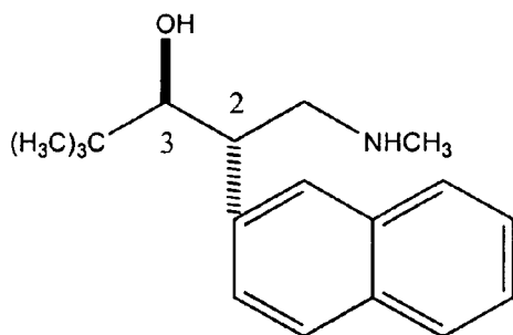
(2 S ,3 S )- N -methyl-3-hydroxy-4,4-dimethyl-2-(2'-naphthyl)pentylamine
