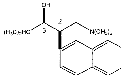
(2 R ,3 R )- N,N -dimethyl-3-hydroxy-4-methyl-2-(2'-naphthyl)pentylamine
