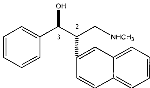
(2S,3S) - N -methyl-3-hydroxy-2-(2'-naphthyl)-3-phenylpropylamine
