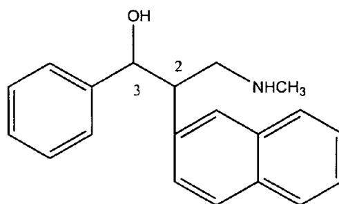
N -methyl-3-hydroxy-2-(2'-naphthyl)-3-phenylpropylamine
