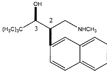
(2 R ,3 S )- N -methyl-3-hydroxy-4,4-dimethyl-2-(2'-naphthyl)pentylamine
