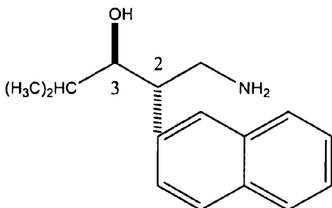
(2 S ,3 R )-3-hydroxy-4-methyl-2-(2'-naphthyl)pentylamine
