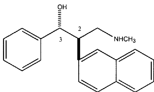
(2R,3R) - N -methyl-3-hydroxy-2-(2'-naphthyl)-3-phenylpropylamine
