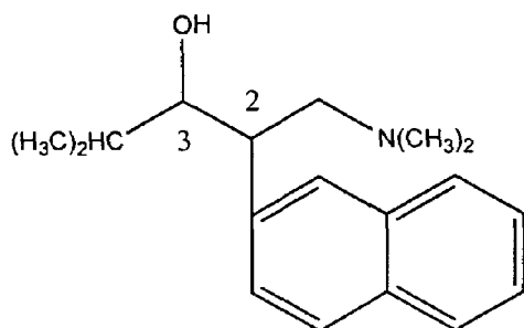
N,N -dimethyl-3-hydroxy-4-methyl-2-(2'-naphthyl)pentylamine
