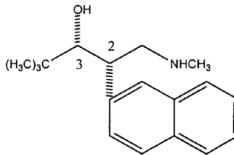
(2 S ,3 R )- N -methyl-3-hydroxy-4,4-dimethyl-2-(2'-naphthyl)pentylamine
