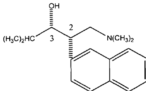
(2 S ,3 S )- N,N -dimethyl-3-hydroxy-4-methyl-2-(2'-naphthyl)pentylamine
