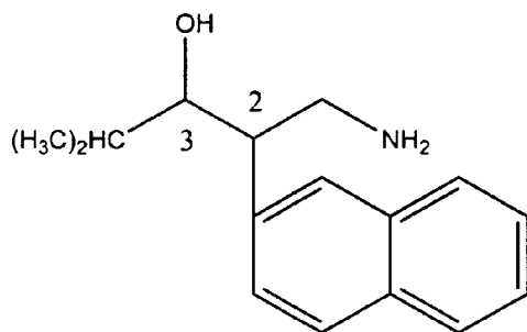
3-hydroxy-4-methyl-2-(2'-naphthyl)pentylamine
