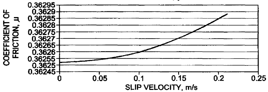
COEFFICIENT OF FRICTION, \mu DECELERATING
