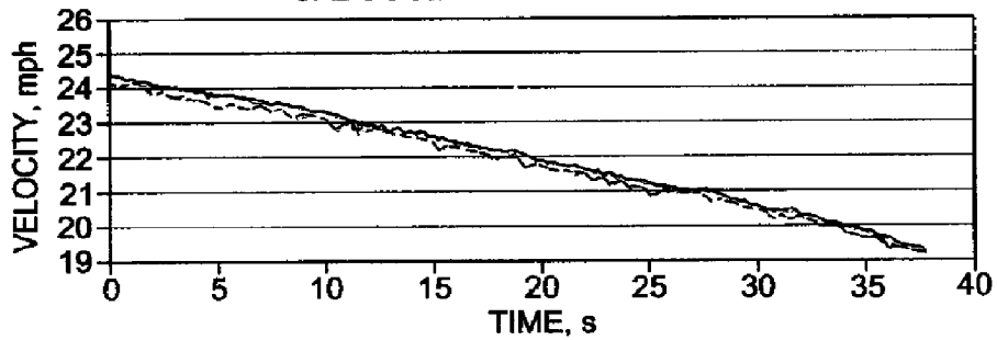
CABOOSE WHEEL SLIP VELOCITIES
