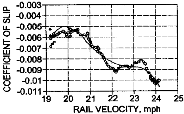
—○— COEFFICIENT OF SLIP
