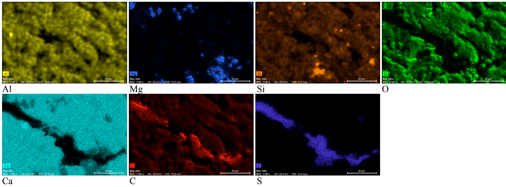
Figure A3.11: Specimen SBT-9-#3
