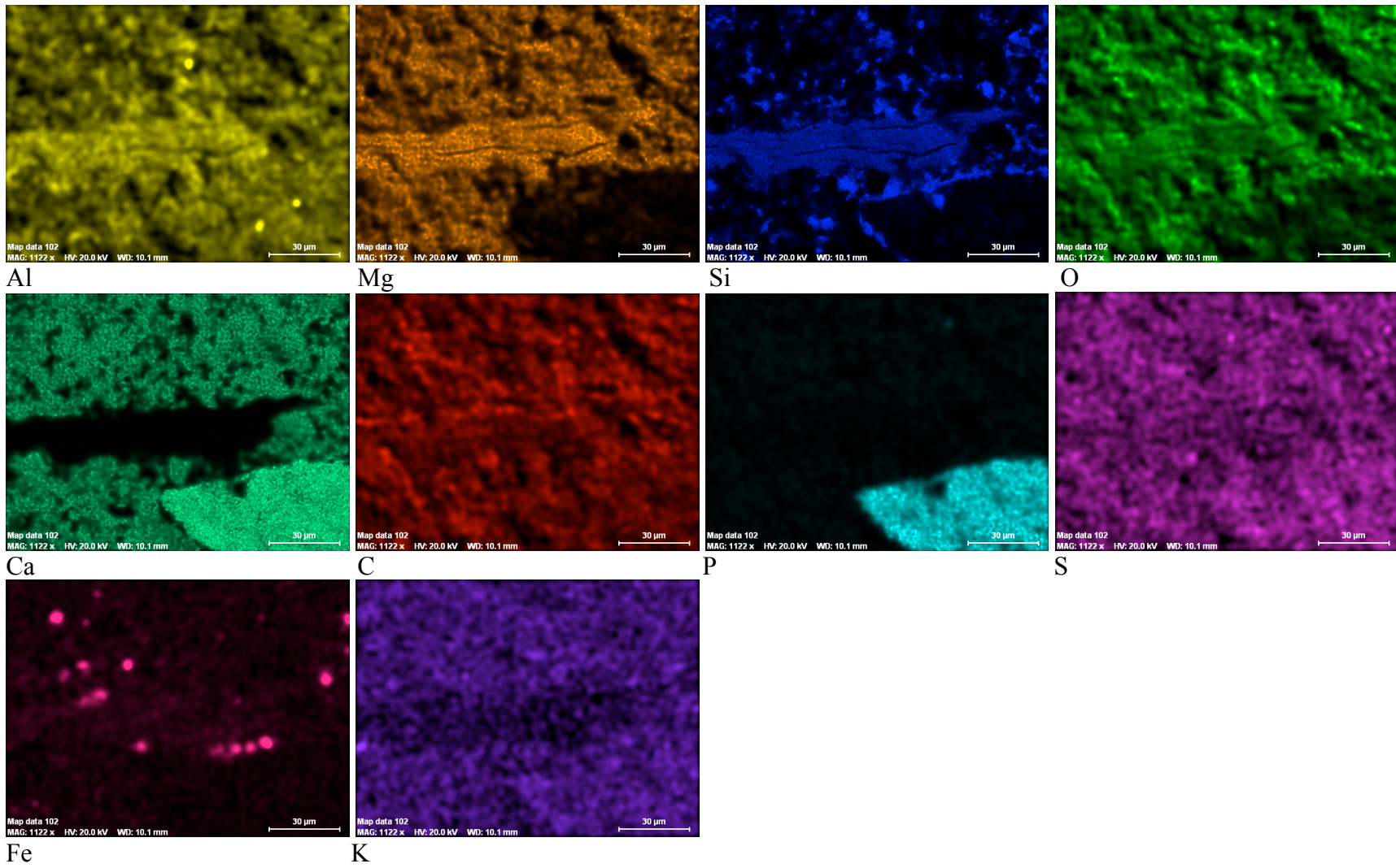
Figure. A3.3: Specimen 08-SX-DST3-3D1e-#1 zoom-in
