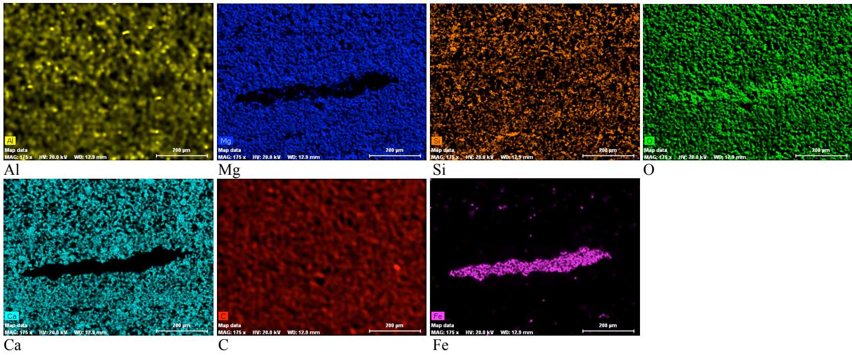
Figure A3.12: Specimen SFT-15-2-#9
