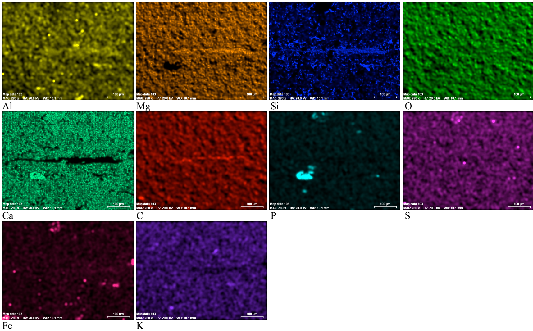
Figure. A3.4: Specimen 08-SX-DST3-3D1e-#2
