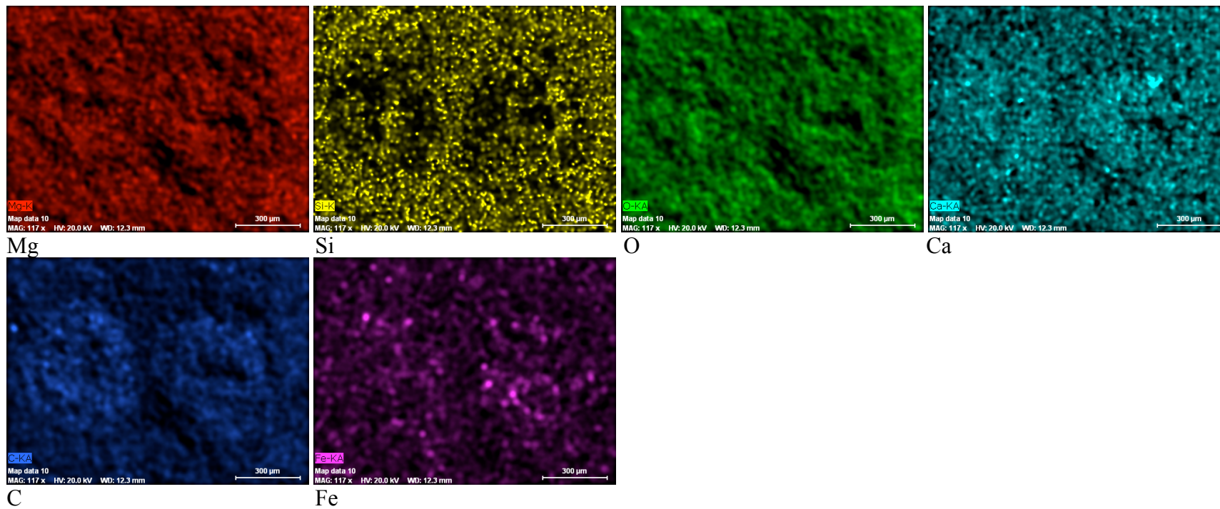
Figure A3.16: Specimens SFT-24-1-#6-7
