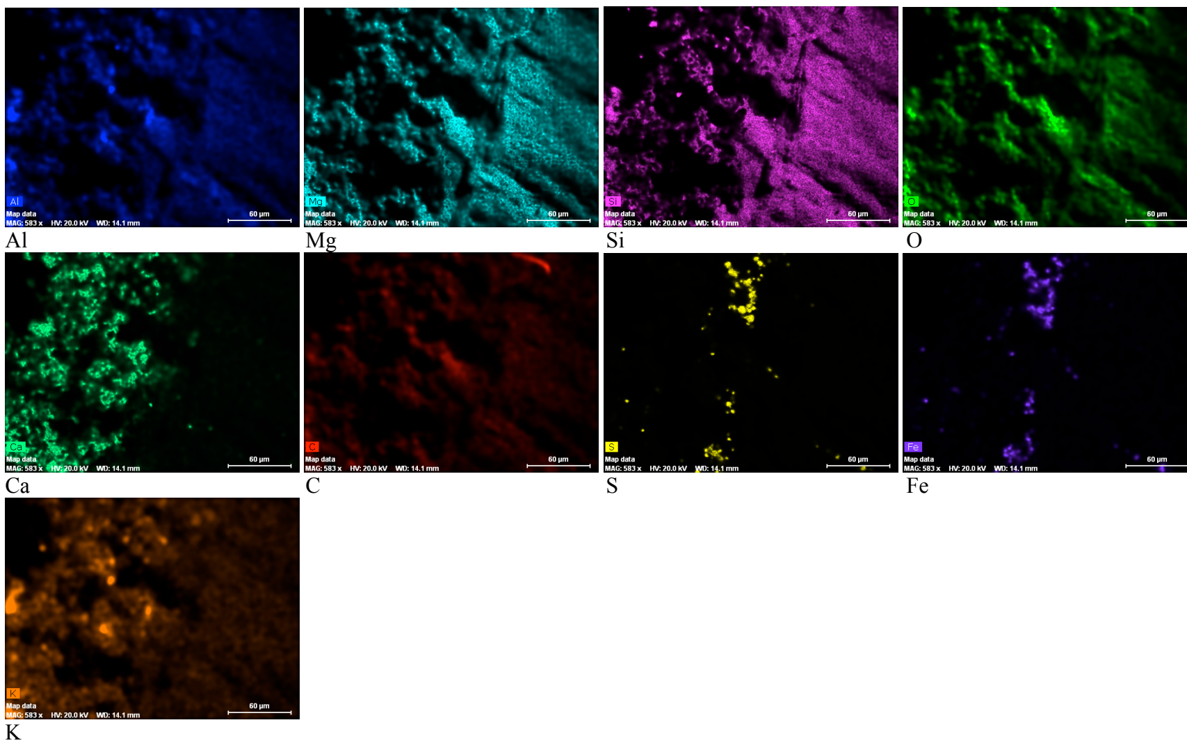
Figure A3.18: Specimen 09-SX-DST-F-#1
