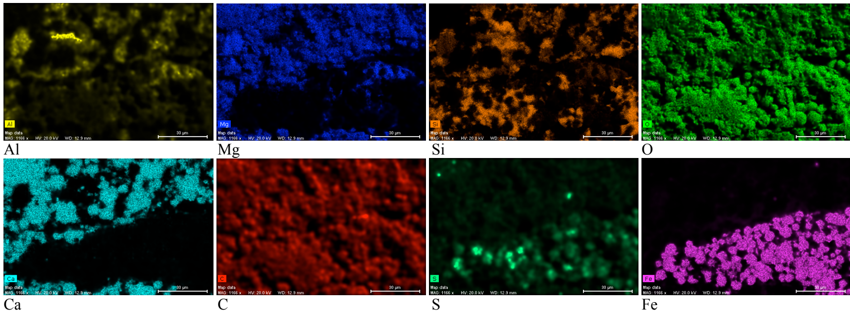
Figure A3.13: Specimen SFT-15-2-#9 zoom-in
