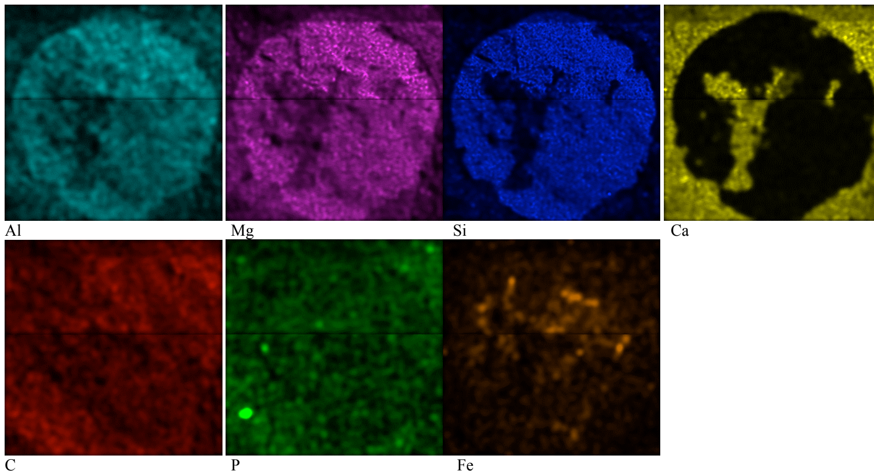
Figure A3.1: Specimen 08-SX-DST3-3B3-#5
