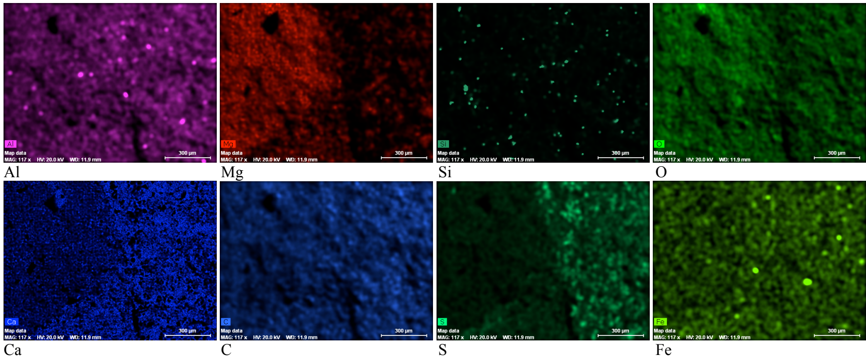
Figure A3.20: Specimen MH-7-#1
