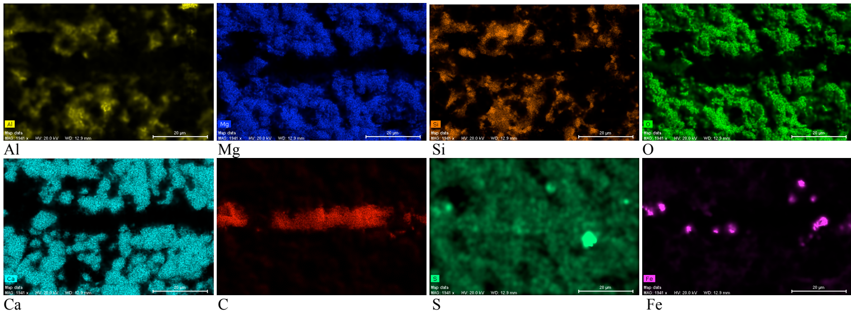
Figure A3.15: Specimen SFT-15-2-#11 zoom-in
