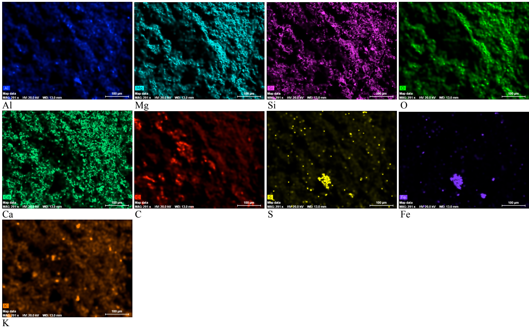
Figure A3.19: Specimen 09-SX-DST-F-#2
