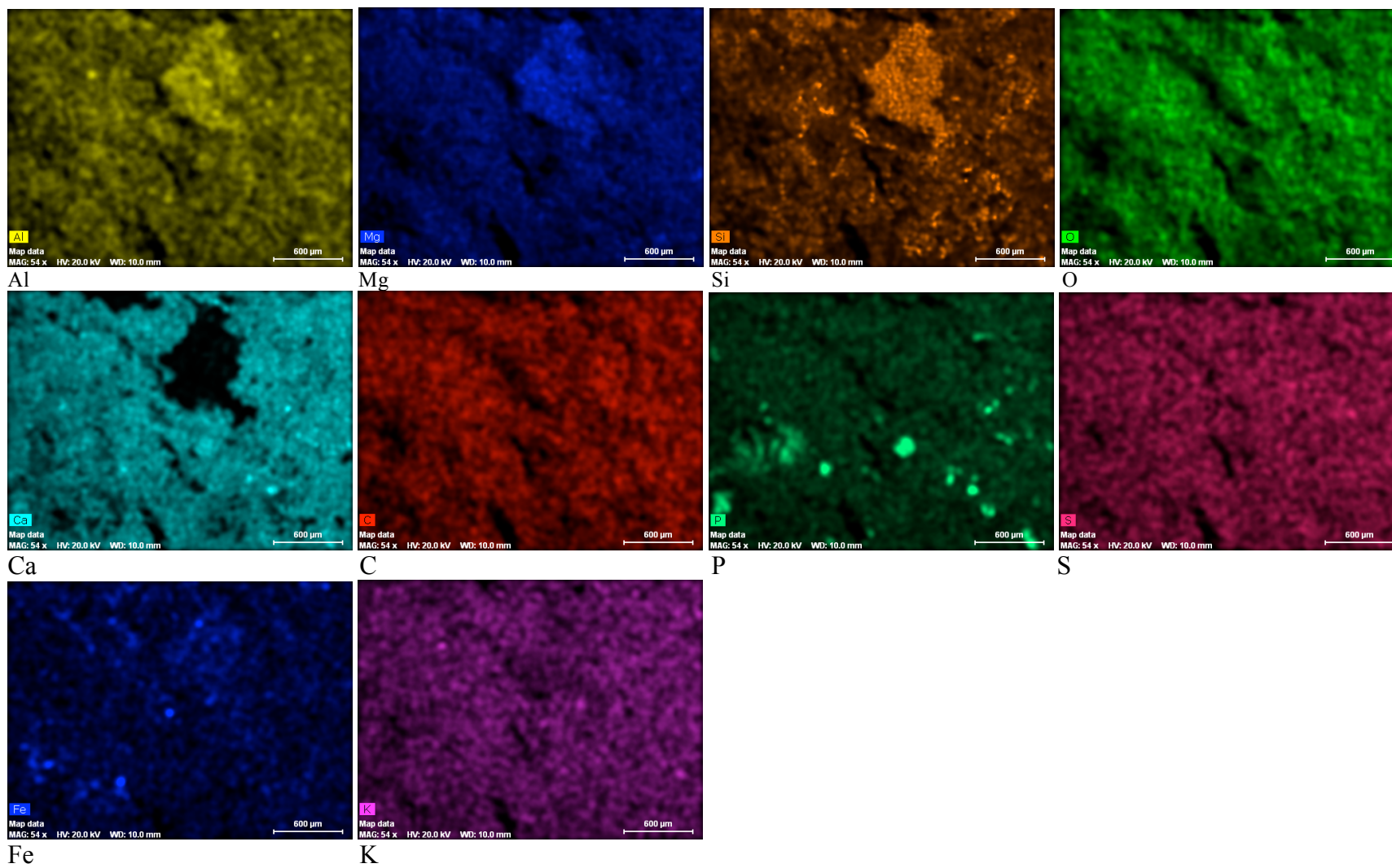
Figure A3.6: Specimen 08-SX-DST3-3E1a-#4
