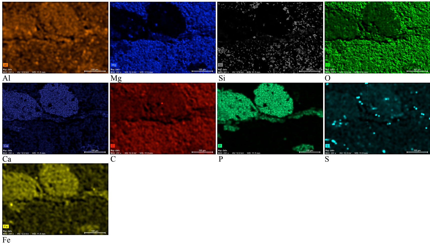
Figure A3.17: Specimen 09-SX-DST-A6-#1
