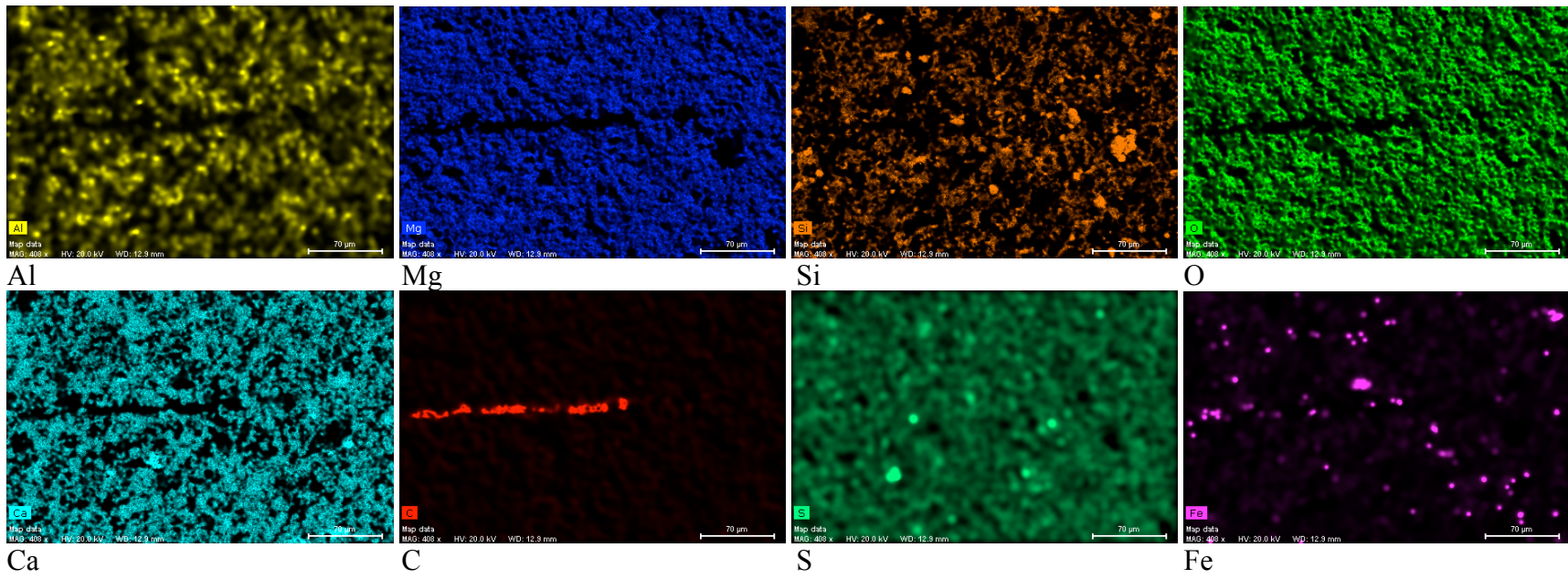
Figure A3.14: Specimen SFT-15-2-#11
