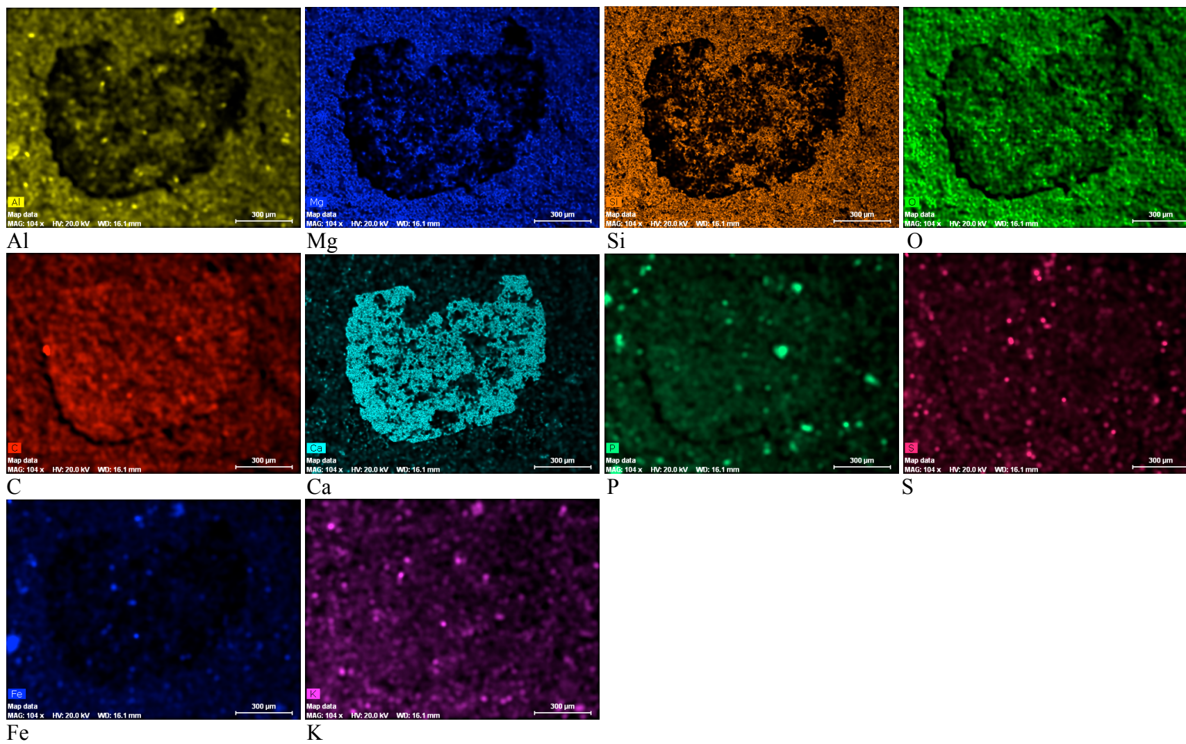
Figure A3.10: Specimen JLW-27Af-#2
