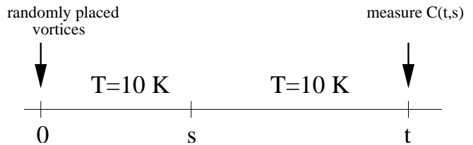
FIG. 1: Sketch of the measurement protocol. At t = 0 , straight vortex lines are initialized far out of equilibrium by placing them randomly in the system at T = 10 \text{ K} in the presence of weak point defects. The vortex lines are then allowed to relax for different waiting times s , before various two-time quantities, such as the height autocorrelation function C(t, s) , are measured.
