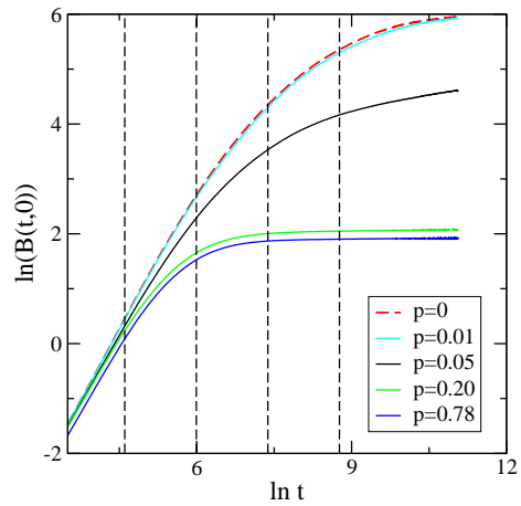
FIG. 7: (Color online) Mean-square displacement B(t, 0) vs. time t (in MCS) for interacting vortex lines with different values of the pinning strength p (system size L = 640 ; the data result from averaging over typically 100 independent runs). Due to the long-range interactions, the flux lines aim to maximize their separations, thus yielding values of B(t, 0) that are two orders of magnitude larger than in the absence of repulsive forces, compare Fig. 4. These displacements are impeded and vortex motion eventually stopped by the caging constraints of neighboring lines and pinning to attractive point defects. The (red) dashed line displays our data for a pure system, in the absence of pinning centers. The vertical dashed lines indicate the times t = 100, 400, 1600, \text{ and } 6400 MCS.
