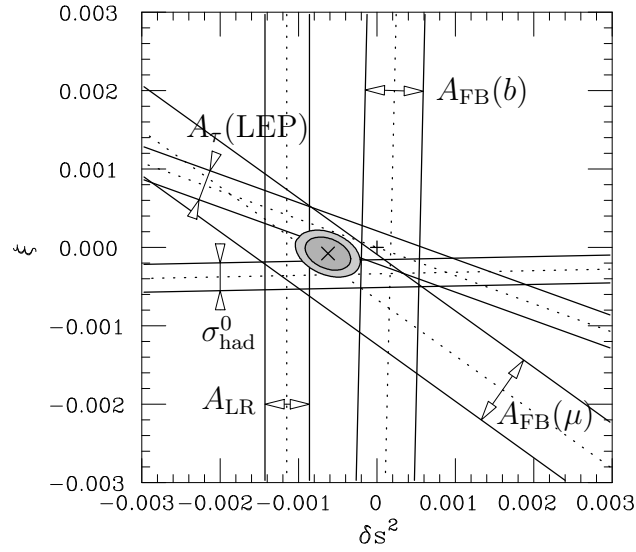
FIG. 3. The 68% and 90% confidence contours in the \delta s^2 - \xi plane for the \alpha = 0 , \beta = \gamma = 1.5 case. The 1\sigma bounds from the observables leading to the strongest constraints are also shown.
