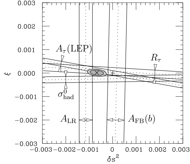
FIG. 2. The 68% and 90% confidence contours in the \delta s^2 - \xi plane for the \alpha = \beta = 0 , \gamma = 3 case. The 1\sigma bounds from the observables leading to the strongest constraints are also shown.
