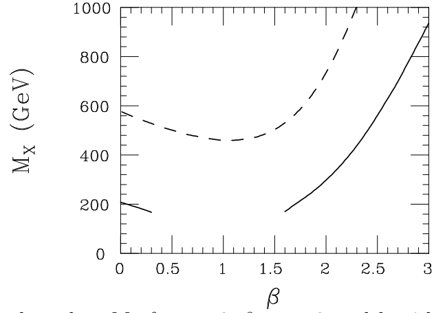
FIG. 5. The 2\sigma lower bound on M_X for \alpha = 0 , \beta + \gamma = 3 models with g_X = 0.65 (dashed line) and g_X = 0.35 (solid line). No bound exists for the g_X = 0.35 case between \beta \approx 0.4 and \beta \approx 1.5 .
