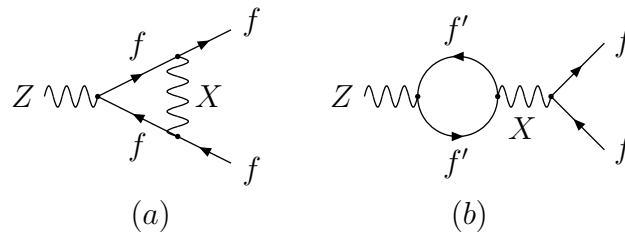
FIG. 1. One-loop vertex corrections to Z \rightarrow f\bar{f} . Wavefunction renormalization corrections are not shown.
