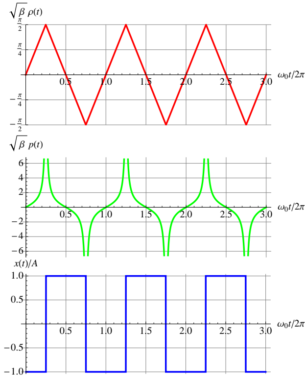
FIG. 6: The classical behavior of a positive mass particle in a harmonic oscillator potential with modified Poisson brackets, Eq. (66), in the limit m \rightarrow \infty with C = 2mE\beta where E and \beta are kept fixed. \rho(t) and x(t) take on the behavior of the position and momentum of a particle in an infinite square well.
