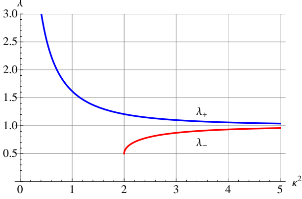
FIG. 2: Plots of \lambda_+ (blue) and \lambda_- (red), Eq. (23), as functions of \kappa^2 = \beta\hbar\sqrt{k|m|} .
