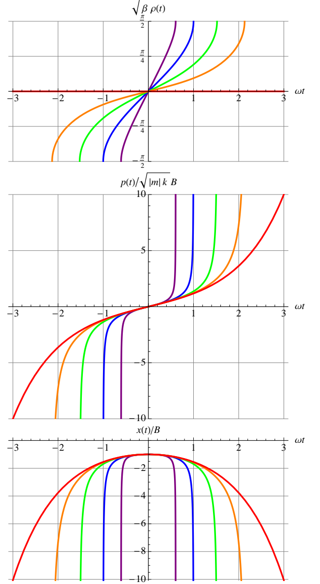
FIG. 7: The dependence of the classical behavior of a negative mass particle in a harmonic oscillator potential on the parameter C = -2\mu E\beta = -\beta|m|kB^2 , where E is the particle's energy, and B is the distance of closest approach to the origin in x -space. Note that due to the negative mass, p(t) is negative when \dot{x}(t) is positive, and vice versa. The undeformed \beta = 0 case is shown in red. The other four cases are C = -\frac{1}{16} (orange), C = -\frac{1}{4} (green), C = -1 (blue), and C = -4 (purple).
