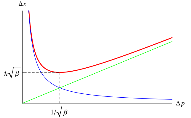
FIG. 1: The lower bound on \Delta x as a function of \Delta p when they obey the minimal length uncertainty relation, Eq. (2), is shown in red. The blue line indicates \Delta x = (\hbar/2)(1/\Delta p) while the green line indicates \Delta x = (\hbar\beta/2)\Delta p .
