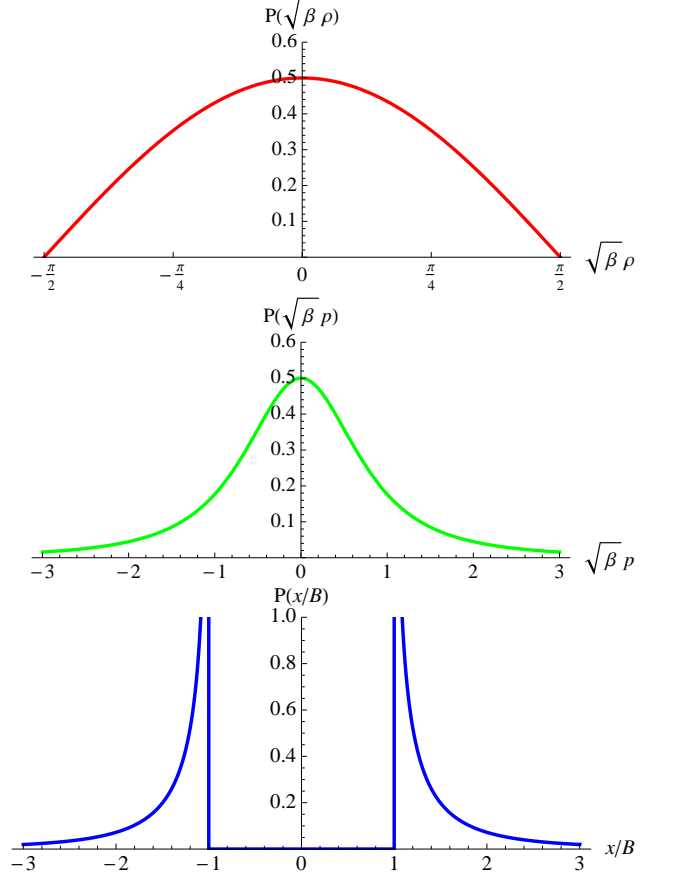
FIG. 12: Classical probabilities in \rho -, p -, and x -spaces of a negative mass particle in a harmonic oscillator potential for the case C = -2|m|E\beta = -1 . The time dependence of this solution was shown in Fig. 11. Though the trajectory of the particle is not confined to a finite region of phase space, the classical probabilities of finding the particle near the phase-space-origin is still finite due to the finiteness of the time it takes for the particle to traverse the entire trajectory.
