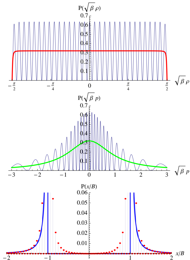
FIG. 13: Comparison of quantum and classical probabilities in \rho -, p -, and x -spaces for a negative mass particle in a harmonic oscillator potential for the case \lambda = \frac{3}{4} and n = 30 , which corresponds to the classical C = -2|m|E\beta = -5044 . The quantum distribution in x -space is discrete due to the existence of the minimal length. There is also some seepage of the probability into classically forbidden regions in x -space as is expected of quantum probabilities.
