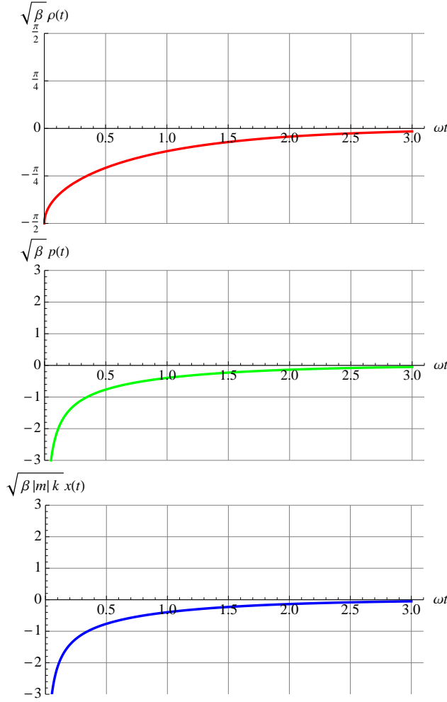
FIG. 10: The classical behavior of a zero-energy particle with negative mass in a harmonic oscillator potential. The particle starts out at x = -\infty at time t = 0 and asymptotically approaches the origin.
