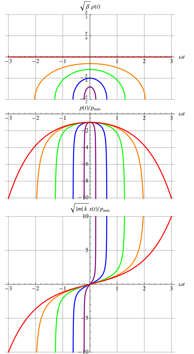
FIG. 8: The dependence of the classical behavior of a negative mass particle in a harmonic oscillator potential on the parameter C = -2|m|E\beta = \beta p_{\min}^2 , where E is the particle's energy, and p_{\min} is the momentum of the particle at the origin x = 0 . The undeformed \beta = 0 case is shown in red. The other four cases are C = +\frac{1}{16} (orange), C = +\frac{1}{4} (green), C = +1 (blue), and C = +4 (purple).
