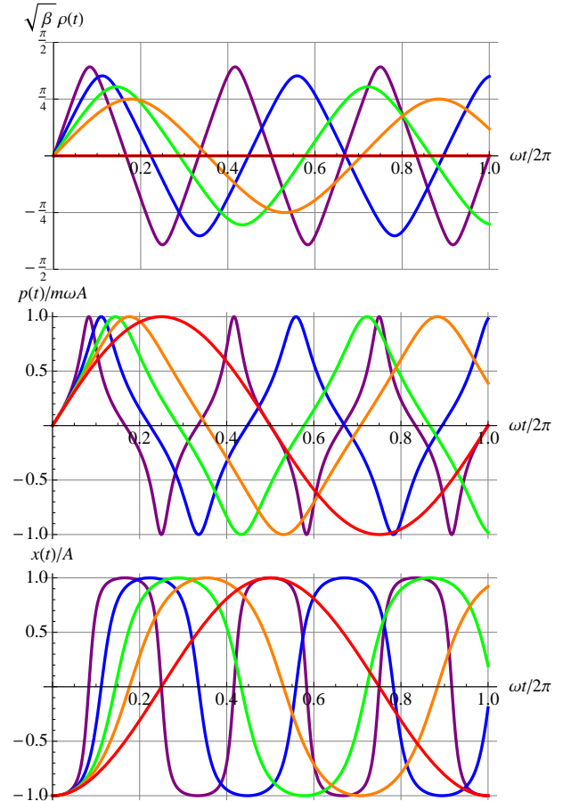
FIG. 5: The dependence of the classical behavior of a positive mass particle in a harmonic oscillator potential on the parameter C = 2mE\beta = \beta m^2 \omega^2 A^2 , where E is the particle’s energy, and A is the amplitude of the oscillation in x . The undeformed \beta = 0 case is shown in red. The other four cases are C = 1 (orange), C = 2 (green), C = 4 (blue), and C = 8 (purple).
