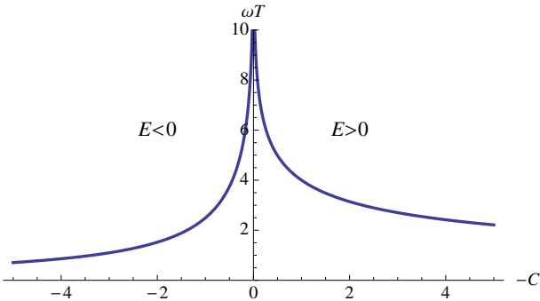
FIG. 9: \omega T as a function of -C = 2|m|E\beta , where \omega = \sqrt{k/|m|} , and E is the particle's energy. T/2 is the time it takes for the particle to traverse the entire trajectory.
