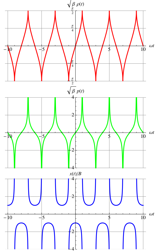
FIG. 11: The periodic behavior of the negative-mass particle in a harmonic oscillator potential in compactified x -space. The example shown is for C = -1 .
