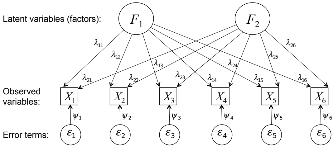
Figure 1: An illustrative example of factor analysis with six observed variables (survey question responses) that can be effectively summarized in terms of two latent variables (factors). Note that the survey question responses are observed with error (the \epsilon_i terms) and the question responses are weighted linear combinations of the factors (where the weights are the \lambda_{ij} s).
