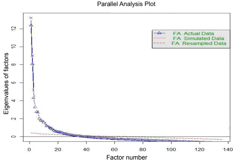
Figure 2: Parallel analysis plot for country A, where the eigenvalues for 27 factors were greater than those from the simulated data (the blue line is greater than the dashed red line), so we set r = 27 . Sensitivity analysis subsequently confirmed that r = 27 was appropriate for country A.
