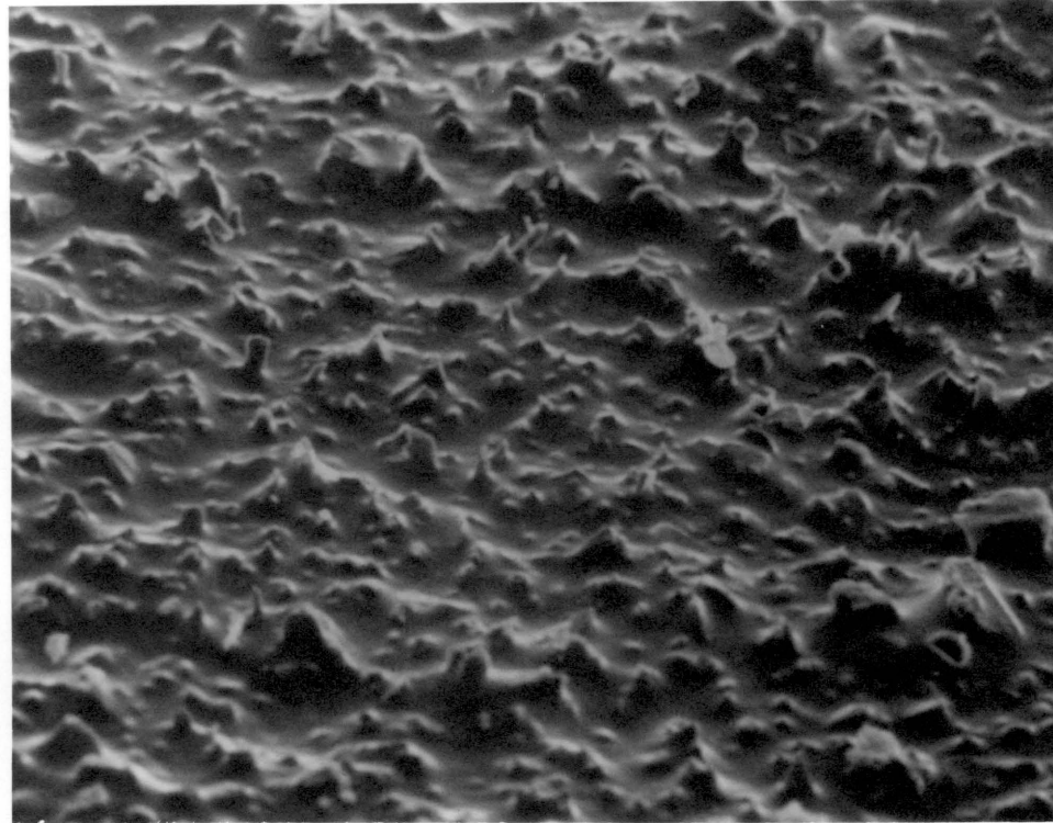
Fig. 4. Electron microscope photograph of 3M 600 grit silicon carbide sandpaper used in the experiments.
