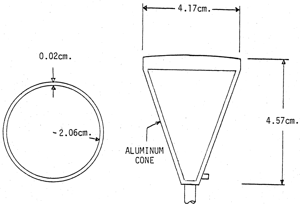
ELEMENT HEAD FOR CONFIGURATION 2 &amp; 3.
