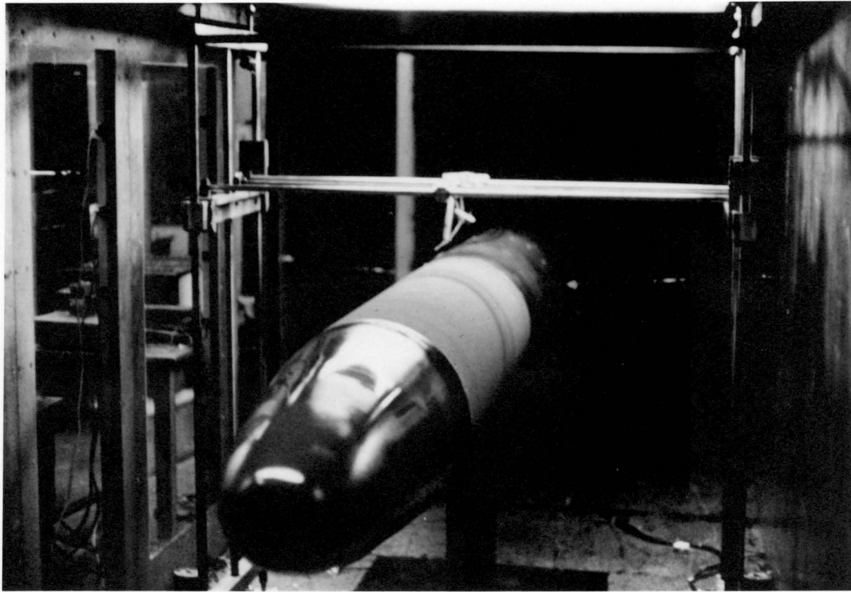
Fig. 8. The axisymmetric model and automatic traverse used in the experiments.
