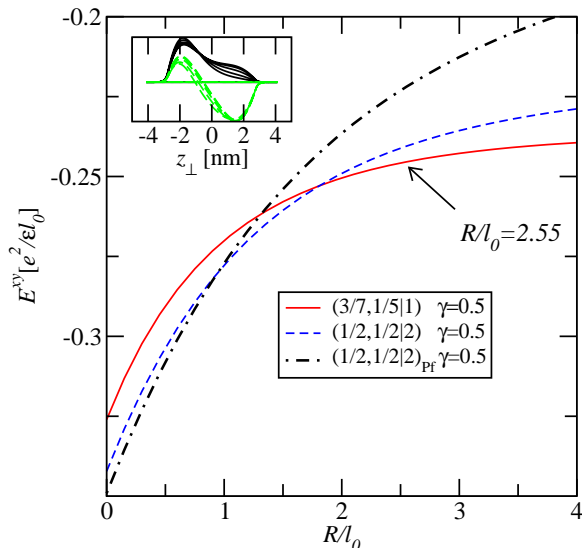
Figure 2: In-plane correlation energies of several states, Eqs. (3) and (4), at \gamma = 0.5 plotted versus the inter-subband interaction parameter R . The arrow indicates the parameter relevant for the tilted well samples of Ref. [15] where the (3/7, 1/5|1) state is shown to have the lowest correlation energy at \gamma = 0.5 . Inset: Normalized lowest (solid) and first (dashed) subband wavefunctions plotted versus position in the tilted quantum well for several \gamma between 0 and 1. In the limit \gamma \rightarrow 0 the subbands localize to mimic layer states.
