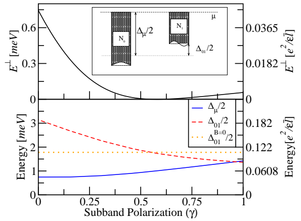
Figure 1: Top: Confinement energy plotted as function of subband polarization for parameters corresponding to tilted wide well samples of Ref. [15]. The right axis shows Coulomb units in terms of the fixed magnetic length, \bar{l} , obtained for \nu = 1/2 and \rho = 1.72 \times 10^{11} \text{ cm}^{-2} . Bottom: The same but for the subband energy difference (dashed) and the chemical potential offset (solid). The dotted line plots the B = 0 subband energy difference. Inset: Schematic showing partial subband occupancy captured by an effective chemical potential.
