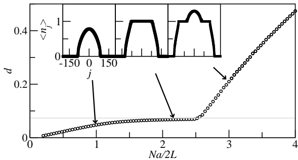
Figure 3. The circles indicate double occupancy fraction versus particle number in a trapped system ( L = 50 ) at T = 0 for half filling at the trap center and U/t = 8 computed using BA-LDA. The solid line is the bulk value in the Mott insulating ground state (Eq. 4). The insets, from left to right, show the corresponding density as function of position in the trap for 100, 216, and 300 particles, respectively.
