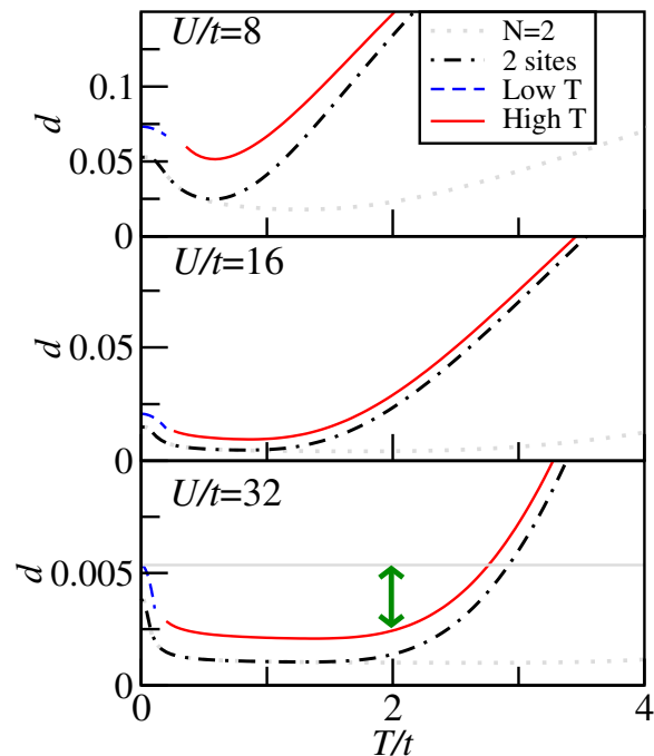
Figure 1. Double-occupancy fraction versus temperature for the uniform 1D Hubbard model at half filling for several U/t . The dashed line indicates the low- T expansion (5); the solid line is the fourth-order high- T expansion; the dot-dashed line is the exact result for a two-site Hubbard model in the grand canonical ensemble; and the dotted line is the same but with the number of particles set to exactly two. At low T , non-zero d arises from coherent quantum fluctuations, but at intermediate temperatures this coherence is destroyed, leading to a suppression of d(T) shown by the double-headed arrow.
