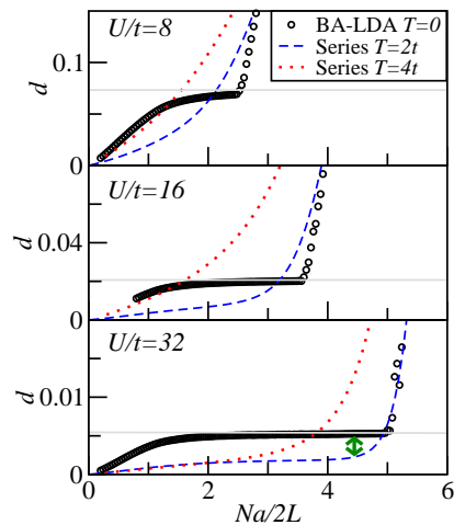
Figure 4. The circles and solid line show the same as Fig. 3 but for three values of U . The dashed (dotted) lines show results computed from an exact second order high temperature series expansion at T = 2t ( T = 4t ). The plateau at finite d indicates strong quantum fluctuations. The double arrow in the bottom panel indicates the observable effects of weak thermal fluctuations in a trap and corresponds to the double arrow in Fig. 1.
