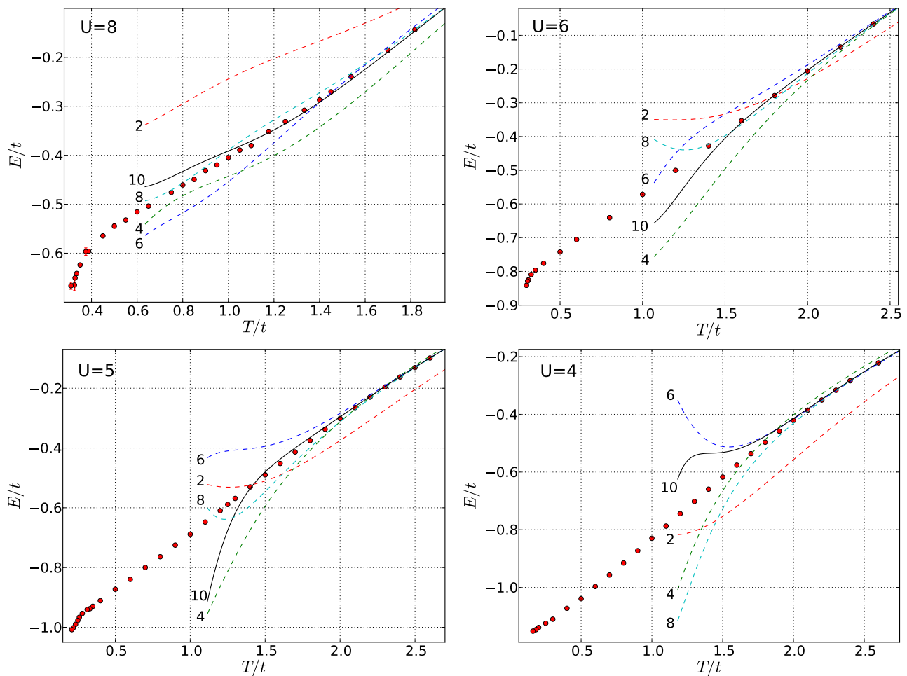
FIG. 9. (Color online.) Energy (extrapolated to the TD limit) versus temperature at U = 8, 6, 5, 4 . The lines represent the results of the high-temperature series expansion series of orders 2, 4, 6, 8, 10 labeled correspondingly.
