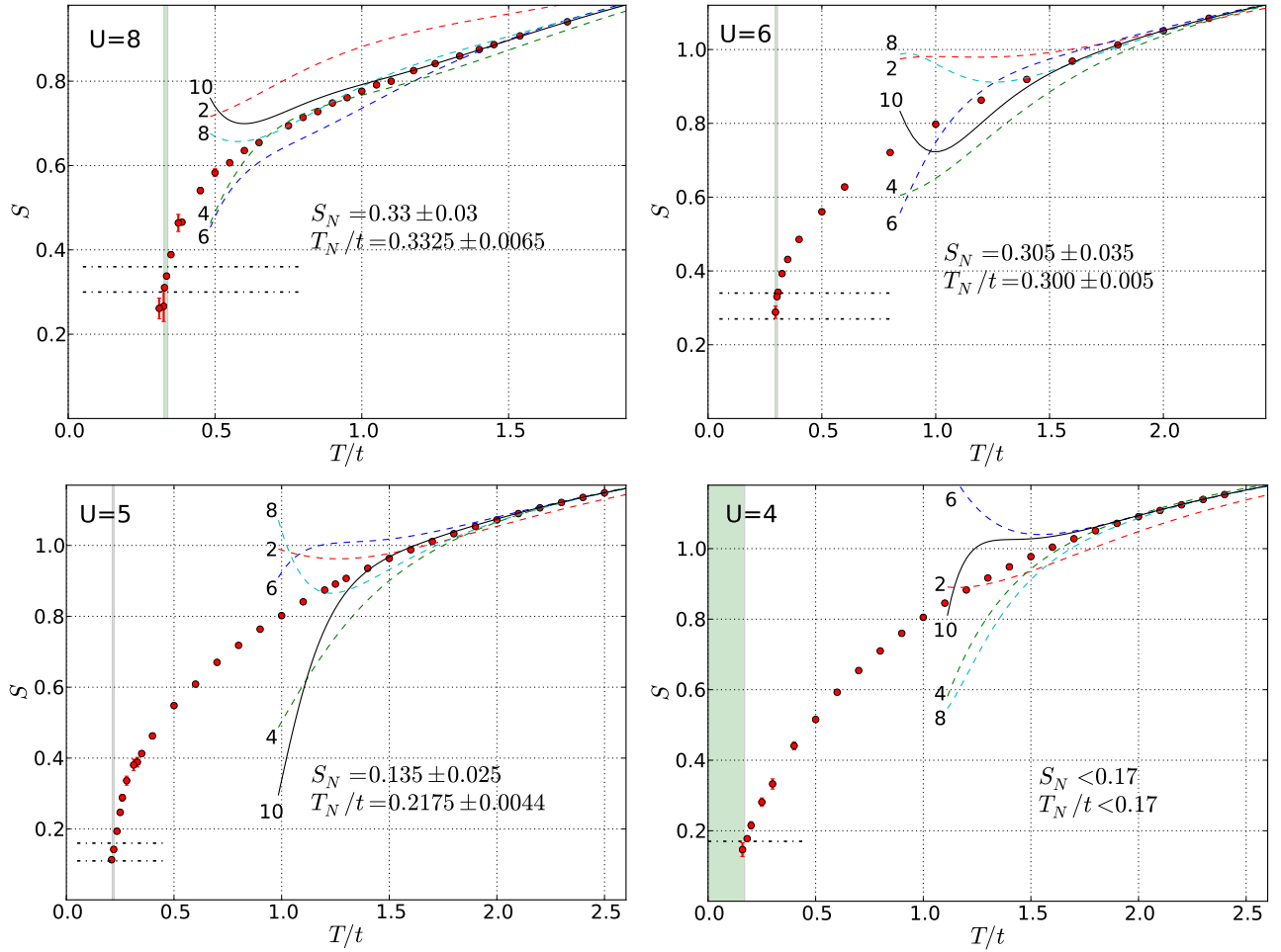
FIG. 10. (Color online.) Entropy (extrapolated to the TD limit) versus temperature at U = 8, 6, 5, 4 . In each panel, the vertical line shows the position of the critical temperature T_N with its width given by the error bar, while the horizontal dashed lines represent the corresponding bounds of the critical entropy S_N listed in Table I. The rest of the lines represent the results of the high-temperature series expansion series of orders 2, 4, 6, 8, 10 labeled correspondingly.
