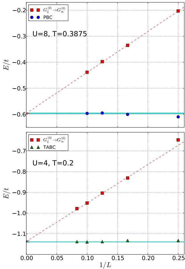
FIG. 8. (Color online.) Example of the dependence of energy on the inverse of the linear system size L obtained with the periodic boundary conditions (PBC, circles) for U = 8 , T = 0.3875 and with the twist-averaged boundary conditions (TABC, triangles) for U = 4 , T = 0.2 compared to the result of a simulation based on free-particle propagators of an infinite system ( G_L^{(0)} \rightarrow G_\infty^{(0)} , squares). The error bars are smaller than the symbols. The dashed line is a linear fit yielding E''(\infty) = -0.5962(9) ( E'(\infty) = -1.1368(32) ) in perfect agreement with the claimed conservative estimate E(\infty) = -0.5960(16) ( E(\infty) = -1.1390(9) ) for U = 8 , T = 0.3875 ( U = 4 , T = 0.2 ) shown by the horizontal band. The data point for the smallest system size L = 4 at U = 4 , T = 0.2 obtained with G_L^{(0)} \rightarrow G_\infty^{(0)} deviates from the linear scaling followed by larger systems and therefore is excluded from the fit.
