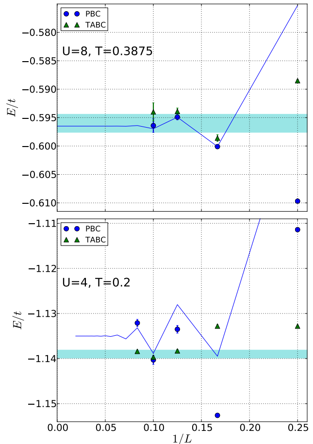
FIG. 7. (Color online.) Example of the dependence of energy on the inverse of the linear system size L obtained with the periodic boundary conditions (PBC, circles) and using the twist-averaged boundary conditions (TABC, triangles) for U = 8, T = 0.3875 and U = 4, T = 0.2 . The solid line is an extrapolation using the formula E(L) = E'(\infty) + C[E_0(L) - E_0(\infty)] (see text). For U = 8, T = 0.3875 the parameters are E'(\infty) = -0.5965, C = 0.6 , while for U = 4, T = 0.2 , E'(\infty) = -1.135, C = 0.95 . The claimed thermodynamic-limit results— E(\infty) = -0.5960(16) for U = 8, T = 0.3875 (using the PBC data) and E(\infty) = -1.1390(9) for U = 4, T = 0.2 (using the TABC data)—are shown by the horizontal bands. More generally, we use PBC data at U \geq 6 and TABC data at U \leq 5 to obtain the thermodynamic-limit values, as explained in Subsection. IV A.
