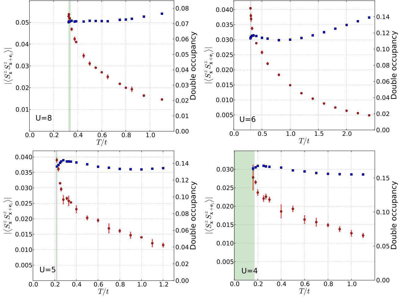
FIG. 12. (Color online.) Double occupancy \langle n_{x\uparrow} n_{x\downarrow} \rangle (squares) and the nearest-neighbor spin correlation function |\langle S_x^z S_{x+e_i}^z \rangle| (circles) versus T at U = 8, 6, 5, 4 extrapolated to the TD limit. In each panel, the vertical line shows the position of the critical temperature for a given value of U listed in Table I with its width corresponding to the error bar.
