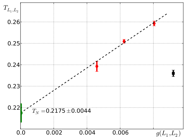
FIG. 3. (Color online.) Scaling—according to Eqs. (25)–(26)—of estimates of the critical temperature at U = 5t obtained from Binder crossings between lines for different system sizes in Fig. 2. See text for discussion. The square corresponds to the crossing point between lines for L = 4 and L = 10 , which substantially deviates from the linear scaling exhibited by all the crossings for L > 4 (circles), demonstrating that the L = 4 system is too small to be consistent with the critical scaling described by Eq. (24). Correspondingly, all the other crossings with the L = 4 line are omitted from the figure.
