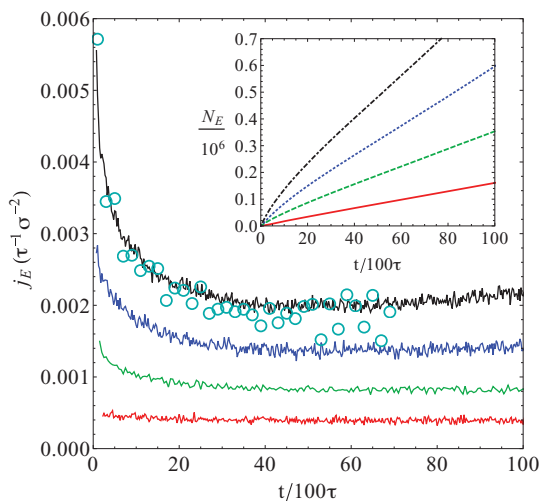
FIG. 8. Evaporation rate j_E vs. time for the LJ dimer system in contact with a vacuum at T_b = 0.9, 1.0, 1.1, and 1.2\epsilon/k_B (from bottom to top). The predicted evaporation flux j_m/m based on Eq. (9) is shown as circles. The inset shows the total number of removed atoms N_E vs. time.
