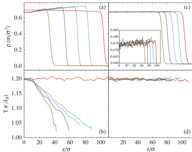
FIG. 7. Density [(a) and (c)] and temperature [(b) and (d)] for the LJ dimer fluid at T_b = 1.2\epsilon/k_B in contact with a vacuum [(a) and (b)] or evaporating at a controlled rate j_E = 5.0 \times 10^{-5} \tau^{-1} \sigma^{-2} [(c) and (d)]. From right to left the profiles are plotted every 5000\tau [(a) and (b)] and 100000\tau [(c) and (d)] since the evaporation process was started at t = 0 (the rightmost curve). The inset in (c) blows up the density profile in the liquid and interfacial region. Temperature in the vapor region is not included because the density of vapor is small and the data are too noisy to indicate a clear trend.
