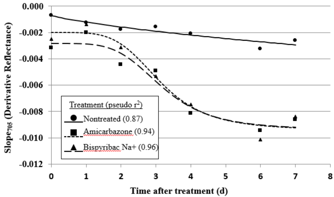
Figure 3. Herbicide treatment effect on first derivative spectral reflectance of annual bluegrass over time using slope between 705 and 730 nm.
