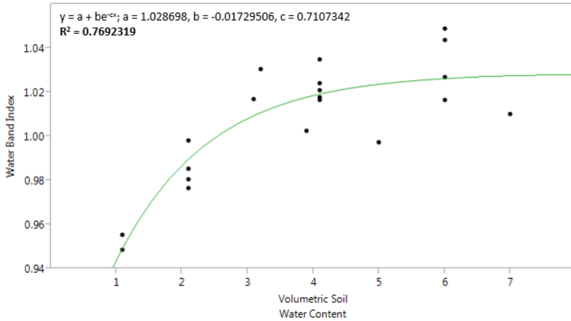
Figure 2. Three-parameter exponential nonlinear regression of water band index and soil water content from non-irrigated creeping bentgrass grown under greenhouse conditions in Blacksburg, VA.
