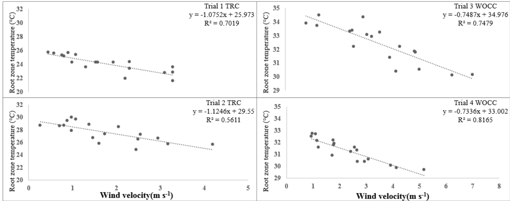
Figure 1. Linear relationship between wind velocity ( \text{m s}^{-1} ) and root zone temperature ( ^{\circ}\text{C} ) of creeping bentgrass putting greens for two trials for two location (left column TRC = Blacksburg, VA; right column WOCC = Richmond, VA).
