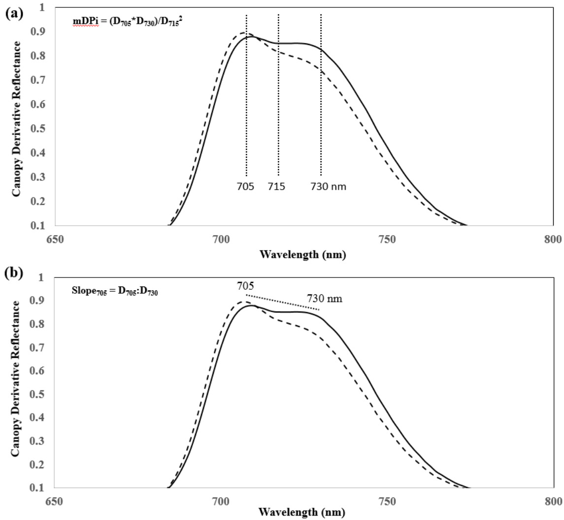
Figure 2. Double-peak spectral feature of derivative reflectance collected from healthy (solid line) and herbicide-stressed (broken line) annual bluegrass using a field radiometer in the 705-730 nm spectral range. A modified double-peak index (mDPi) was calculated using derivative reflectance bands 705, 715, and 730 nm (a) and slope of derivative spectra between 705 and 730 nm (b).
