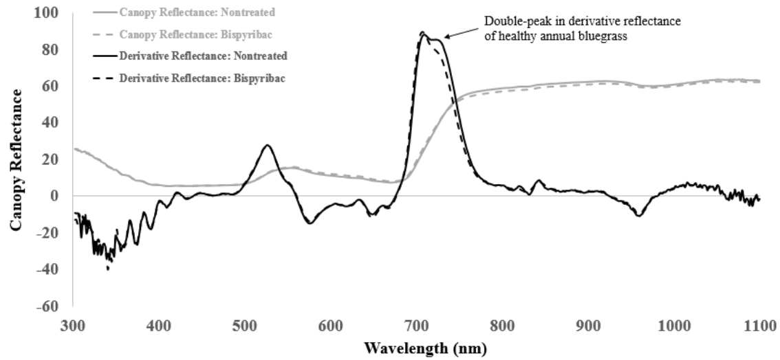
Figure 1. Canopy reflectance (gray line) and derivative reflectance (black line) collected from healthy, nontreated (solid) and bispyribac-treated (broken) annual bluegrass using a field radiometer over a spectral range of 300-1100 nm. Derivative spectra scaled up (*100).
