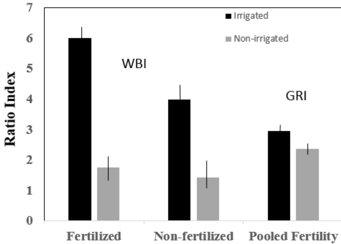
Figure 1. Treatment means for the effect of irrigation on the water band index ( WBI = R_{900}/R_{970} * 100 ) and the green/red ratio index ( GRI = R_{550}/R_{670} ) pooled over creeping bentgrass trials conducted under greenhouse conditions in Blacksburg, VA.
