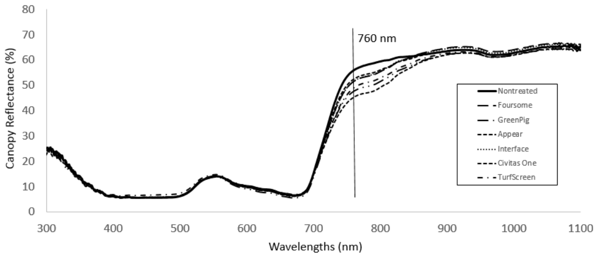
Figure 2. Percent canopy reflectance of six commercially available synthetic phthalocyanine pigment-containing products 24 hours after application to 'L-93' creeping bentgrass fairways at the Glade Road Research Facility, Blacksburg, VA.
