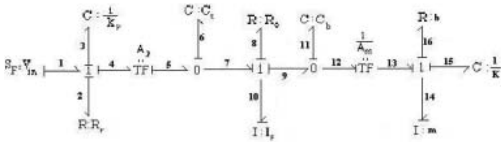
Fig. 5. Bond Graph Model of Fig. 4.
