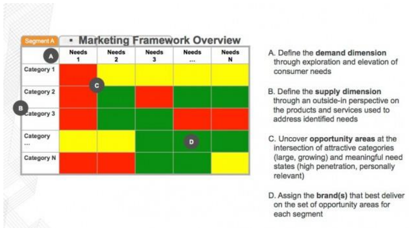
Figure 1: Segmentation Approach
