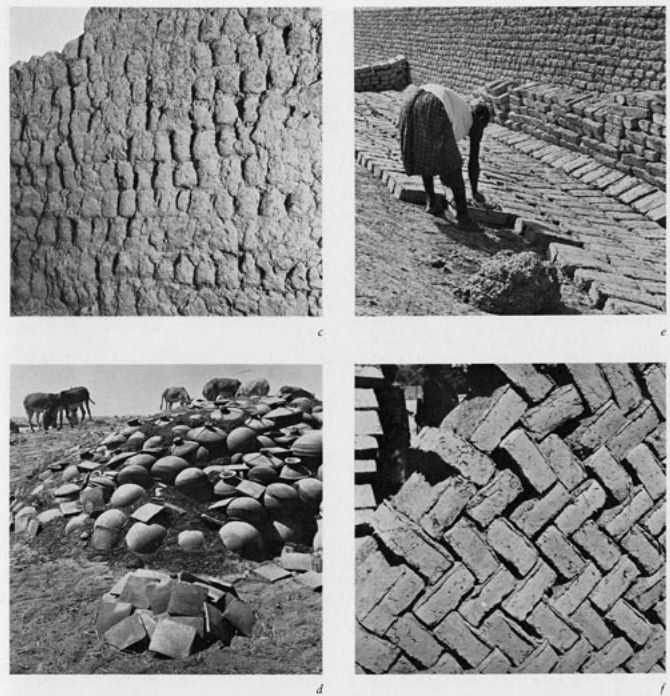
Examples of the techniques of earthen construction used by the women of Djenné, Mali, including cylindrical sun-dried bricks and kiln-fired pottery and paving bricks. Photo from Hatumere: Islamic Design in West Africa by Dr. Labelle Prussin, 1986.
