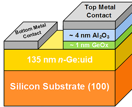
FIG. 7. Ge-on-Si MOS capacitor structure.
