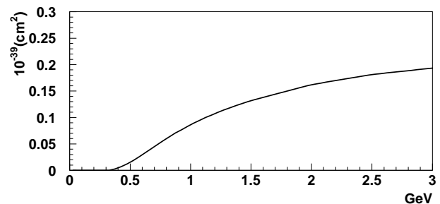
FIG. 2. Cross section versus neutrino energy of NC single \pi^0 production per nucleon on a polystyrene target ( C_8H_8 ) estimated in NEUT; the curve is based on the Rein and Sehgal model.
