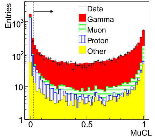
FIG. 9. The muon confidence level (MuCL) of tracks after the EC cut. The contributions from true gamma ray, muon, and proton tracks are shown separately for the MC simulation.
