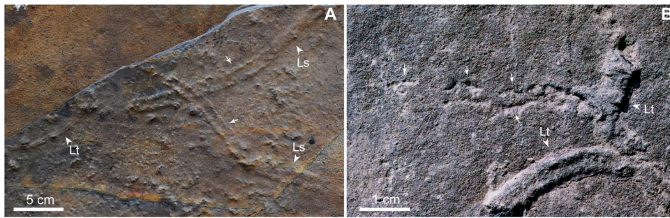
Fig. 5. Possible trackways associated with trace fossils of the genus Lamonte from the Shibantan Member. (A) Positive hyporelief from the same bedding surface where trackways illustrated in Fig. 2 were found. Two species are recognized on the basis of size: L. trevallisi (labeled as Lt) is narrower than Lamonte sp. (labeled as Ls). Note that Lamonte sp. consists of possible trackways (arrows; with poorly preserved imprints) transitioning into burrows (arrowheads). NIGP-166149 (catalog number for the entire slab). (B) L. trevallisi from a different stratigraphic horizon of the Shibantan Member. Note burrows (arrowheads) and possible tracks (arrows) preserved as positive and negative epireliefs, respectively. Also illustrated in the study of Chen et al. (13). NIGP-154193. Figure produced by Z.C. and S.X. using Adobe Photoshop.
