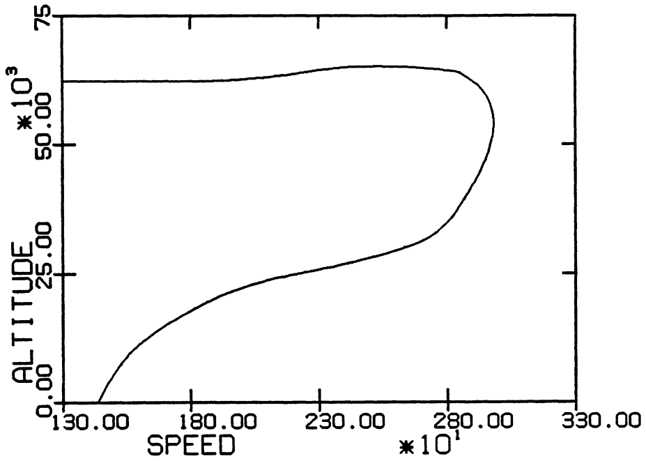
Fig 7.....Unlimited Flight Envelope, Smooth Data
