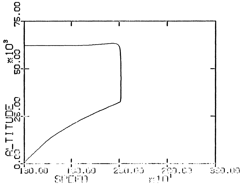
Fig 9.....Envelope with q and Mach Limits
