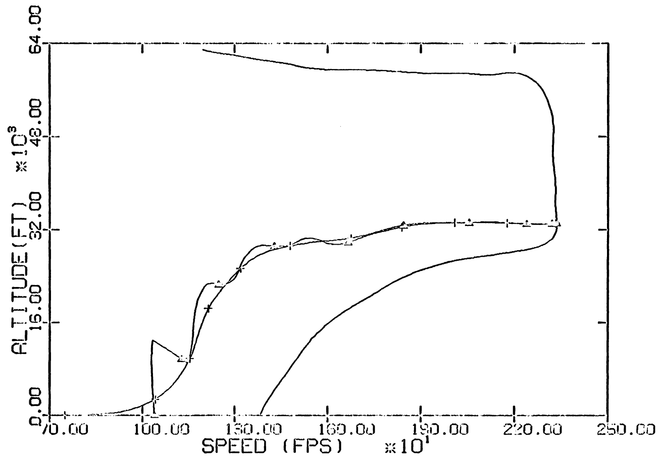
Fig 27.....Range-Energy-Climb and Point Mass Solution
