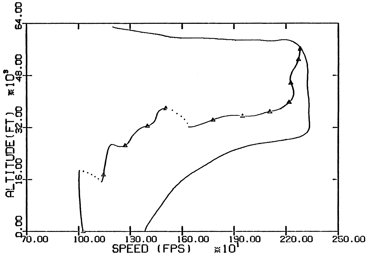
Fig 1.....Energy Climb Schedule on h-v plane
