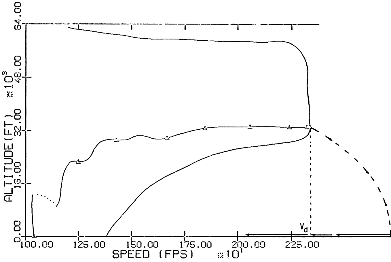
Fig 3.....Terminal Energy Transient
