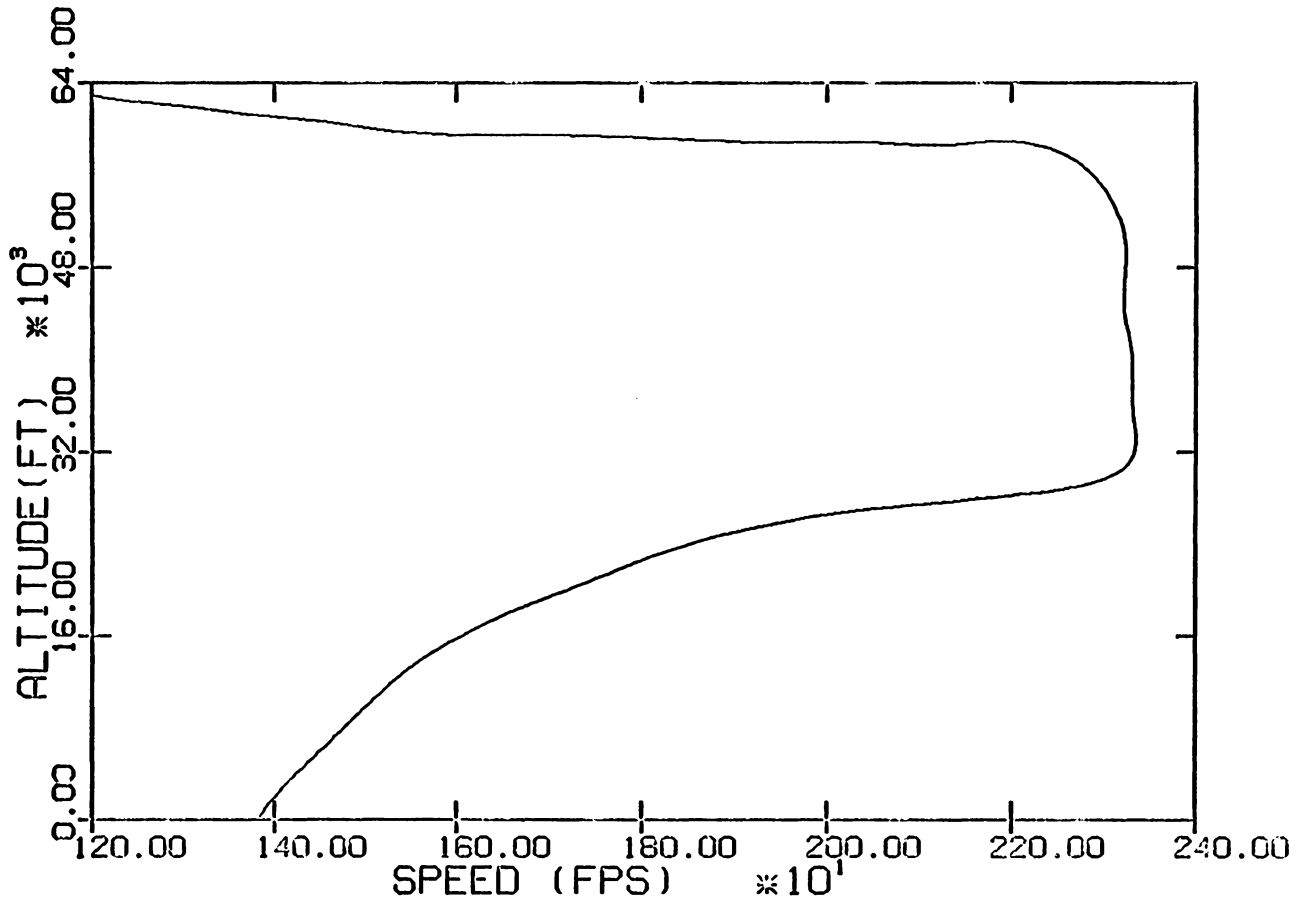
Fig 15.....Flight Envelope Spline Data
