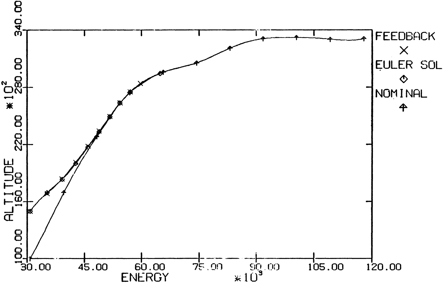
Fig 42.....Altitude vs Energy, 5000 ft above
