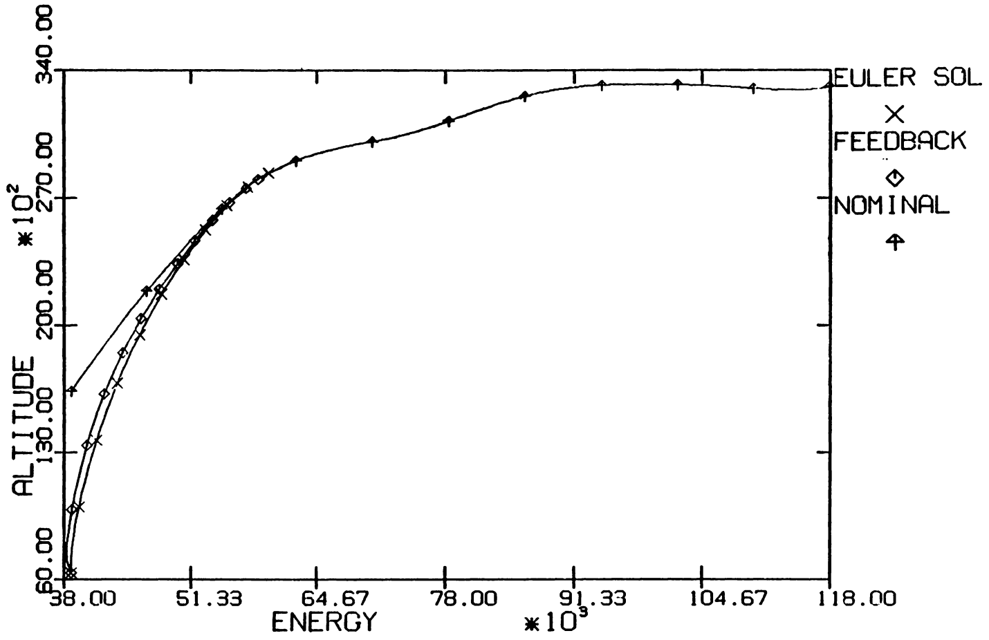
Fig 46.....Altitude vs Energy, 10000 ft below
