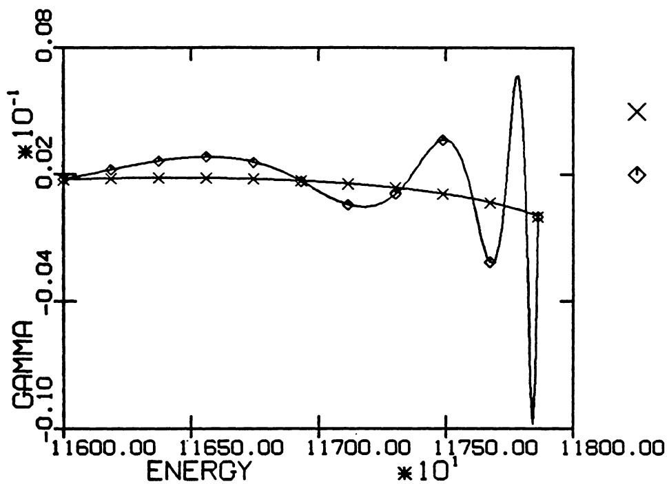
Fig 23.....Path-Angle vs Energy 300,360 seconds
