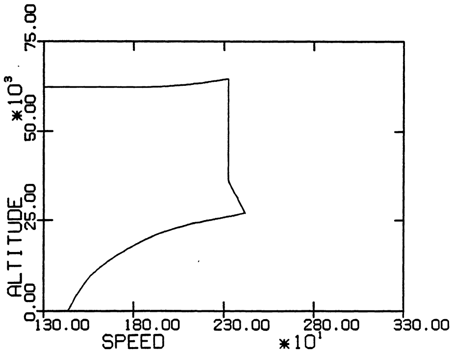
Fig 8.....Envelope with Mach Limit, Smooth Data
