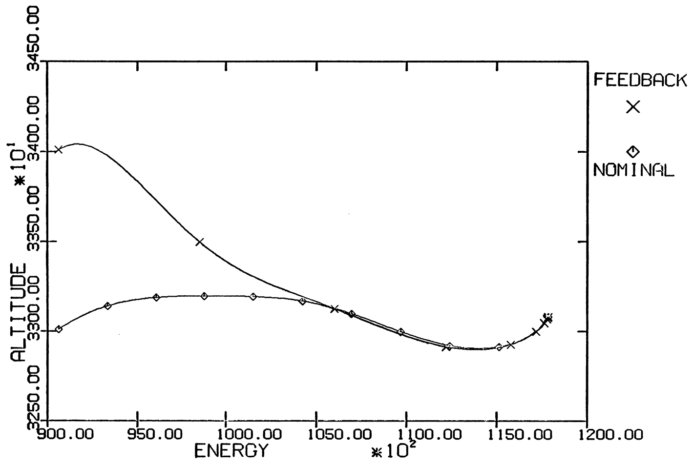
Fig 40.....Altitude vs Energy, 1000 ft above
