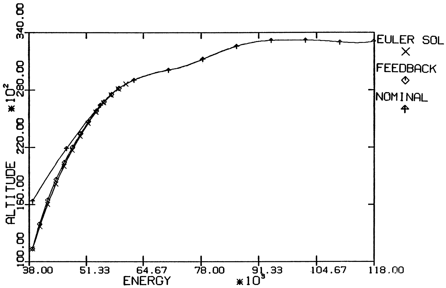
Fig 45.....Altitude vs Energy, 5000 Ft below
