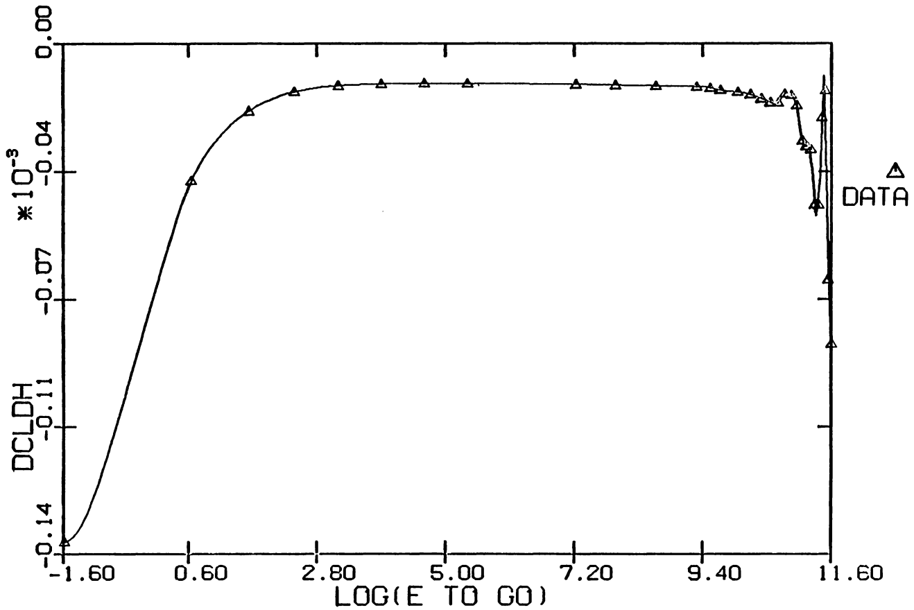
Fig 38.....Altitude Gain vs Log(E)
