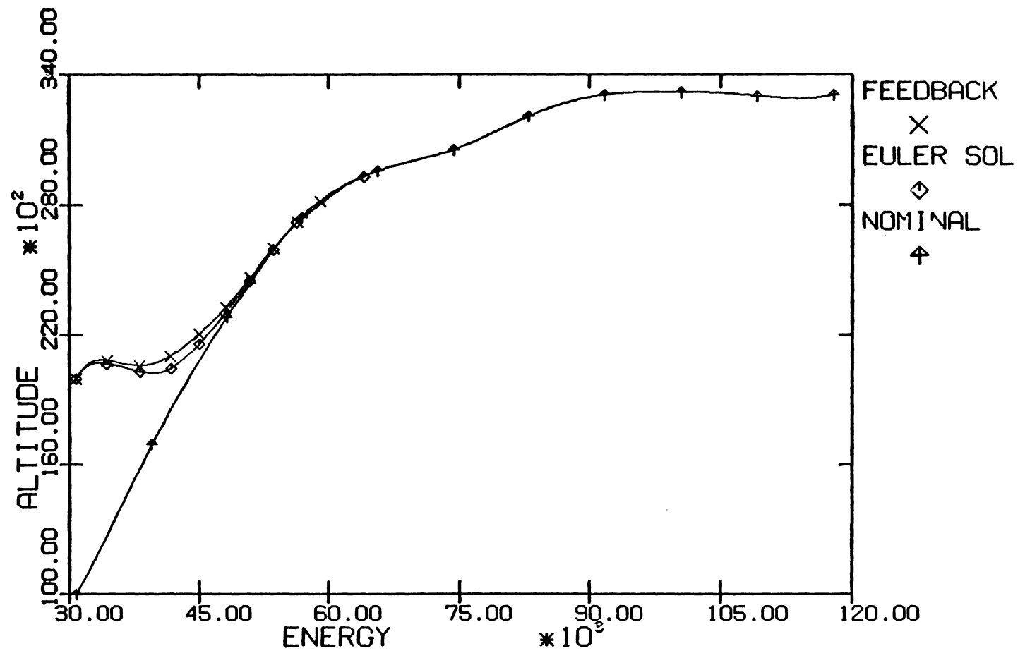
Fig 43.....Altitude vs Energy, 10000 ft above
