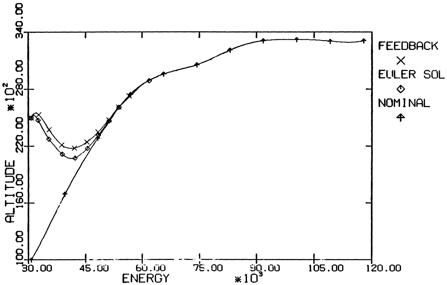
Fig 44.....Altitude vs Energy, 15000 ft above
