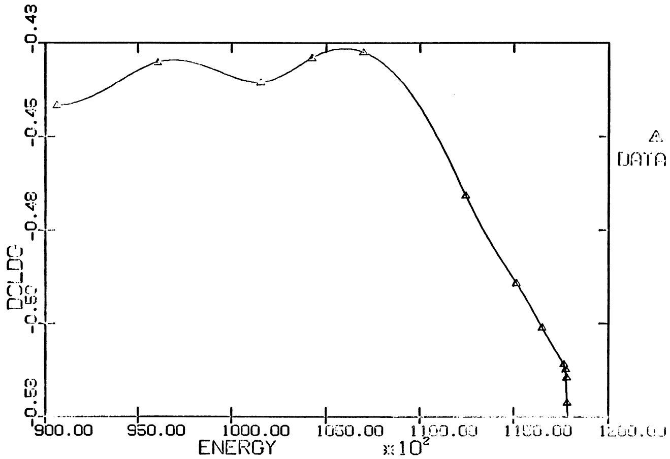
Fig 33.....Path-Angle Gain vs Energy
