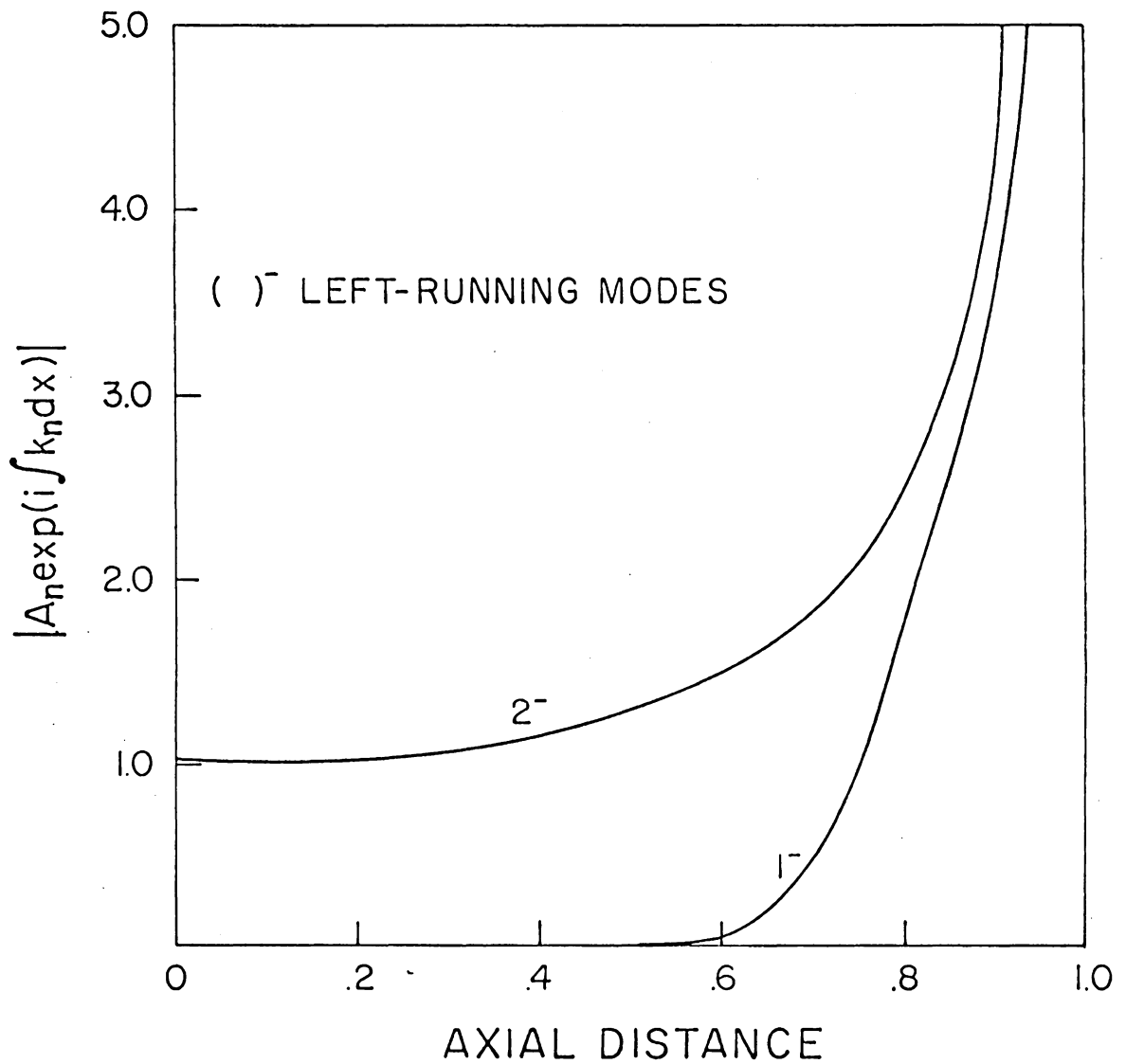
Figure 6. The absolute value of the left-running modes, \omega = 7 , \delta = 0.06 , maximum wall slope = 0.37, L = 2 , throat Mach number 0.95, lined wall.
