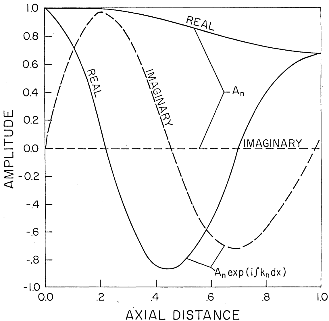
Figure 3. Comparison between the slowly varying functions A_n and A_n \exp(isk_n dx) , \omega = 10 , \delta = 0.06 , maximum wall slope = 0.37, L = 2 , throat Mach number = 0.6, lined wall.
