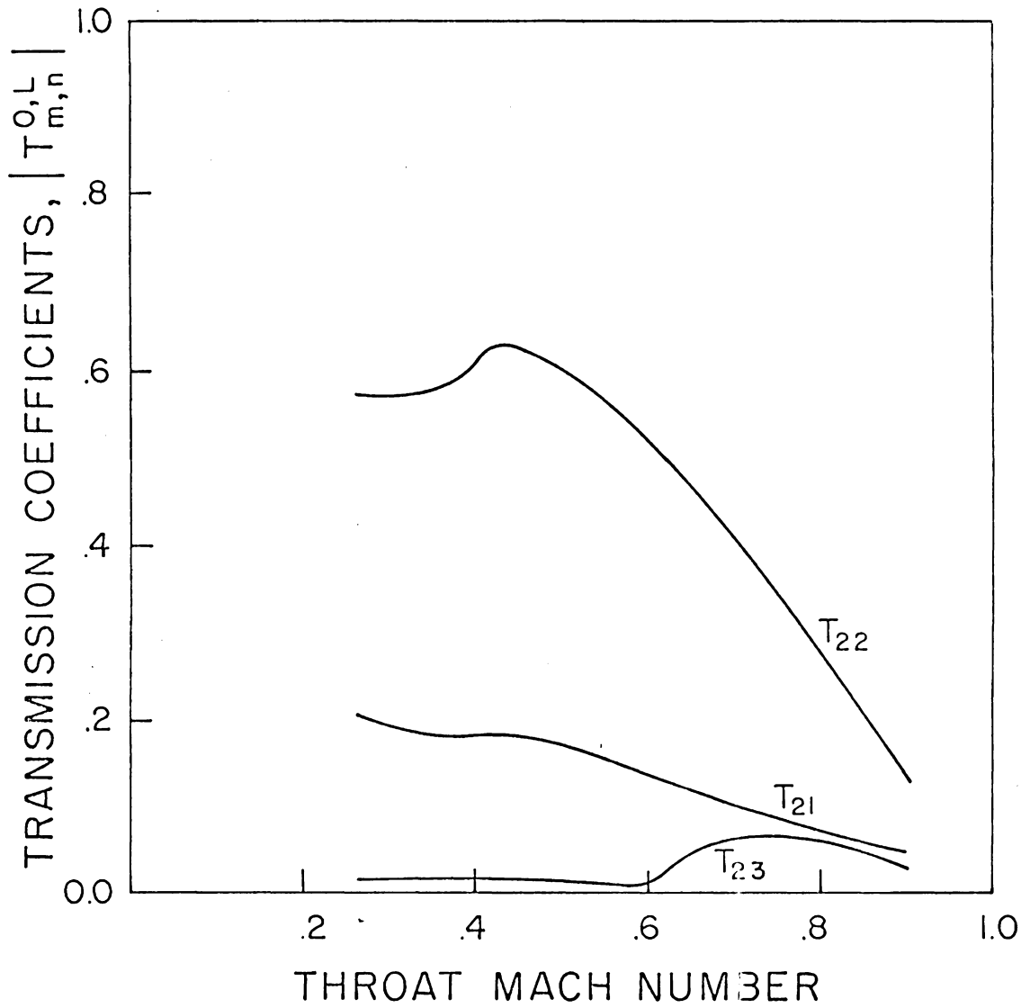
Figure 12. Effect of the throat Mach number on the absolute value of the transmission coefficients at x = 0 , due to exciting the second mode only, \omega = 10 , \delta = 0.06 , maximum wall slope = 0.37, L = 2 , lined wall.
