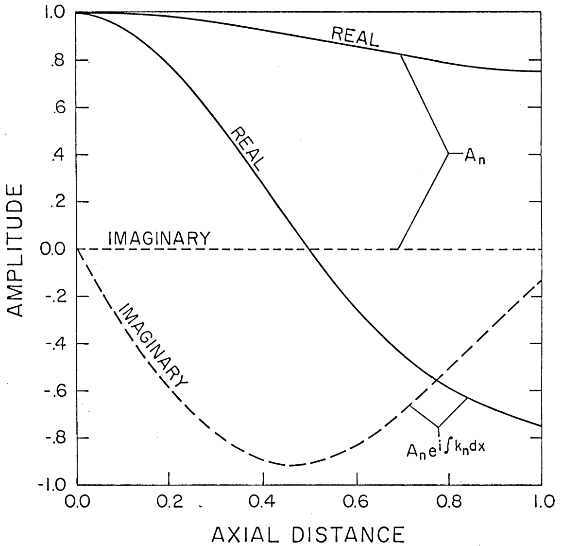
Figure 2. Comparison between the slowly varying functions A_n and A_n \exp(i \int k_n dx) , \omega = 4 , \delta = 0.06 , maximum wall slope = 0.37, L = 2 , throat Mach number = 0.6, lined wall.
