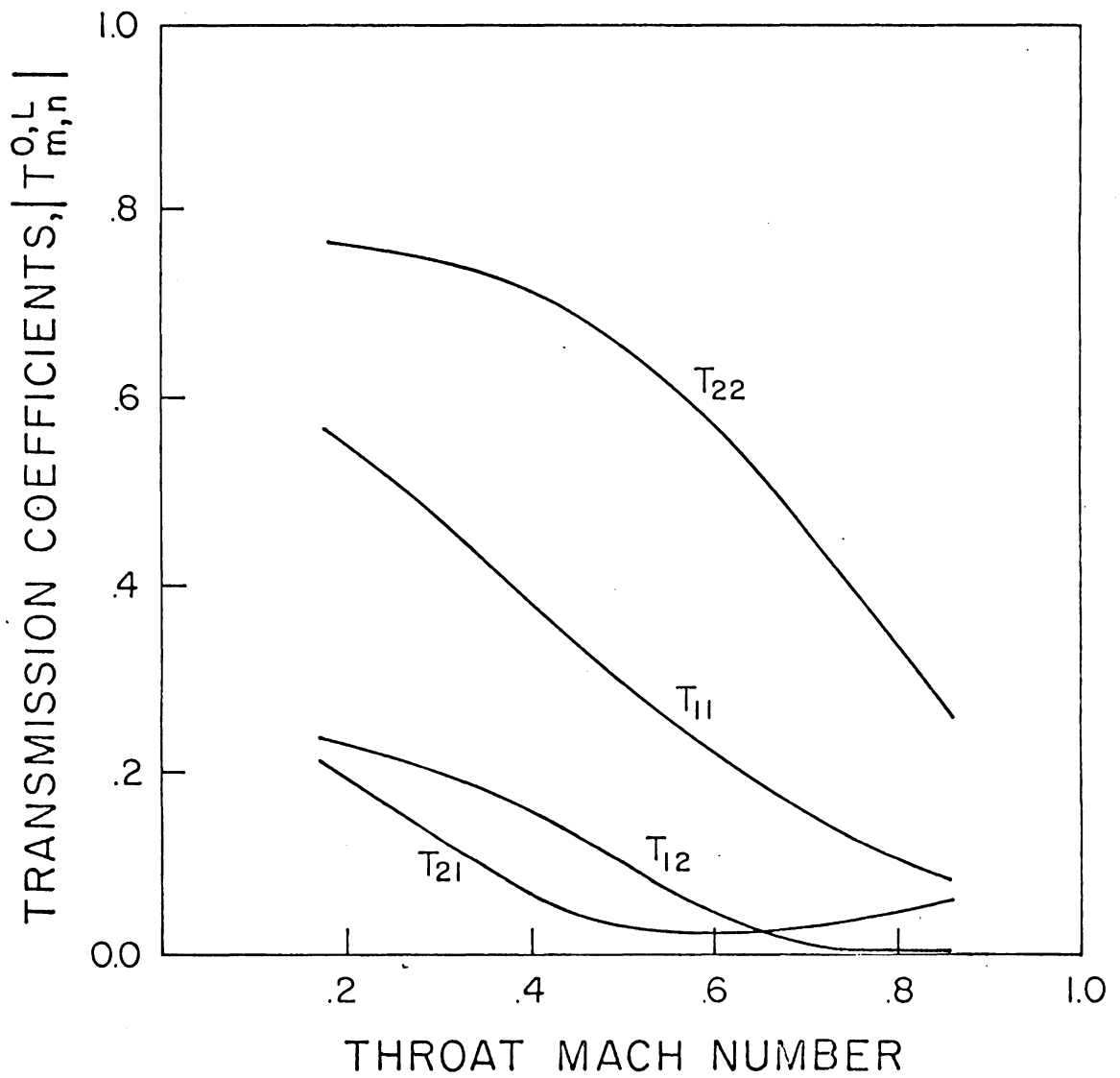
Figure 8. Effect of the throat Mach number on the absolute value of the transmission coefficients at x = 0 , \omega = 7 , \delta = 0.06 , maximum wall slope = 0.37, L = 2 , lined wall.
