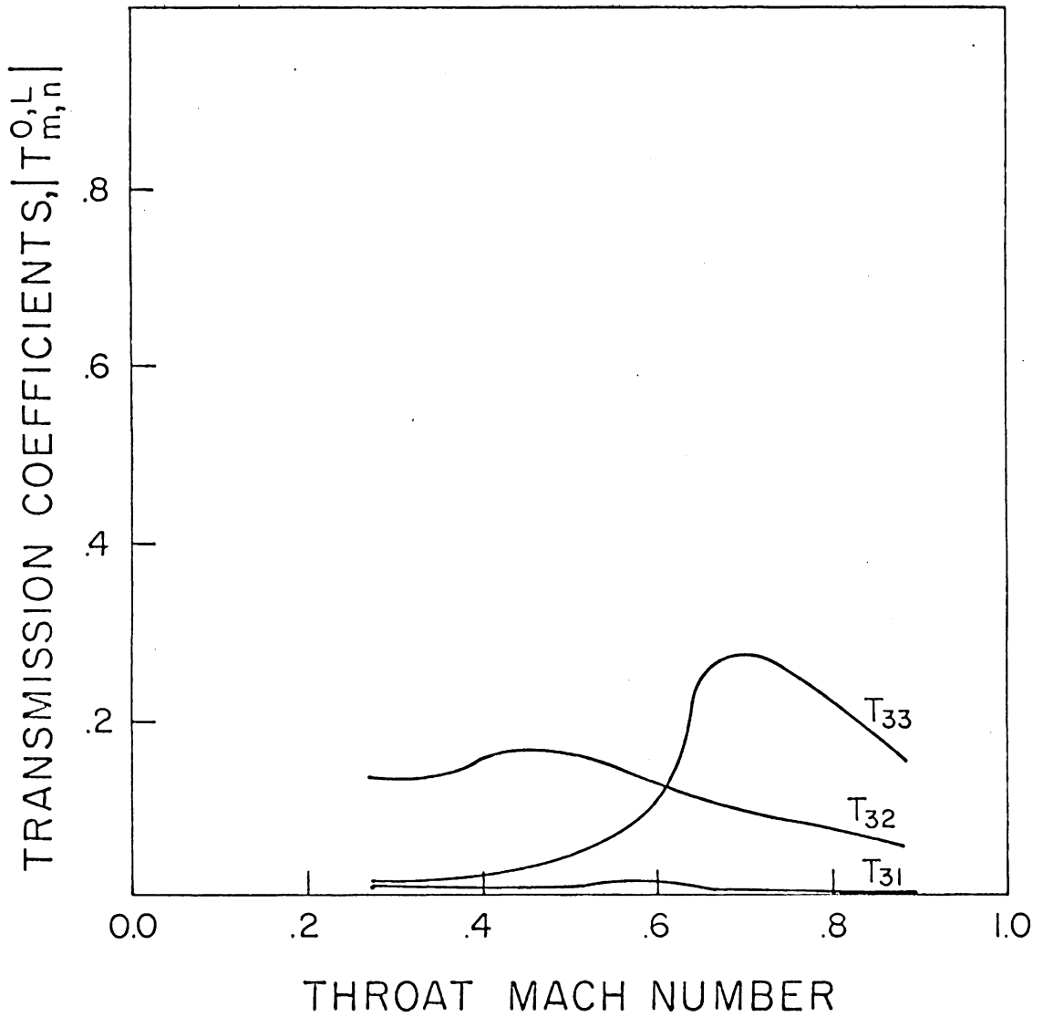
Figure 13. Effect of the throat Mach number on the absolute value of the transmission coefficients at x = 0 , due to exciting the third mode only, \omega = 10 , \delta = 0.06 , maximum wall slope = 0.37, L = 2 , lined wall.
