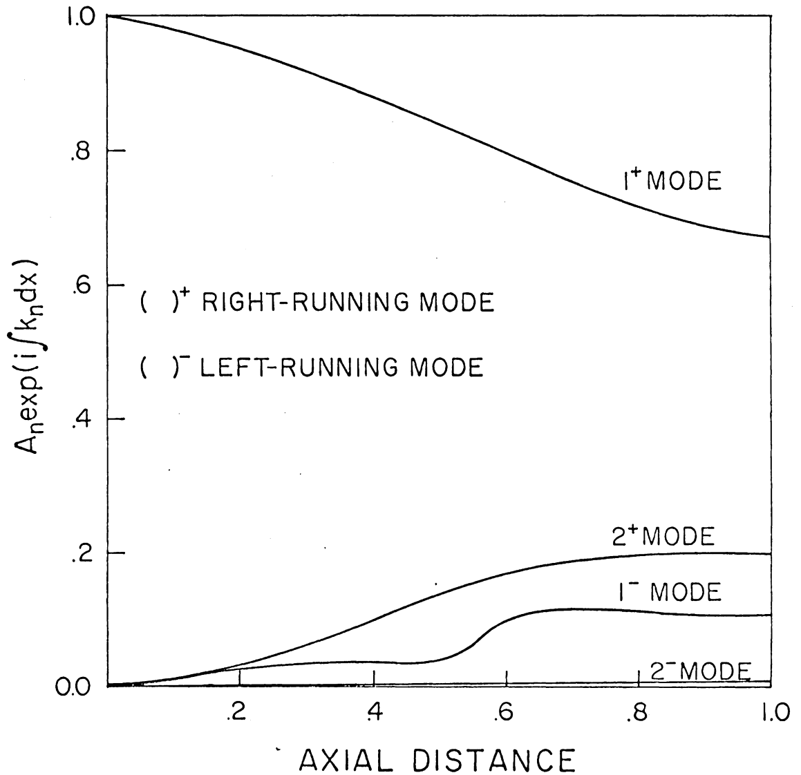
Figure 5. The absolute value of the amplitude for various modes when the first mode is excited, \omega = 7 , \delta = 0.06 , maximum wall slope = 0.37, L = 2 , throat Mach number = 0.6, lined wall.
