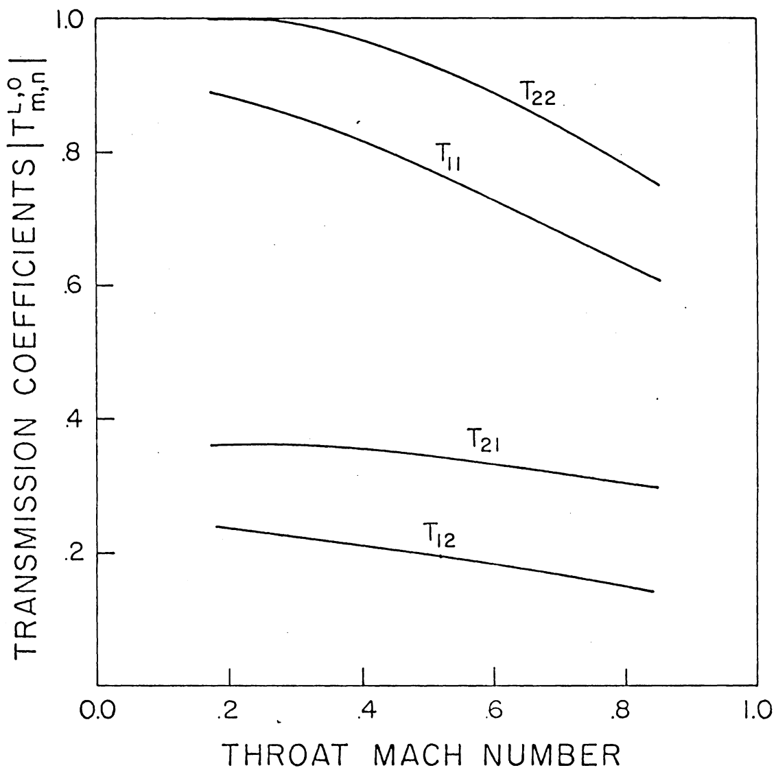
Figure 9. Effect of the throat Mach number on the absolute value of the transmission coefficients at x = L , \omega = 7 , \delta = 0.06 , maximum wall slope = 0.37, L = 2 , hard wall.
