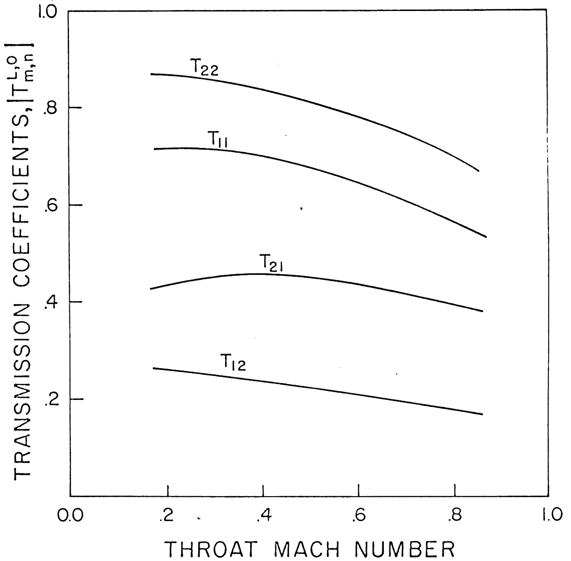
Figure 10. Effect of the throat Mach number on the absolute value of the transmission coefficients at x = L , \omega = 7 , \delta = 0.06 , maximum wall slope 0.37, L = 2 , lined wall.
