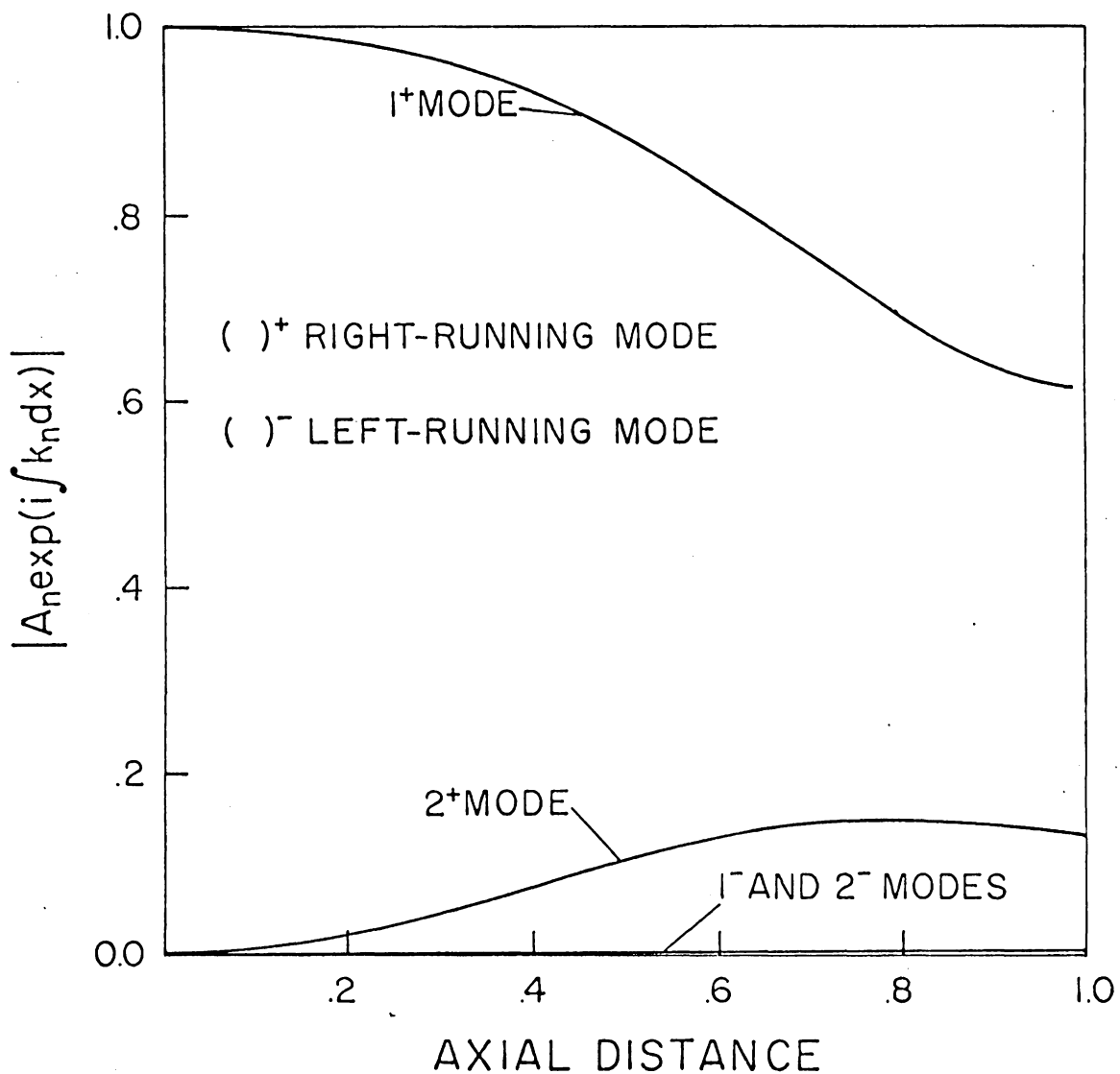
Figure 4. The absolute value of the amplitude for various modes when the first mode is excited, \omega = 7 , \delta = 0.06 , maximum wall slope = 0.37, L = 2 , throat Mach number = 0.86, hard wall.
