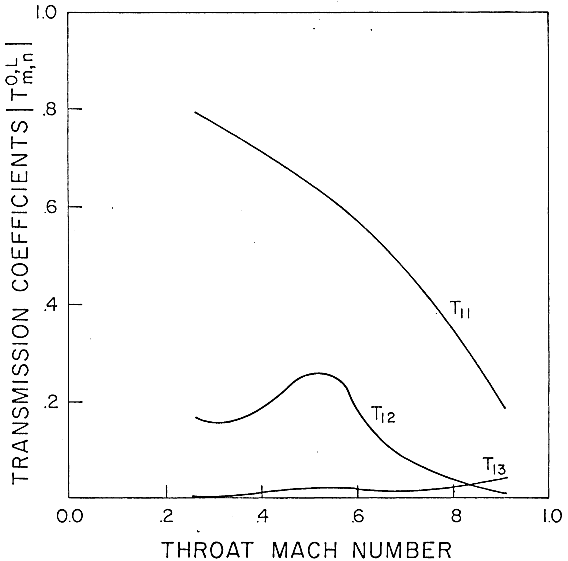
Figure 11. Effect of the throat Mach number on the absolute value of the transmission coefficients at x = 0 , due to exciting the first mode only, \omega = 10 , \delta = 0.06 , maximum wall slope = 0.37, L = 2 , lined wall.
