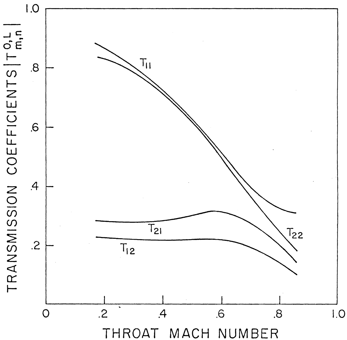
Figure 7. Effect of the throat Mach number on the absolute value of the transmission coefficients at x = 0 , \omega = 7 , \delta = 0.06 , maximum wall slope = 0.37, L = 2 , hard wall.
