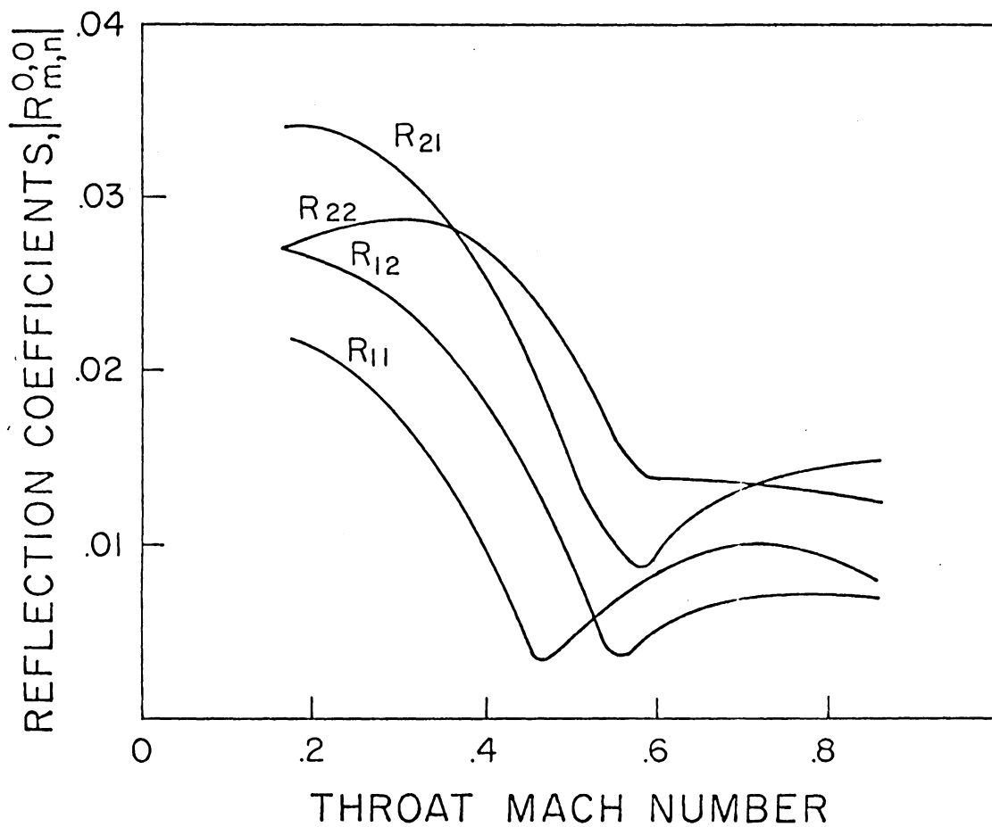
Figure 14. Effect of the throat Mach number on the absolute value of the reflection coefficients at x = 0 , \omega = 7 , \delta = 0.06 , maximum wall slope = 0.37, L = 2 , hard wall.
