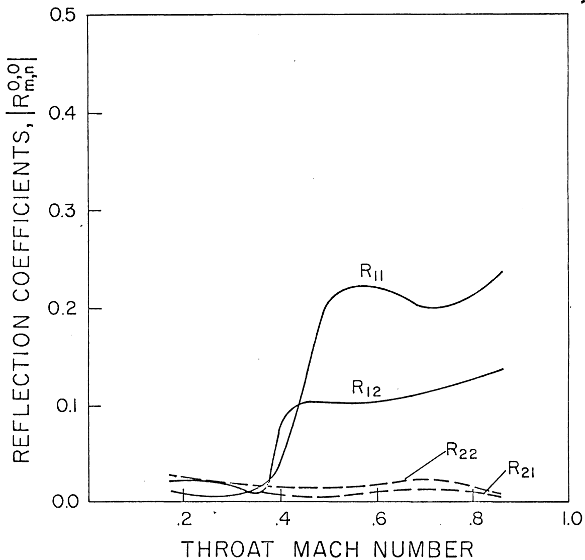
Figure 15. Effect of the throat Mach number on the absolute value of the reflection coefficients at x = 0 , \omega = 7 , \delta = 0.06 , maximum wall slope = 0.37, L = 2 , lined wall.
