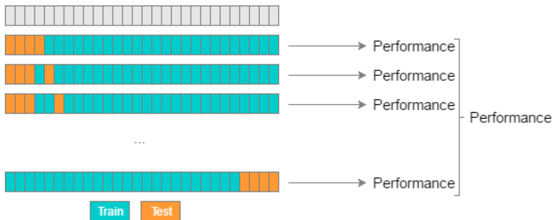
Fig. 1: Ref: http://www.ebc.cat/2017/01/31/cross-validation-strategies/
