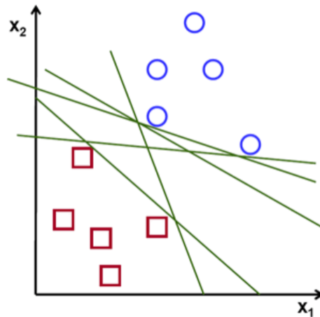
Fig. 1: Ref: https://towardsdatascience.com/support-vector-machine-introduction-to-machine-learning-algorithms-934a444fca47
