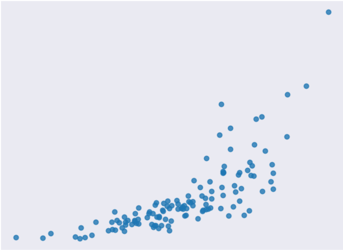
Fig. 5: Figure 4. A sample data set that follows an exponential curve [code]
