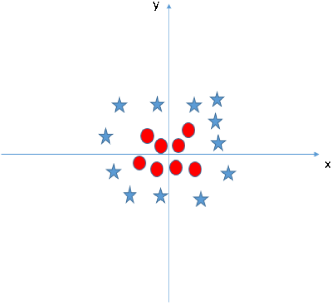
Fig. 4: Ref: https://www.analyticsvidhya.com/blog/2017/09/understaing-support-vector-machine-example-code/
