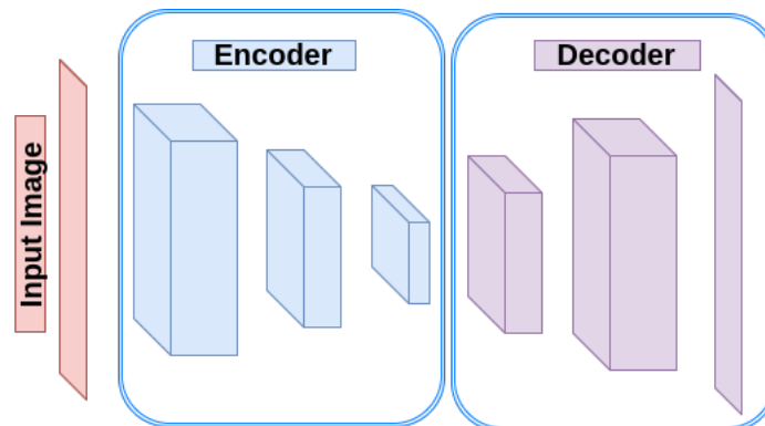
Fig. 1: Figure 1: Autoencoder
