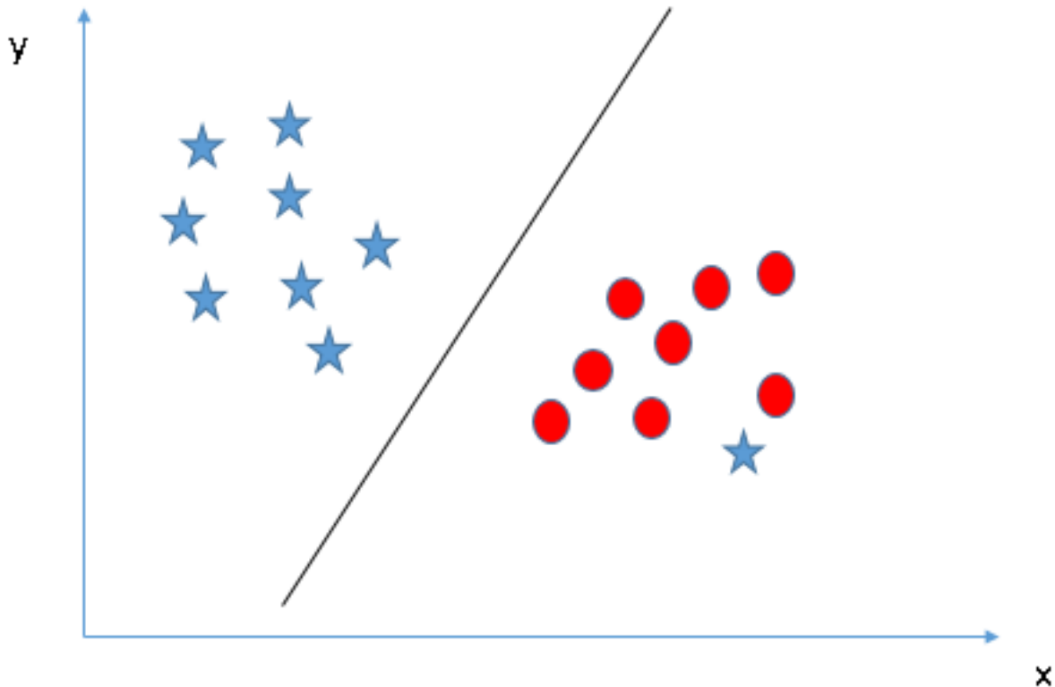
Fig. 3: Ref: https://www.analyticsvidhya.com/blog/2017/09/understaing-support-vector-machine-example-code/
