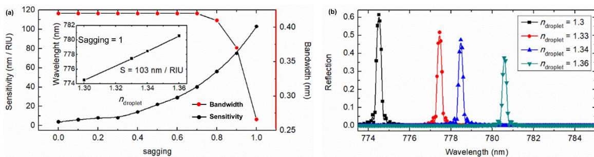
Figure 8. (a) Sensitivity and bandwidth dependence on sagging of the droplet. The inset shows the Bragg wavelength vs. n_{\text{droplet}} ; (b) Wavelength shift for the optofluidic filter system with sagging = 1.
