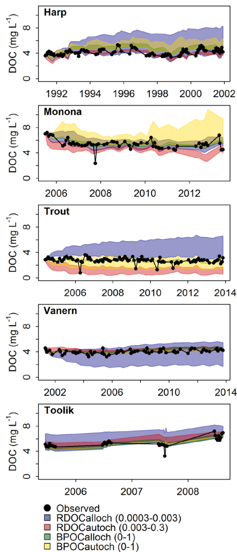
Fig. 3. Sensitivity of modeled dissolved organic carbon (DOC) concentrations to free parameters in the model. Each parameter was varied across a given range (RDOC Alloch 0.0003–0.003 d -1 , RDOC Autoch 0.003–0.3 d -1 , BPOC Alloch 0–1, BPOC Autoch 0–1) while the other three parameters remained fixed at their calibrated values. Shaded areas represent the range of modeled DOC concentrations as each parameter was varied. Black circles represent observed in-lake DOC concentrations.
