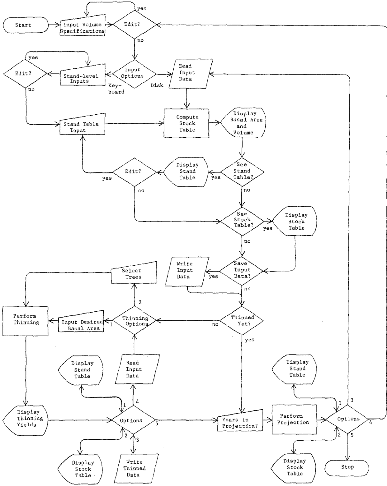
Figure 1. Generalized flow chart for BASIC G-HAT.
