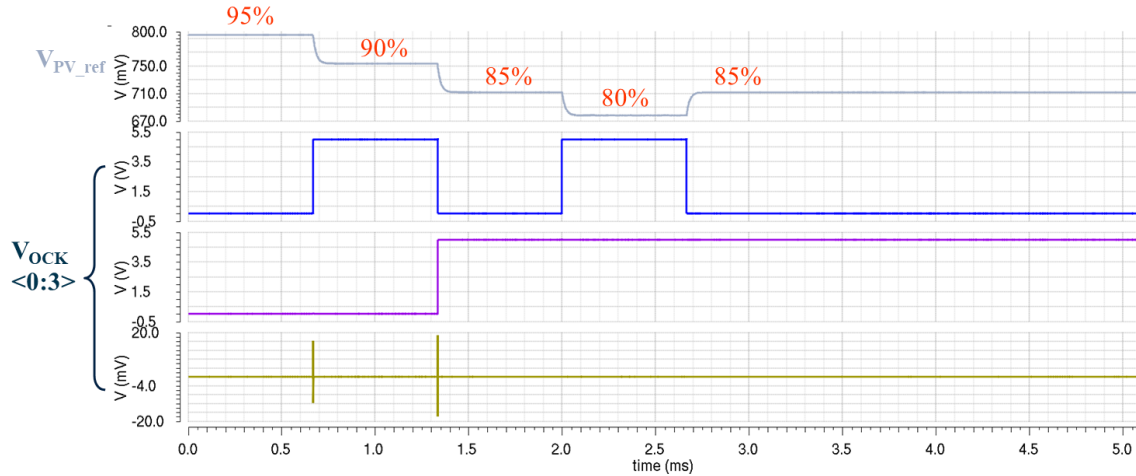
Figure 4.9 Reference perturbing
