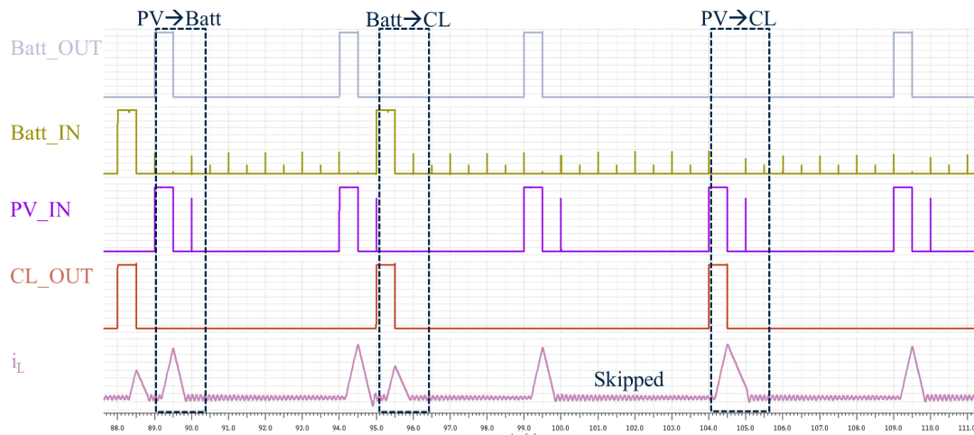
Figure 4.6 I/O Configuration under different combination cases
