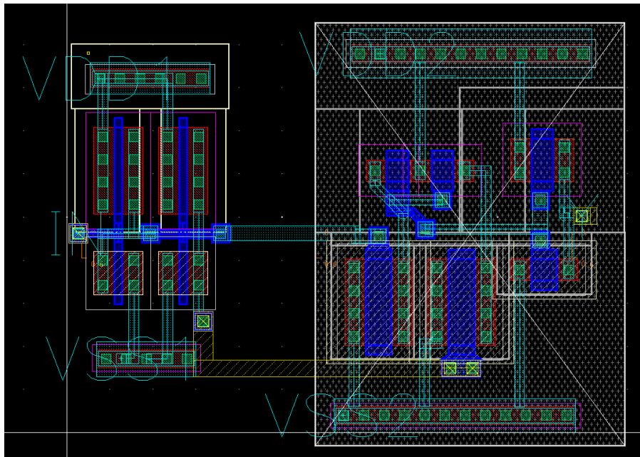
Figure B-10 Level Shifter
