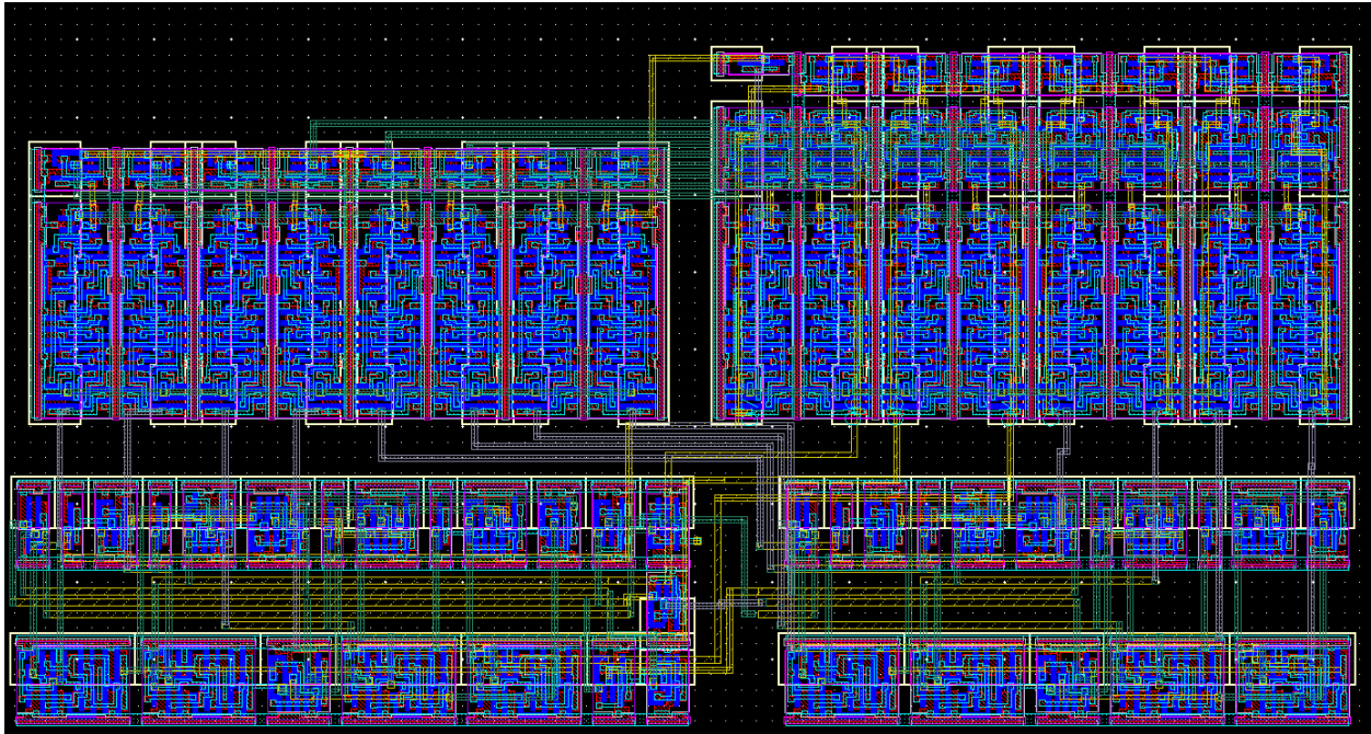
Figure B-1 8-bit Sample/Store/Comp Unit
