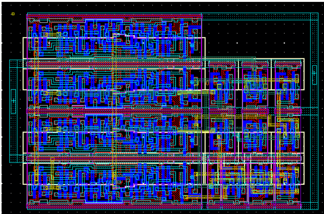
Figure B-6 4-bit Up/down Counter
