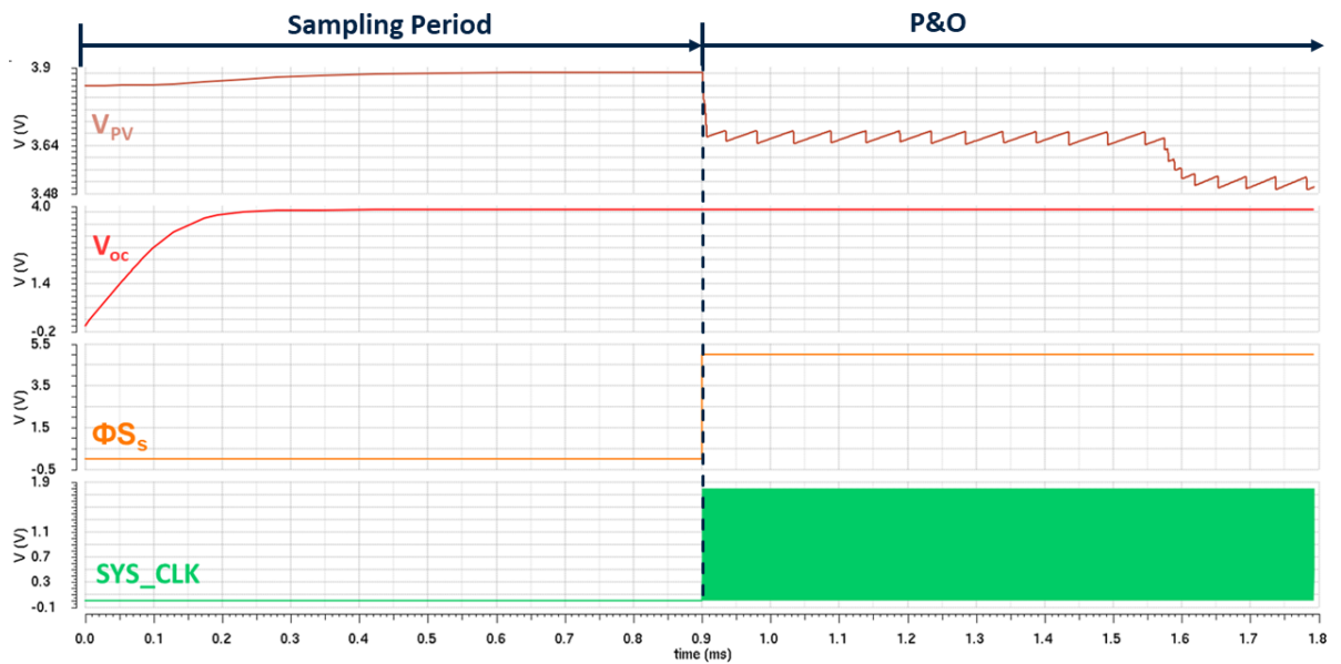
Figure 4.7 Open-voltage sampling process
