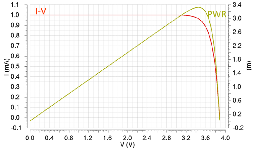
Figure 4.2 I-V characteristics and power curve of the solar panel used in this design
