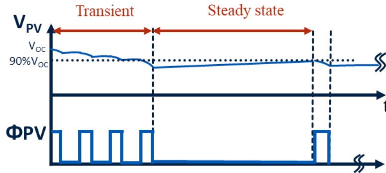
Figure 3.2 Pulse skipping modulation for PV
