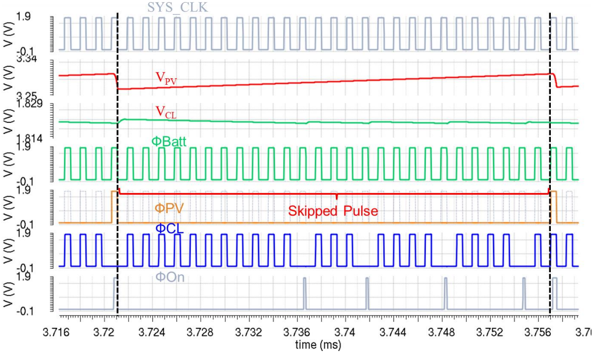
Figure 4.4 Pulse skipping Modulation Waveforms
