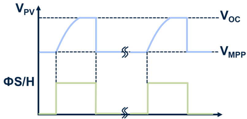
Figure 3.12 Sampling behavior waveform
