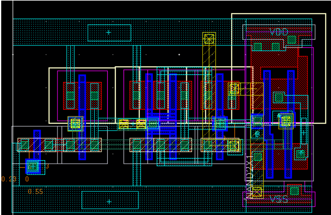
Figure B-7 On-time Generation Block
