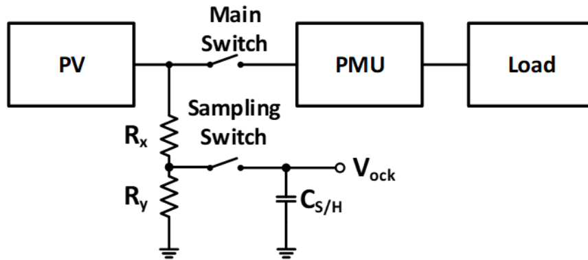
Figure 2.6 Common FOCV structure
