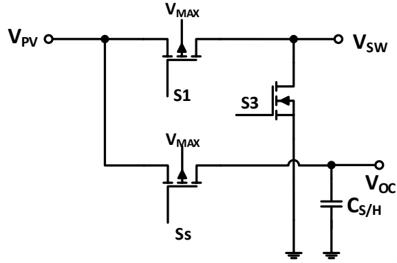
Figure 3.6 Open-circuit voltage sampling
