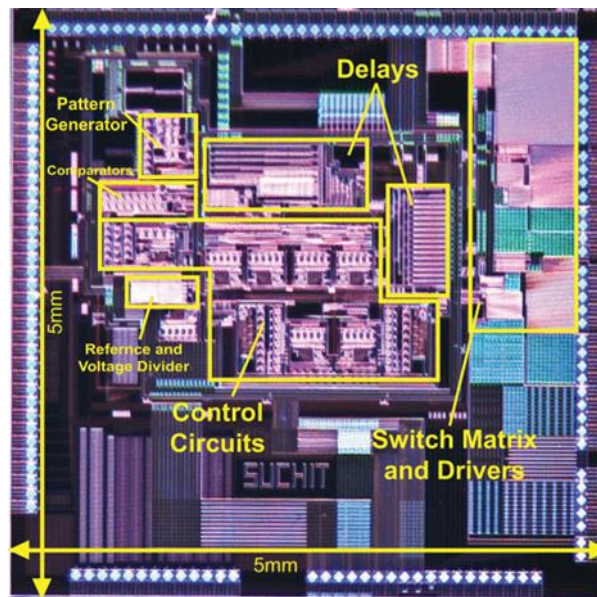
Figure 2.9 Die photo of the first previous work [17]
