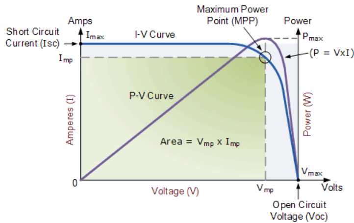
Figure 2.2 PV panel IV characteristics
