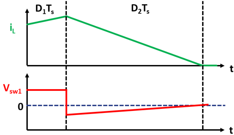
Figure 3.3 V_{sw1} and i_L waveform when zero current switching occurs
