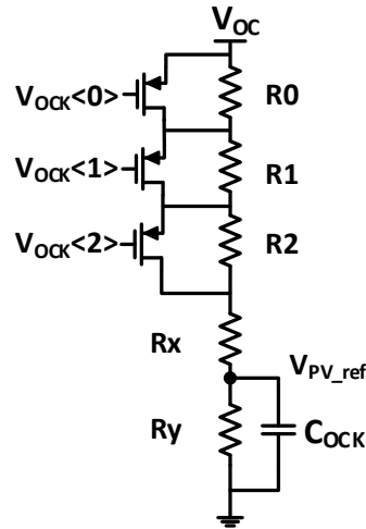
Figure 3.7 3-bit digital controlled reference ladder to setup perturb region
