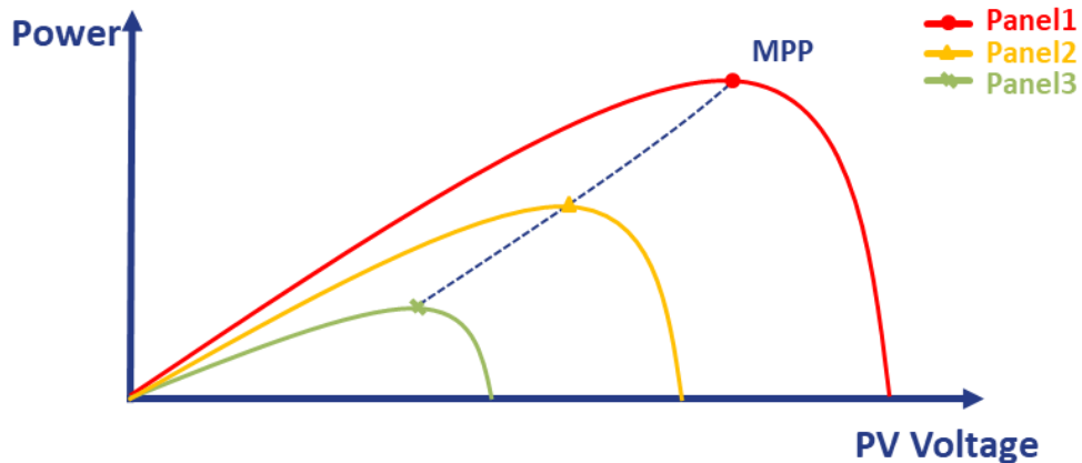
Figure 2.4 Different PV panel I-V characteristics under the same light condition
