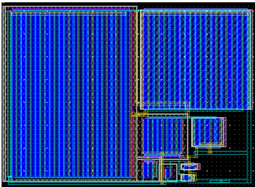
Figure B-12 Gate Driver
