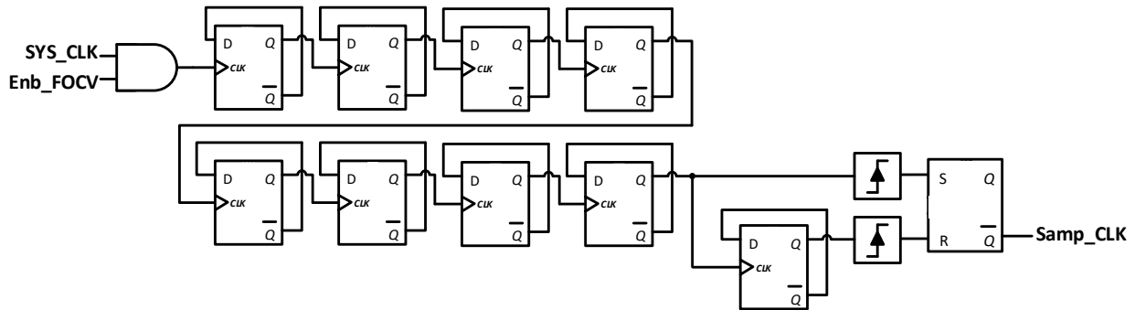
Figure 3.9 Sampling CLK signal generation
