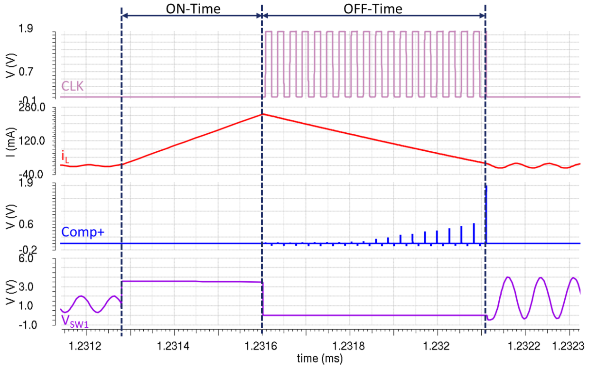
Figure 4.3 Zero current detection waveforms
