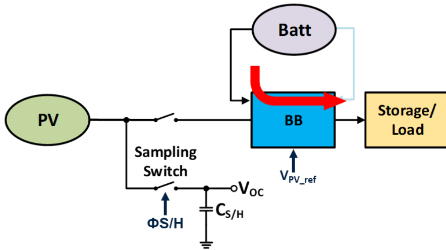
Figure 3.11 FOCV mode block diagram
