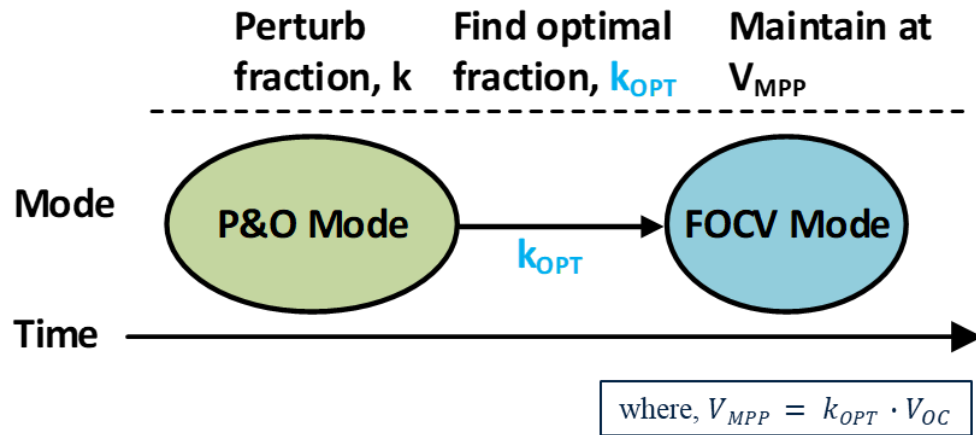
Figure 3.5 Algorithm of the proposed MPPT method
