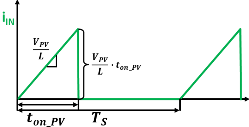
Figure A-2 Input current waveform for PV as input
