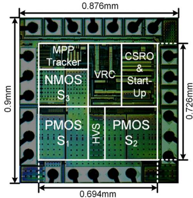
Figure 2.10 Die photo of the second previous work [18]
