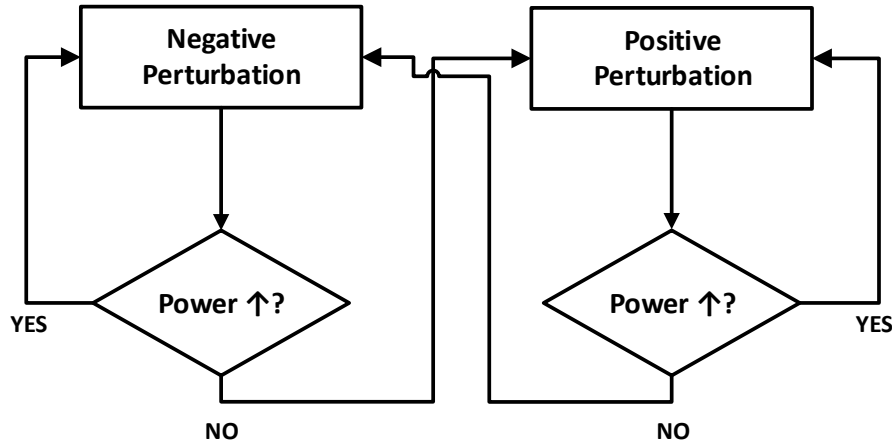
Figure 2.7 P&O algorithm
