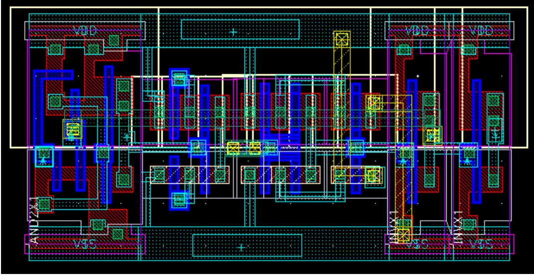
Figure B-3 Ring Oscillator
