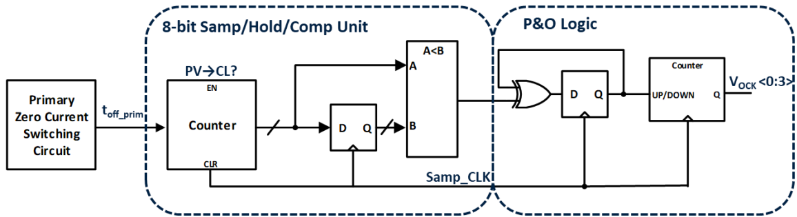
Figure 3.8 Power Measurement Circuit
