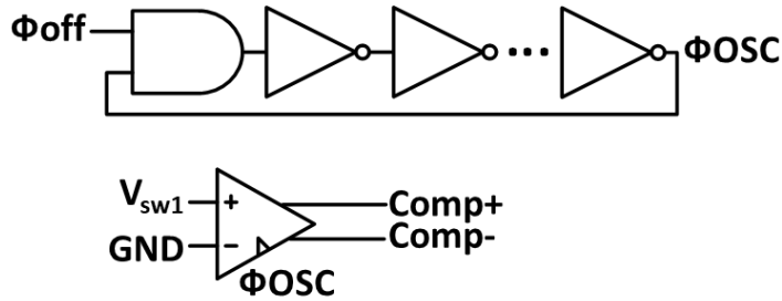
Figure 3.4 Zero Current Detection (ZCD) Circuit
