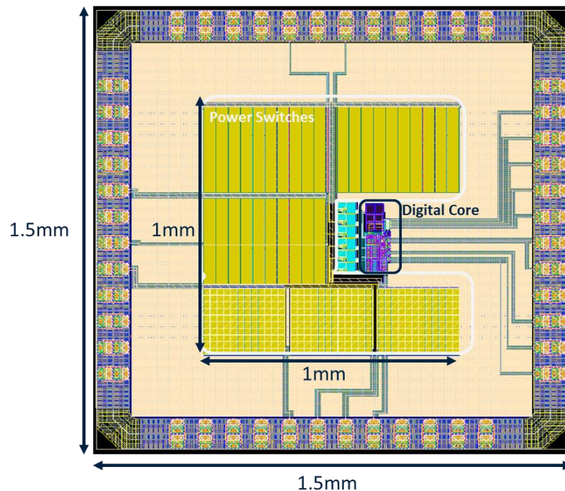
Figure 4.1 Die photo of the proposed circuit and system
