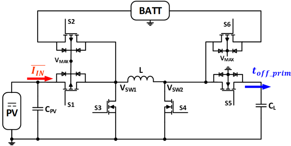
Figure A-1 Power stage Diagram
