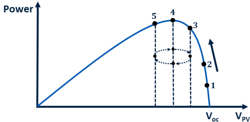
Figure 3.10 Perturb process on the power curve
