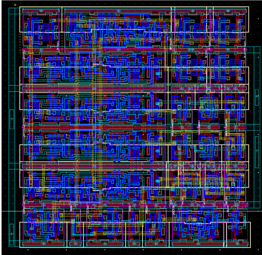
Figure B-5 P&O Logic Block
