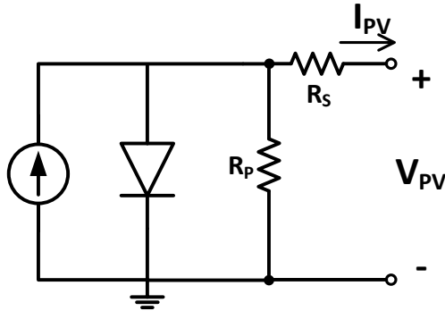
Figure 2.5 One-diode model
