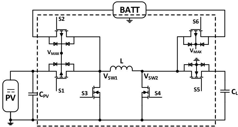
Figure 3.1 Dual-input dual-output buck-boost converter (DIDOB)
