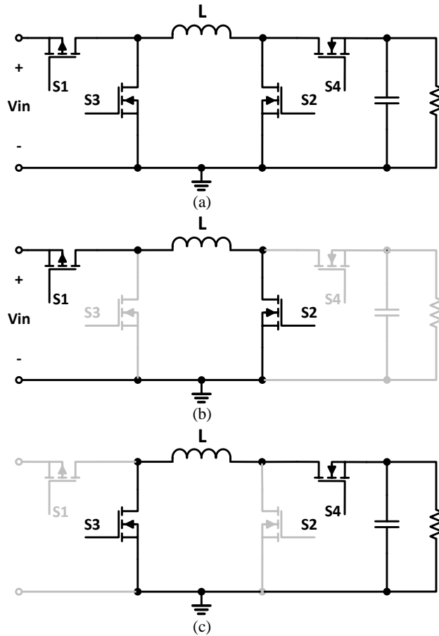
Figure 2.8 (a) Conventional non-inverting Buck-boost converter (b) Charging period (c) Discharging period
