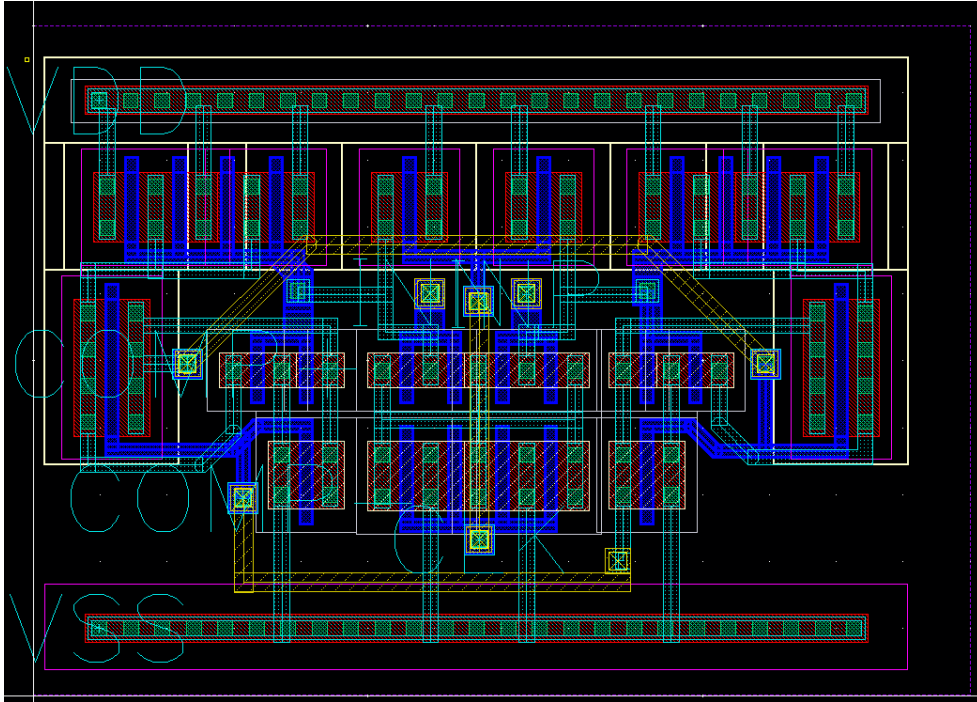
Figure B-9 Clocked Comparator
