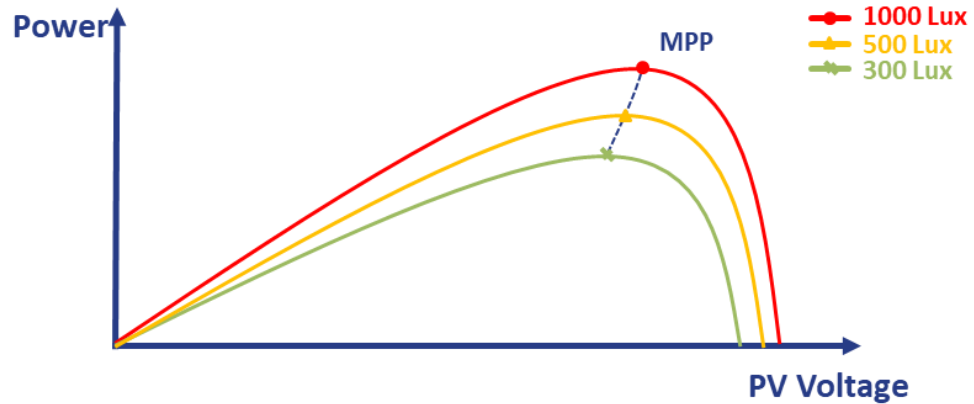
Figure 2.3 The influence of illumination level on the same PV panel I-V characteristics
