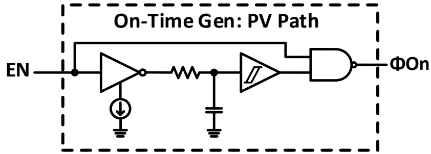
Figure 4.5 Constant On-time Generation Block
