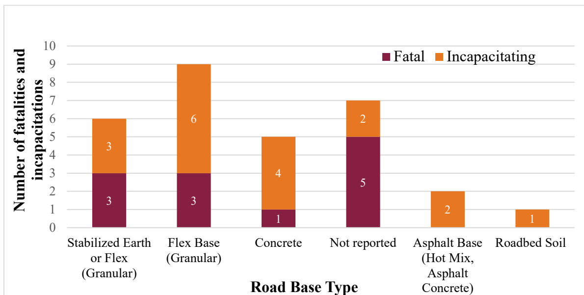
Figure 4. Chart. All KA on flyovers/connectors for various road base materials.
