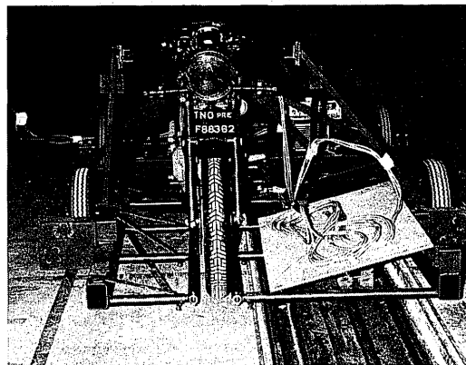
Figure 27. Motorcycle trolley (Nieboer et al., 1993).
