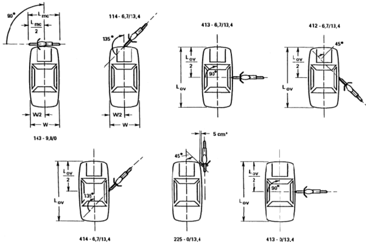
Figure 34. ISO 13232-2 requires seven impact configurations between the MC and OV (ISO 13232, 1996).
