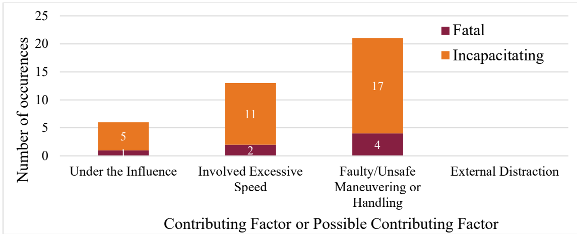
Figure 24. Chart. Distribution of secondary contributing factors and possible contributing factors for KA on curves where the primary contributing factor was “Other (explain in narrative), not reported.”
