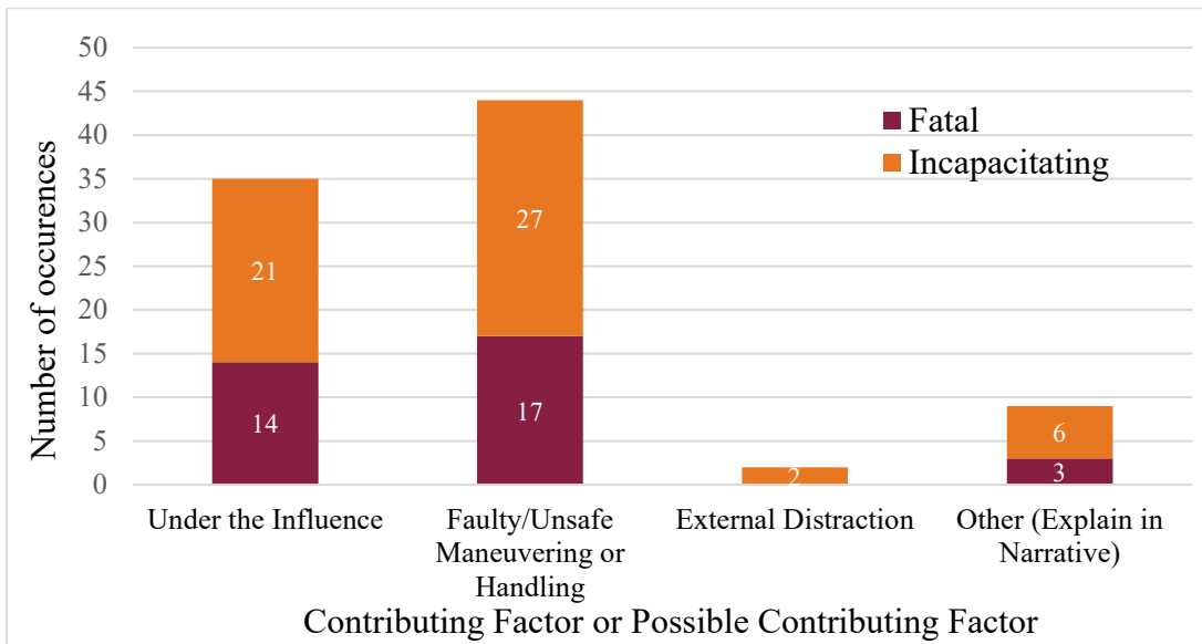
Figure 23. Chart. Distribution of secondary contributing factors and possible contributing factors for KA on curves where the primary contributing factor was “Involved excessive speed.”
