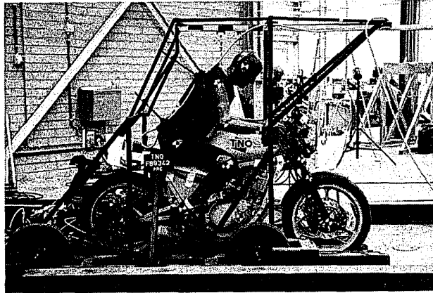
Figure 28. Motorcycle trolley including dummy support frame (Nieboer et al., 1993).
