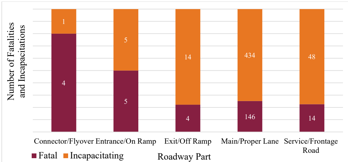
Figure 10. Chart. All KA on curves for various roadway functional classifications.
