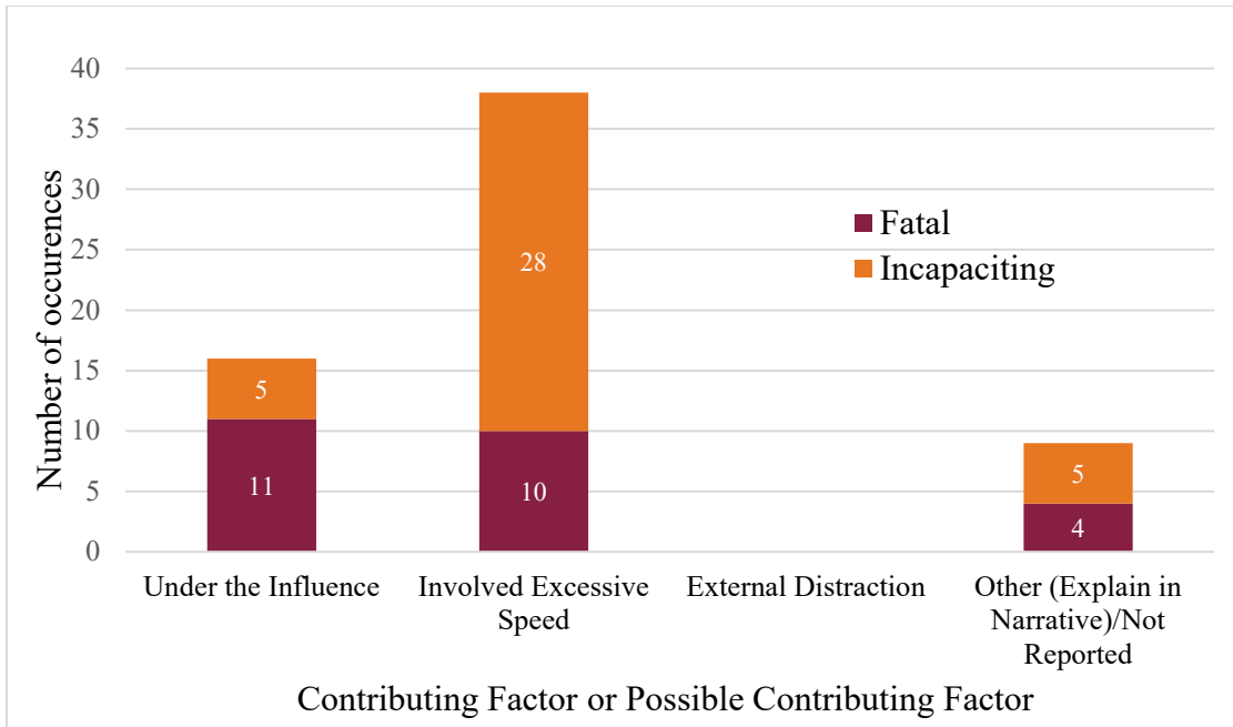
Figure 22. Chart. Distribution of secondary contributing factors and possible contributing factors for KA on curves where the primary contributing factor was “Faulty/unsafe maneuvering.”
