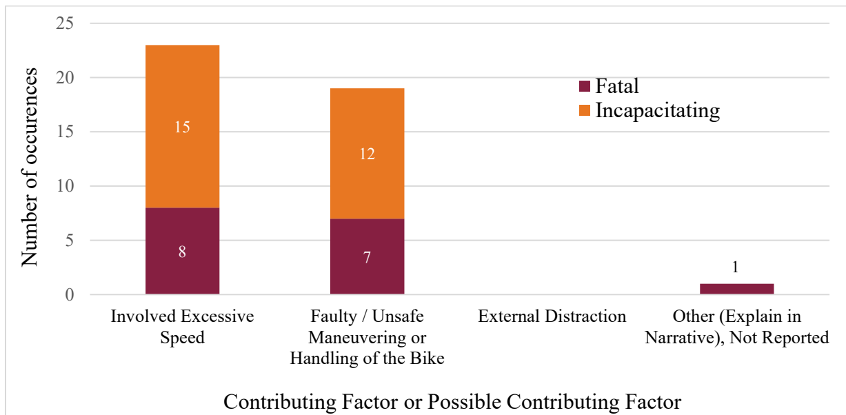
Figure 21. Chart. Distribution of secondary contributing factors and possible contributing factors for KA on curves where the primary contributing factor was “Under the influence.”
