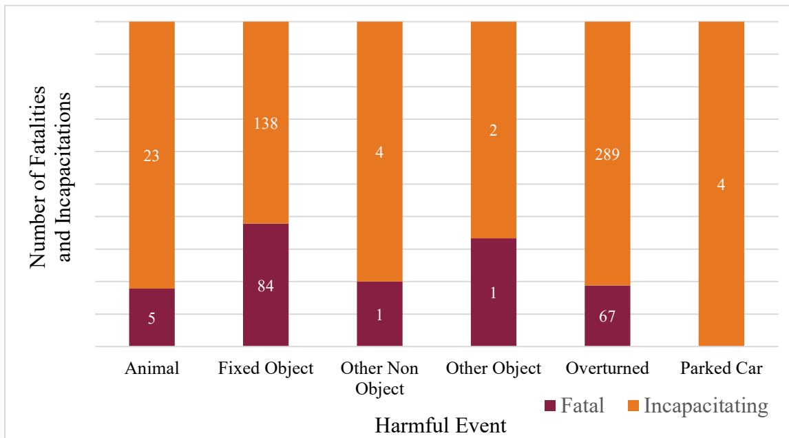
Figure 16. Chart. All KA on curves for harmful events.
