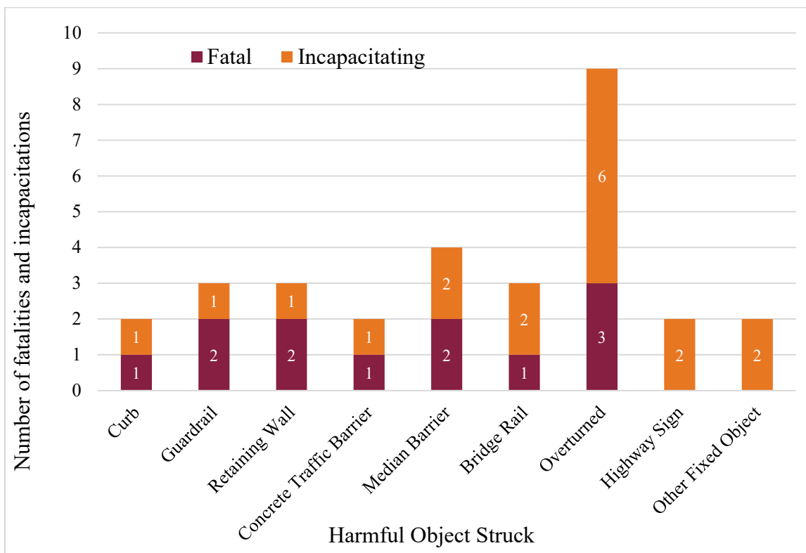
Figure 6. Chart. Distribution of all harmful objects struck resulting in KA on flyovers/connectors.
