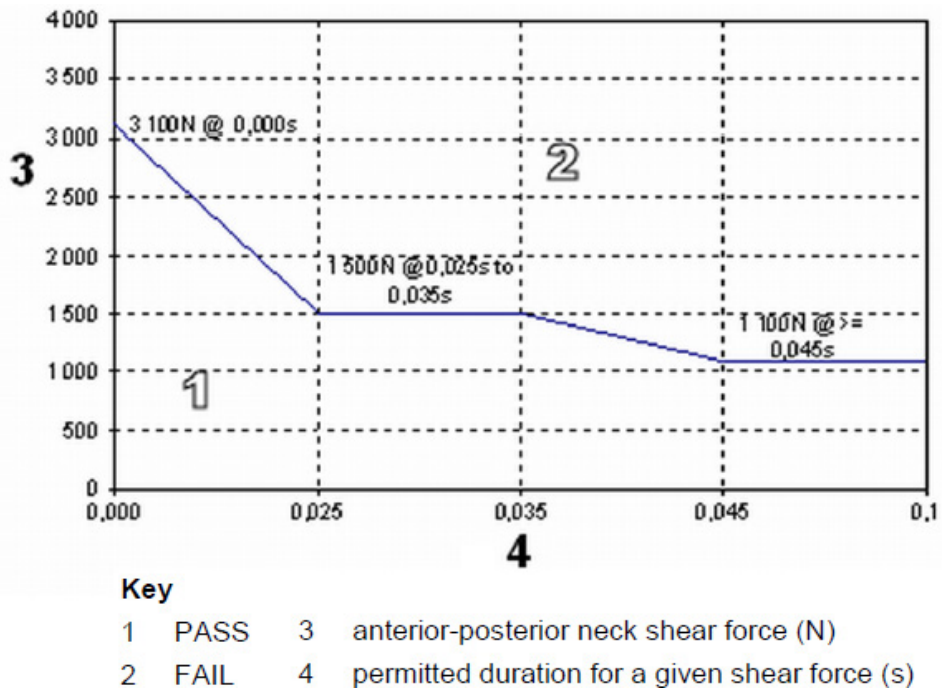
Figure 33. EN 1317-8 Technical Specification Force and Moment Criteria
