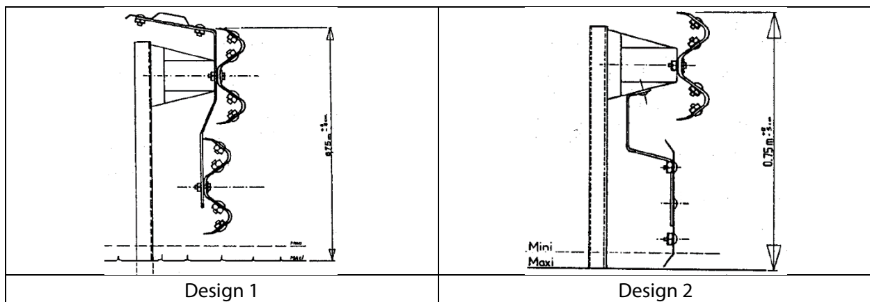
Figure 26. Metal beam standard guardrail designs – INRETS (Quincy et al., 1988).
