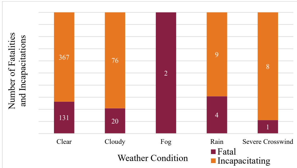
Figure 12. Chart. All KA on curves for various weather conditions.
