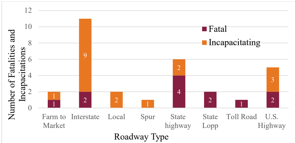
Figure 1. Chart. All KA on flyovers/connectors for various roadway types.
