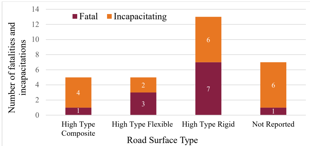
Figure 5. Chart. All KA on flyovers/connectors for various road surfaces.
