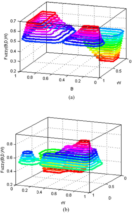
FIGURE 4. A graphical illustration of the fuzzy observations with variations in fuzzy function with respect to B' , W , D . The plots help to understand the impact of rules on the observation of identifying the verifiability for given behavior rules. In both diagrams, the interest is given to a V = \text{Fuzzy}(B, D, W) value higher than the medium value defined by the expert or the user. (a) Fuzzy ( B, D, W ) vs. W and B . (b) Fuzzy ( B, D, W ) vs. W and D .
