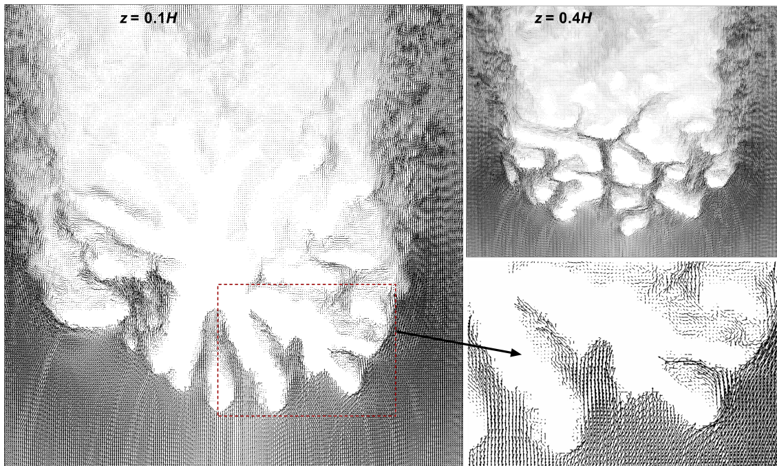
Figure 5. Top view of the instantaneous velocity vector fields at two different heights ( z = 0.1H and 0.4H , where H is the height of the colony) inside the P. meandrina colony. These vector fields show the detailed interaction of the oncoming flow with the individual branches of the colony. The lower right figure shows a zoomed-in view of the velocity vectors at the frontal section of the colony at z = 0.1H . The difference in vector fields at the front and rear halves of the densely branched coral, P. menadrina is clearly observable from the figure.
