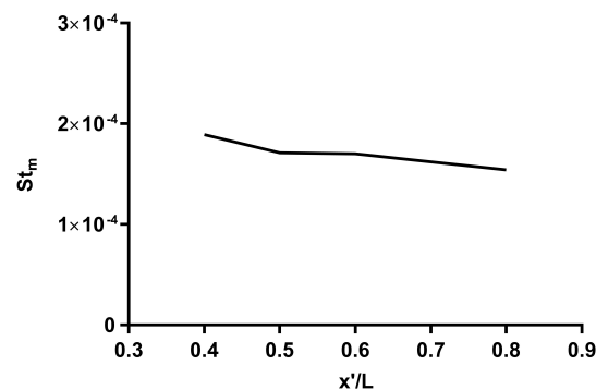
Figure 8. The Stanton number calculated in the interior of the P. meandrina colony based on the mean flow magnitude and advection time scale at Reynolds number 15,000. Here, the advection time scale was calculated based on the mean vortex diameter at different sections of P. meandrina perpendicular to the flow direction, and the mean velocity value in those sections.
