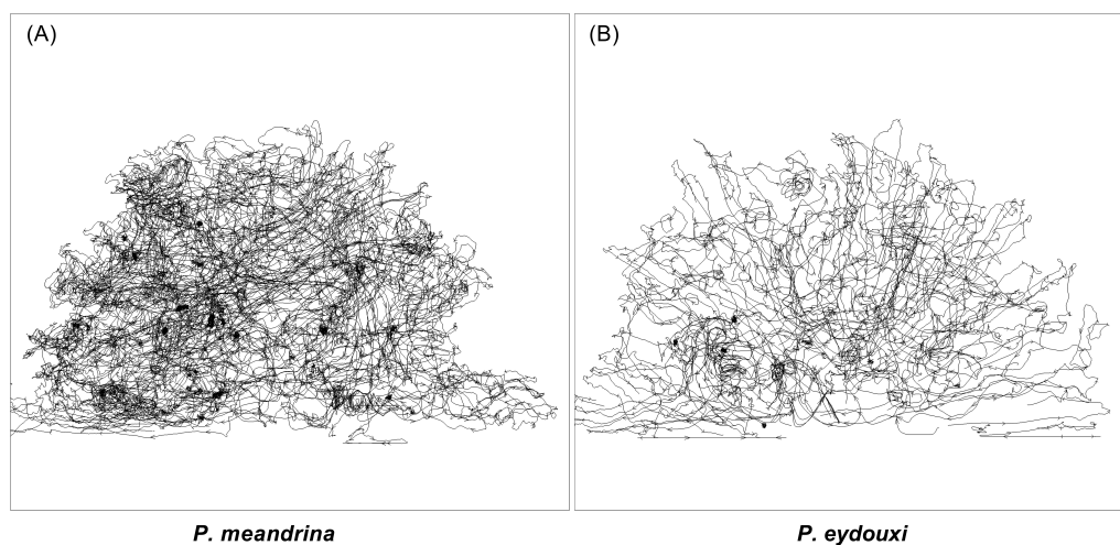
Figure 7. Front-view streamline sections plotted at x' = 0.5 L for both Pocillopora colonies. The formation of vortices can clearly be seen in the inter-branch velocity field of P. meandrina in (A), whereas relatively few vortices are formed around the branches of P. eydouxi , as seen in (B).
