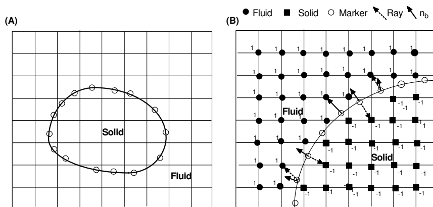
Figure 1. (A) An arbitrary object immersed in Cartesian coordinates. (B) A ray tracing algorithm is utilized in the immersed boundary algorithm [45,46] to identify solid and fluid grid points in the computational domain.
