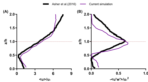
Figure 4. Comparison of (A) the normalized streamwise velocity and (B) Reynolds stress over a single P. meandrina colony from the current simulation with the experimental results over 81 P. meandrina colonies at Re = 23,513 by Asher et al. [20]. The dotted line represents the top of the colony. The experimental data were obtained using GRABIT in MATLAB [52] and reproduced with permission from Asher et al. Vertical variations of coral reef drag forces. Journal of Geophysical Research: Oceans 2016 , 121 , 3549–3563. For both data sets, the mean velocity and Reynolds stress were normalized by the friction velocity.
