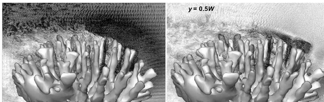
Figure 10. Side view of instantaneous mean (left) and fluctuating (right) velocity vector components above P. eydouxi at y = 0.5W , where W is the width of the colony. Here, the flow is moving from right to left. The instantaneous mean vector field (left) shows a higher concentration of velocity vectors above the colony as most of the flow is diverted to the top and sides of the colony. The fluctuating vector field was obtained by subtracting mean velocity from the instantaneous velocity field. These fluctuating velocity components also appear denser at the top surface of colony and contribute, to the Reynolds stress which controls mass transport to and from the top surface of the colony.
