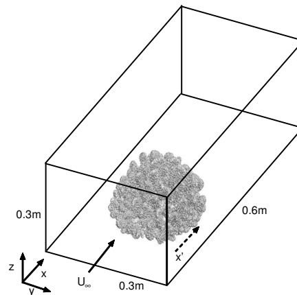
Figure 2. Schematic of flow domain used in the simulation (not to scale). x = 0 indicates the beginning of the flow domain, while x' = 0 represents the beginning (front edge) of the coral in the flow domain.
