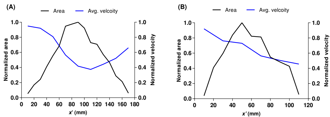
Figure 9. Mean velocity profile and internal cross-sectional area ( y - z plane) along the length of (A) the densely branched P. meandrina colony and (B) the loosely branched P. eydouxi colony. Here, the area and velocity are normalized by the maximum cross-sectional area and oncoming velocity magnitude, respectively.
