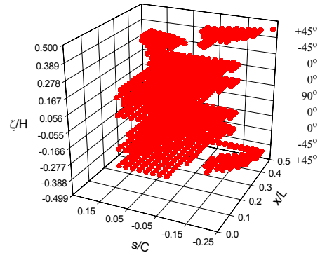
Figure 3.8 Effects of shear modulus degradation on the matrix cracking scenario for the axially-stiff [\pm 45/0_2/90_{1/2}]_s elliptical cylinder, maximum stress criterion, \beta=0.2
