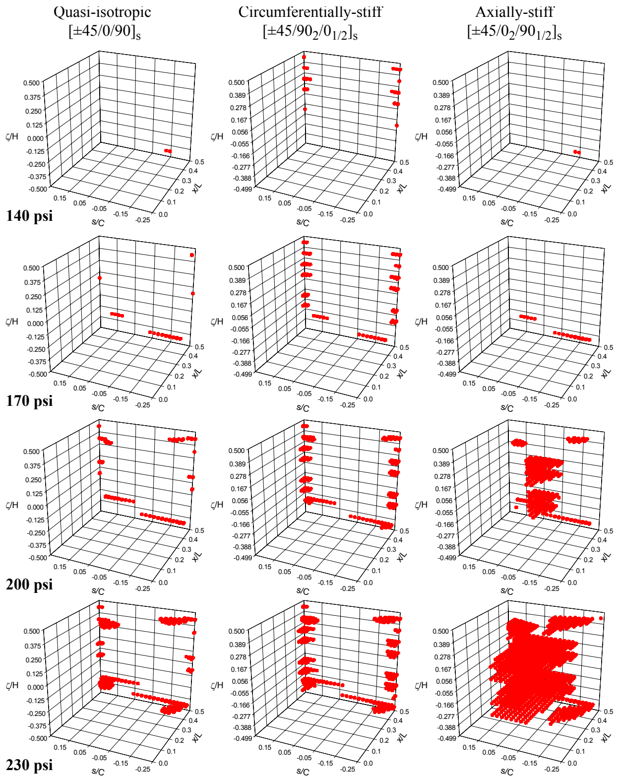
Figure 3.5 Matrix cracking scenarios for elliptical cylinders with different material orthotropy, maximum stress criterion, baseline degradation scheme, \beta=0.2
