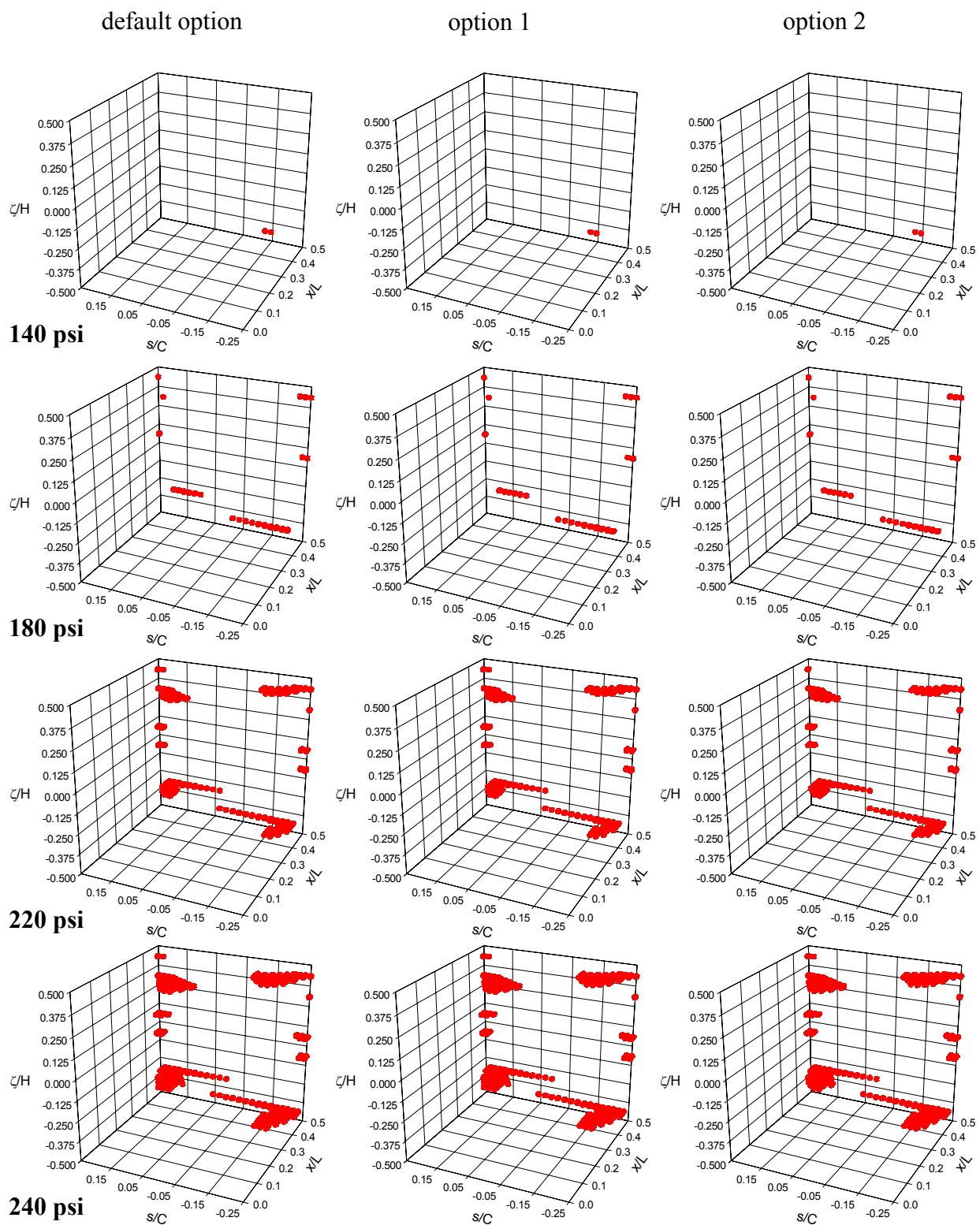
Figure 3.15 Matrix cracking scenarios for the quasi-isotropic [\pm 45/0/90]_3 elliptical cylinder, maximum stress criterion, baseline degradation scheme, \beta=0.2 , different computational algorithms
