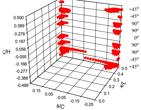
Figure 3.7 Effects of shear modulus degradation on the matrix cracking scenario for the circumferentially-stiff [\pm 45/90_2/0_{1/2}]_s elliptical cylinder, maximum stress criterion, \beta=0.2
