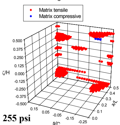
Figure 5.1 Modes of failure involved in leakage for the quasi-isotropic [\pm 45/0/90]_s elliptical cylinder, baseline degradation scheme, maximum stress criterion, \beta=0.2
