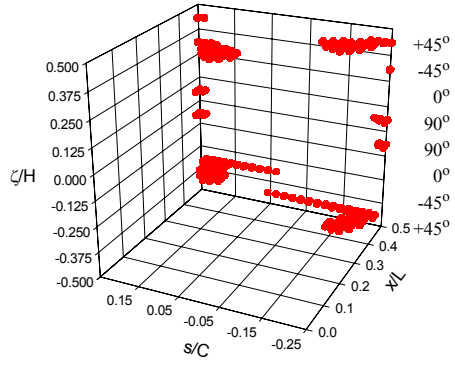
Figure 3.6 Effects of shear modulus degradation on the matrix cracking scenario for the quasi-isotropic [\pm 45/0/90]_s elliptical cylinder, maximum stress criterion, \beta=0.2
