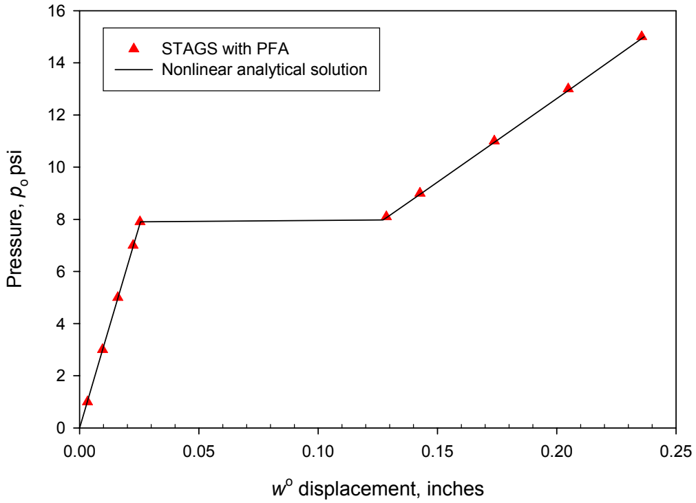
Figure 2.5 Internal radial load vs. outward displacement at any axial location
