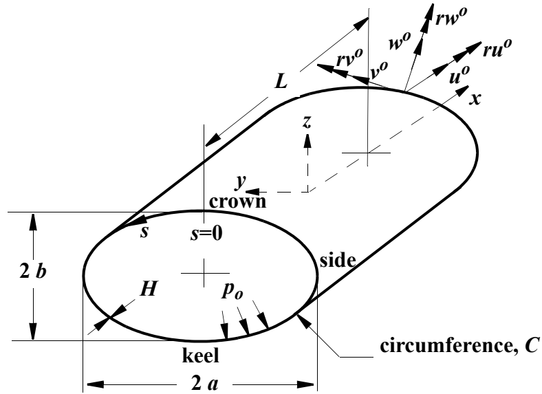
Figure 3.1 Geometry and nomenclature of elliptical cylinder
