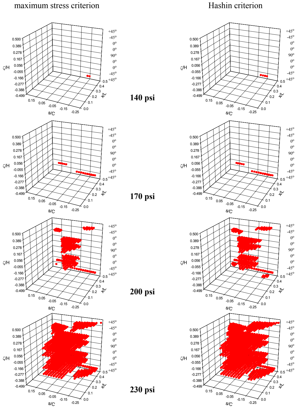
Figure 4.3 Matrix cracking scenarios for maximum stress and Hashin failure criteria for the axially-stiff [\pm 45/0_2/90_{1/2}]_s elliptical cylinder, baseline degradation scheme, \beta=0.2
