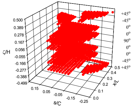
Figure 3.8 Effects of shear modulus degradation on the matrix cracking scenario for the axially-stiff [\pm 45/0_2/90_{1/2}]_s elliptical cylinder, maximum stress criterion, \beta=0.2
