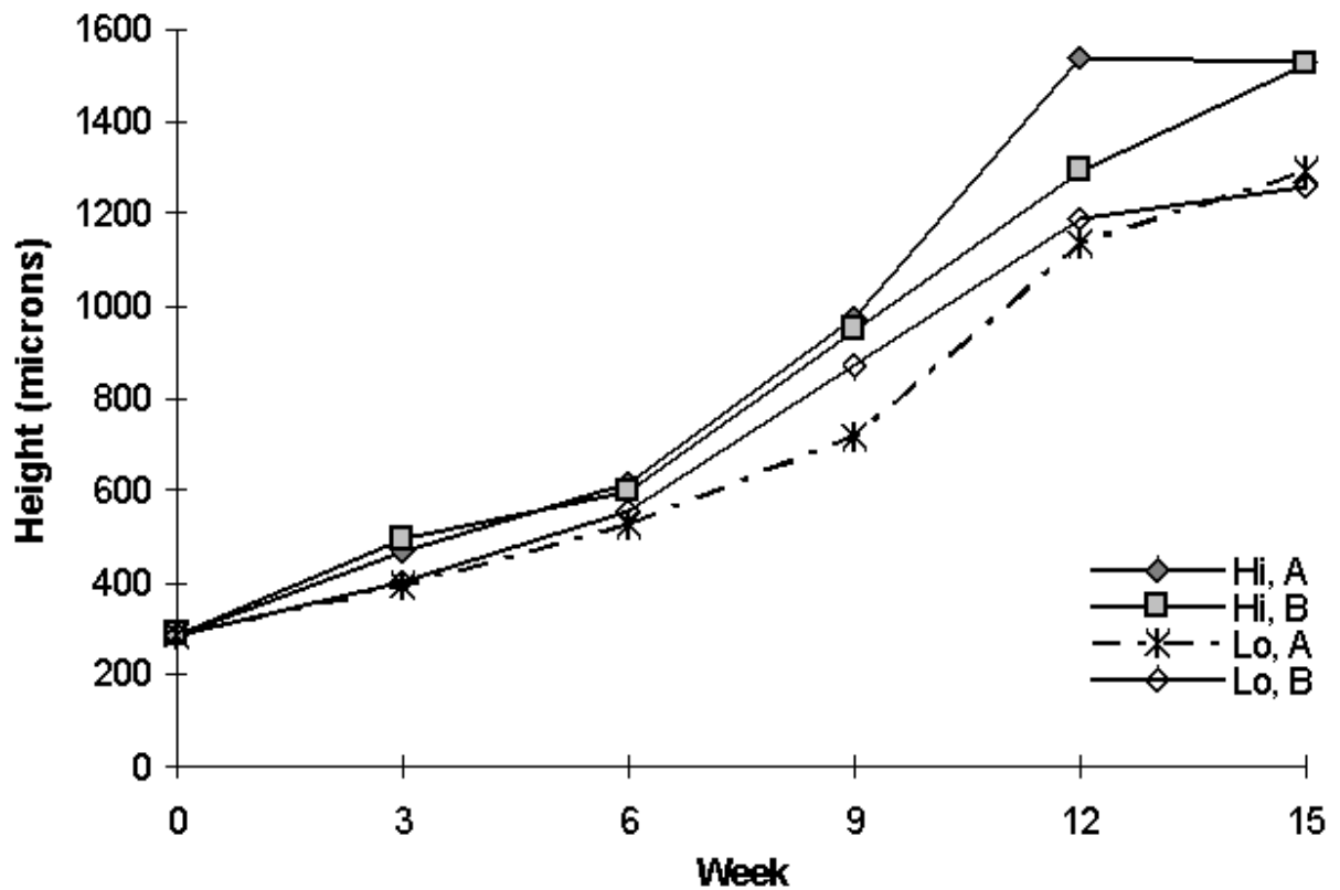
Figure 8. Growth in shell height of juveniles in the water hardness and substrate organic content culture treatments. (“Hi”= high water hardness, “Lo”= low water hardness, “A”= high soil organic content, “B”= low soil organic content).
