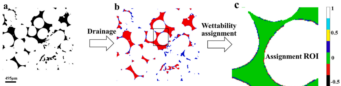
Fig. 1. The workflow for the assignment of contact angles; (a) is the binary image (black = pore, white = grain); (b) is the image after drainage (red = oil, blue = water, white = grain); (c) is the Region-Of-Interest (ROI) image after wettability assignment.
