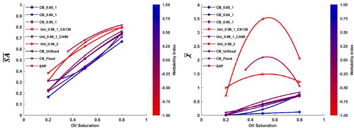
Fig. 4. (a) Surface area normalization (oil-grain surface area/total grain surface area) (b) Euler normalization (Euler of NWP/Euler of pore space) of 8 simulations and experimental data. The reported value at oil saturation of 0.2 is not the residual oil saturation. Overall, the results from ‘Uni_0.99_2’ and ‘Uni_0.99_1’ provided the best morphological match with the experimental data.
