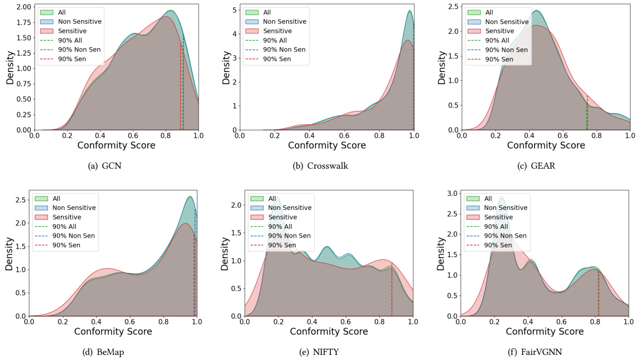
Figure 4: Comparison of Conformity Score Distributions Across Different Methods.
