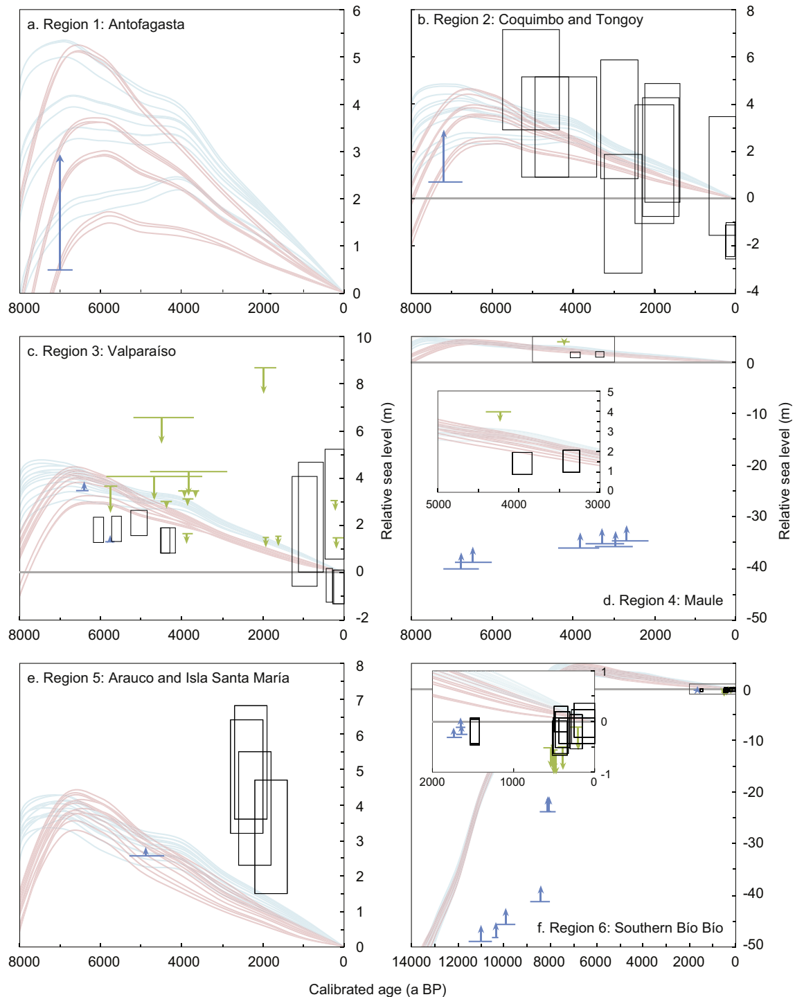
Fig. 7. Regional plots comparing the age – elevation distribution of the sea-level data points with glacial isostatic adjustment model predictions (following Peltier, 2004 ; Peltier et al., 2015 ). Sea-level index points are black rectangles, terrestrial and marine limiting points are green T-shaped symbols and blue L-shaped symbols respectively. ICE_5G predictions are light blue curves, ICE_6G predictions are pink curves; for both ice models we vary the lithospheric thickness between 71 and 120 km and the upper mantle viscosity between 5 \times 10^{19} Pa s and 2 \times 10^{20} Pa s (see section 3.7). Note different x-axis scaling for panel f and variable y-axis scaling between all panels. (For interpretation of the references to colour in this figure legend, the reader is referred to the Web version of this article.)
