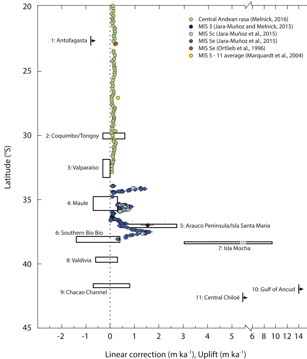
Fig. 8. Comparison of best-fit linear correction rates (black rectangles) required to remove the misfit between sea-level data and a suite of glacial isostatic adjustment models with independently derived estimates of tectonic uplift (coloured circles). Sea-level data and GIA models for the 11 regions are shown in Fig. 7 and the linear corrections are illustrated in Supplementary Information S3 Marquardt et al., 2004.
