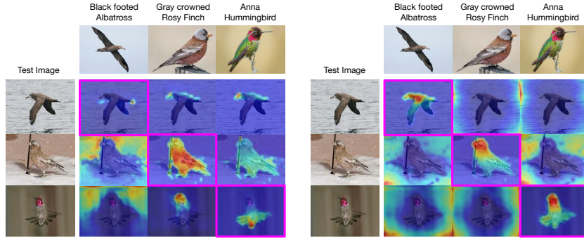
Figure 18: We show the attention maps from two cross-attention heads: Head-1 (left) and Head-4 (right). Row-wise: test images from different classes; column-wise: different class-specific queries. To make correct predictions (diagonal), INTR must find and localize the property of an attribute (e.g., the dotted pattern of the tail from Head-1; the color pattern of the bird’s head from Head-4) at the correct part (e.g., on the tail or head).
