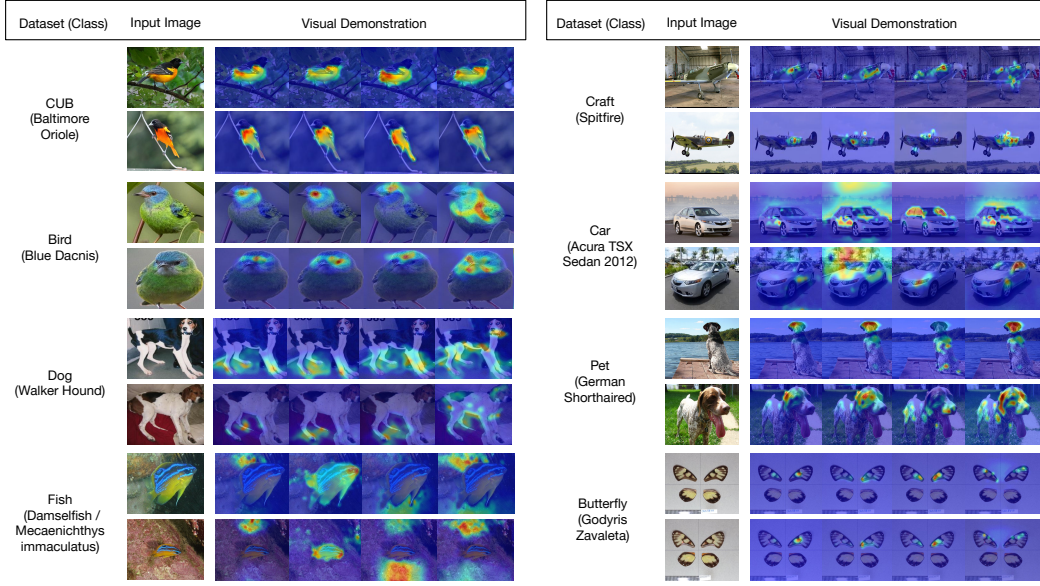
Figure 4: INTR on all eight datasets. We show the top four cross-attention maps per test example triggered by the ground-truth classes (based on the peak un-normalized attention weights in the maps). As the indices of the top maps may not be the same across test examples, the attributes may not be the same in each column.
