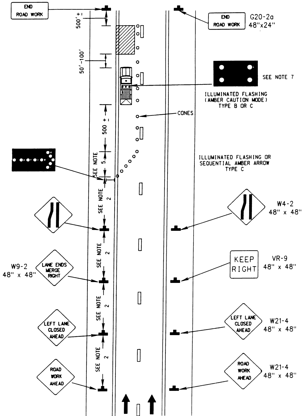
INSIDE LANE CLOSURE ON FOUR-LANE ROADWAY FIGURE TTC-15 0
