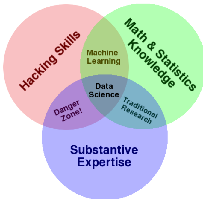
Figure 1.1: Reproduction of Drew Conway’s Data Science Venn Diagram [27].
