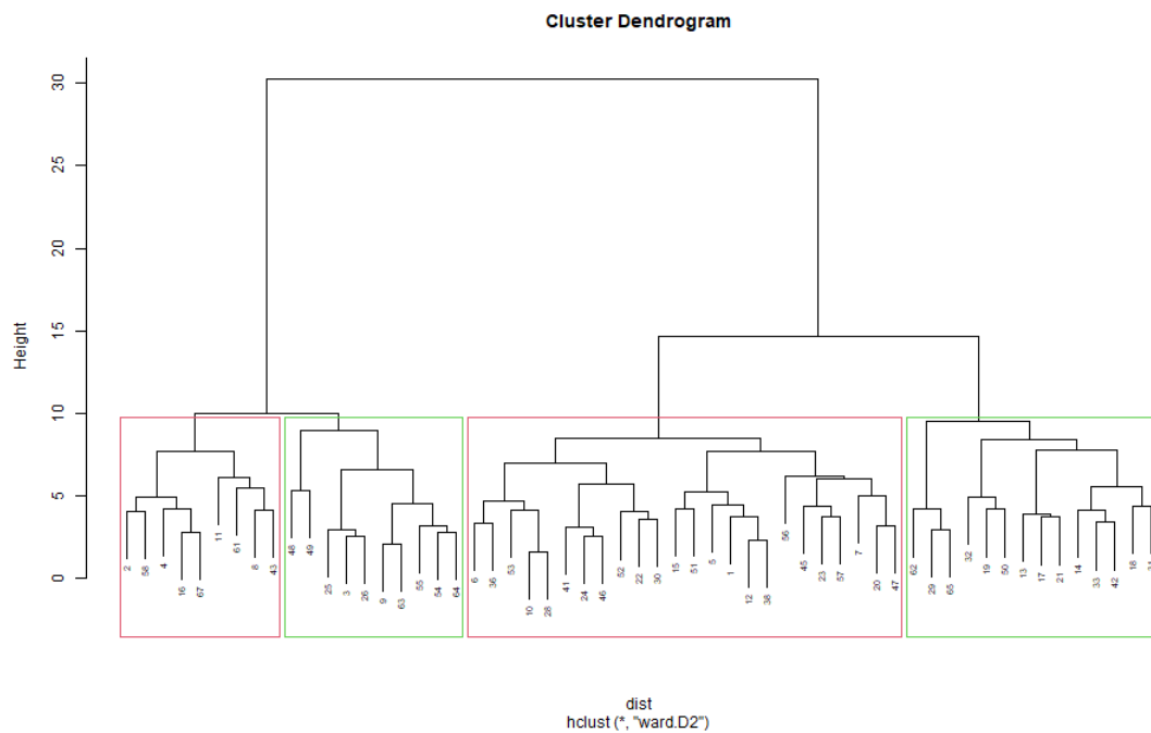
Figure 2.11: Dendrogram showing 4 clusters. Looking at the differences in how the clusters were split from the 3-cluster model (Figure 2.10), the same group that eventually was named Samir Student (Group 2) was split into another cluster. This split was hard to interpret, so the 3-cluster model was used for creating the learner personas.
