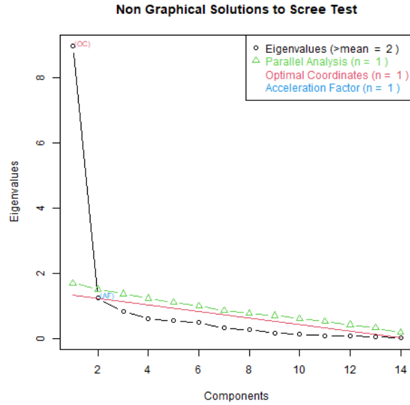
Figure 2.4: Scree plot for factor analysis showing the number of components (x) and the eigenvalues (y). The figure suggests exploring 2 to 4-factor models.
