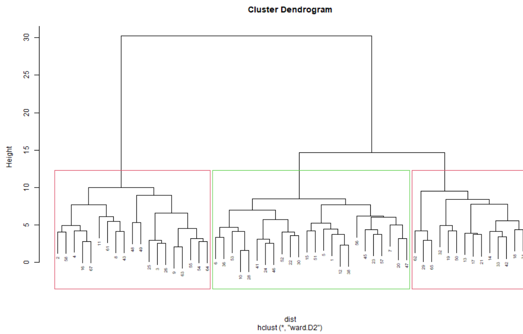
Figure 2.10: Dendrogram of the three (3) learner persona clusters. The clusters were combined with the survey responses to identify the learner personas. From left to right, the clusters are: Samir Student (Group 2), Ash Academic (Group 1), and Clare Clinician (Group 3).
