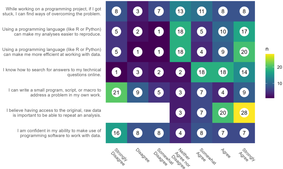
Figure 2.2: Number of responses for each summary Likert scale question. Likert questions were initially created as a summary table to gauge respondents attitudes programming in data analysis. Results show that most respondents believe having raw access to data is important to repeat an analysis, but are less likely able to use a programming language to perform an analysis. There is a bimodal distribution between being indifferent and strongly agreeing about programming languages making analysis easier and more efficient.
