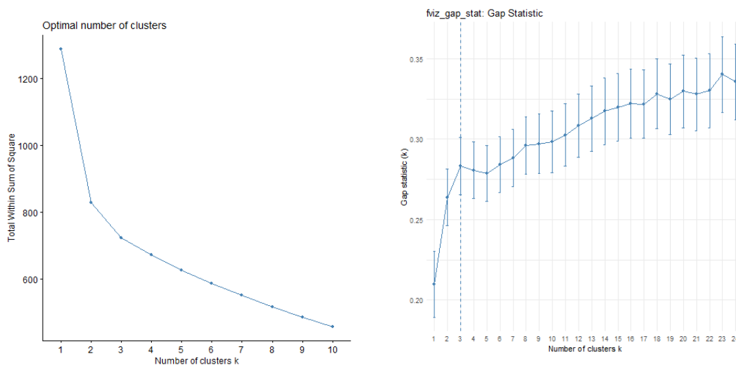
(a) Elbow plot showing the total within-cluster sum of squares (y-axis) for increasing number of clusters, k (x-axis). (b) Gap statistic comparing intra-cluster variation as compared to a distribution with no clustering (y-axis) for different number of clusters, k (x-axis).
