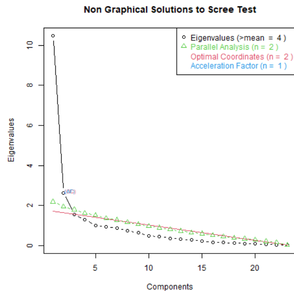
Figure 2.9: i Scree plot for factor analysis showing the number of components (x) and the eigenvalues (y) for all 23 survey items. The figure suggests exploring 2 to 4 factor models.
